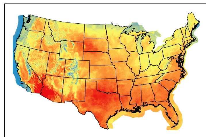
Dry Bulb Temp temp20240803.bil
