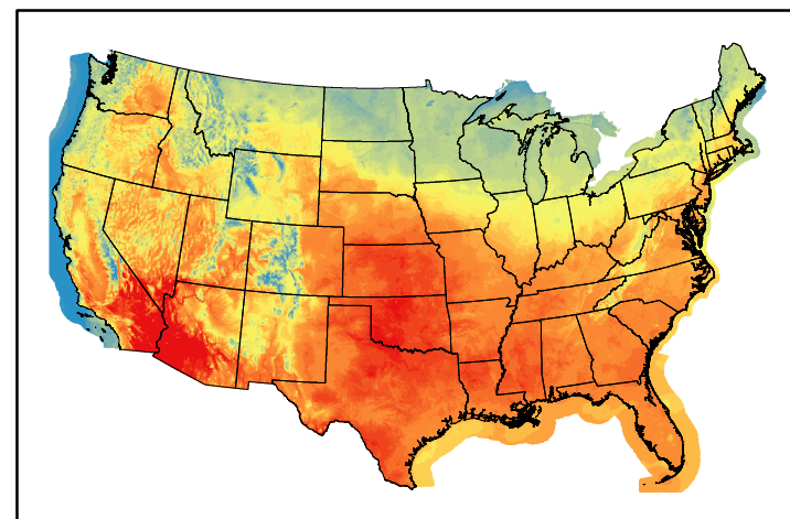
Dry Bulb Temp temp20240805.bil
