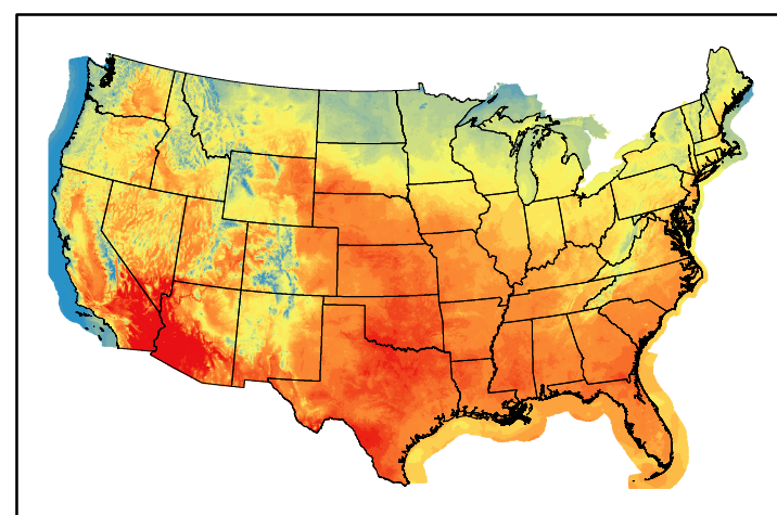
Dry Bulb Temp temp20240804.bil
