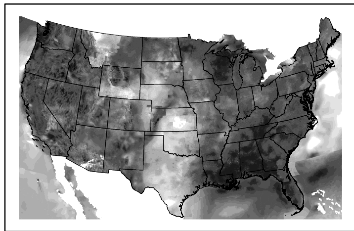
Wind Speed wspd20240731.bil
