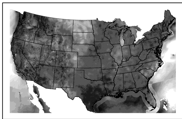
Wind Speed wspd20240803.bil
