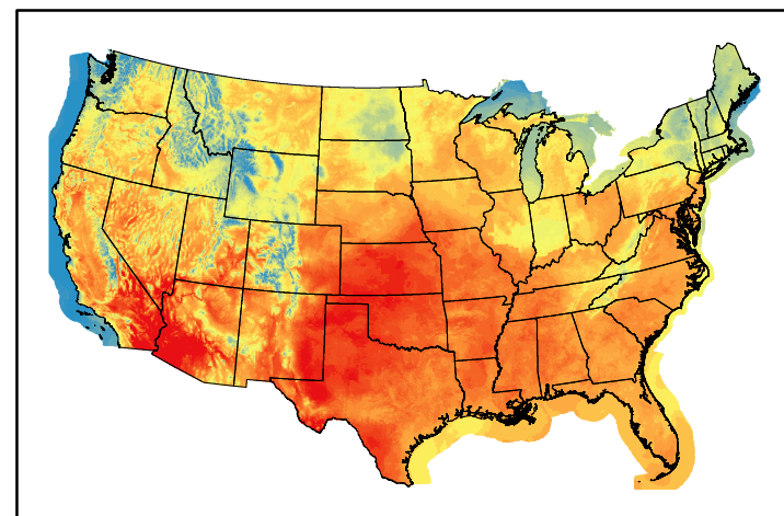
Dry Bulb Temp temp20240731.bil
