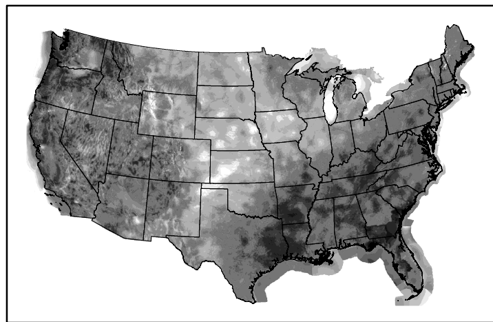
Wind Speed wspd20240806.bil
