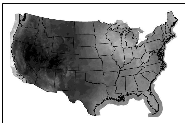
10hr Fuel Moisture mc10240801.bil
