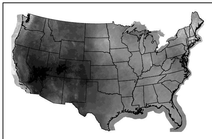
10hr Fuel Moisture mc10240731.bil
