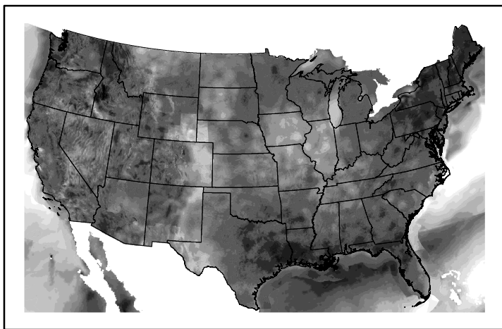
Wind Speed wspd20240802.bil
