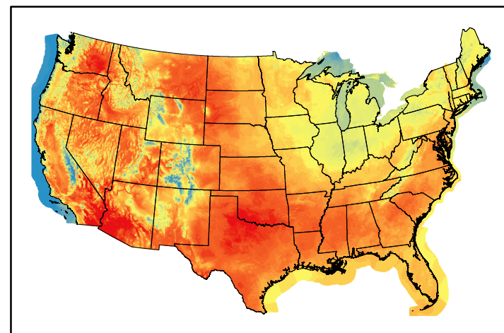
Dry Bulb Temp temp20240802.bil
