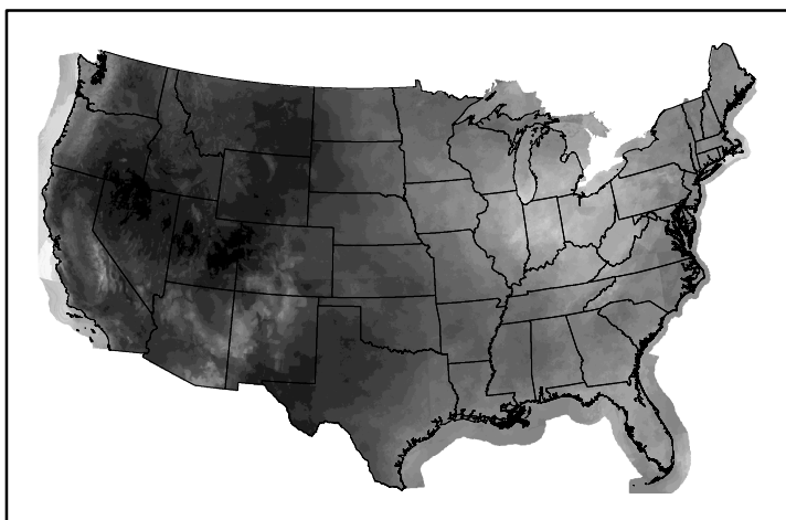
10hr Fuel Moisture mc10240802.bil
