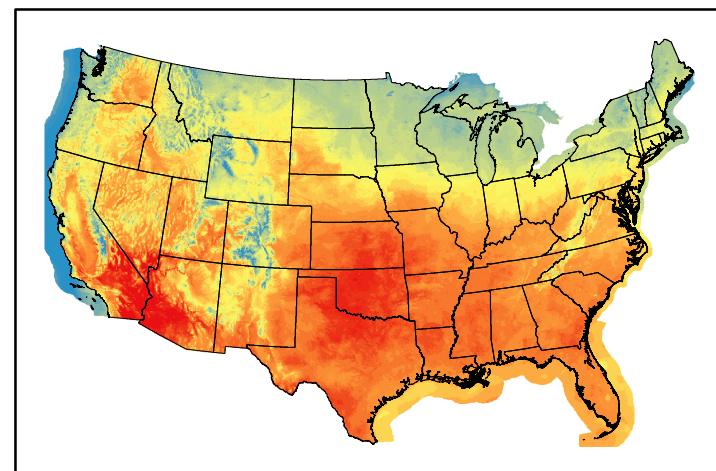
Dry Bulb Temp temp20240806.bil
