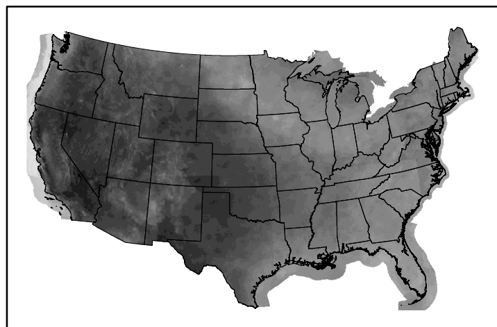
10hr Fuel Moisture mc10240805.bil
