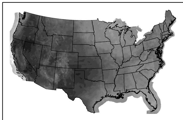
10hr Fuel Moisture mc10240806.bil
