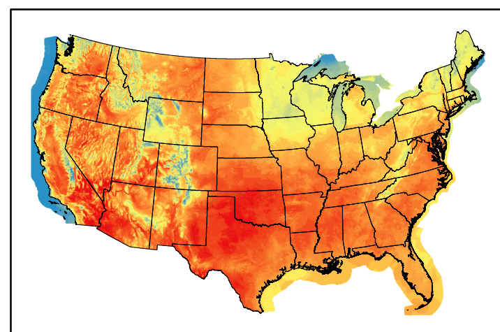
Dry Bulb Temp temp20240801.bil
