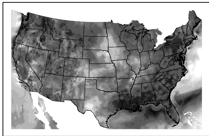
Wind Speed wspd20240801.bil
