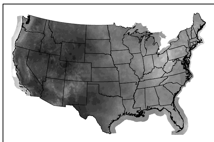
10hr Fuel Moisture mc10240803.bil
