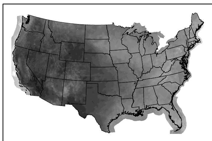
10hr Fuel Moisture mc10240804.bil
