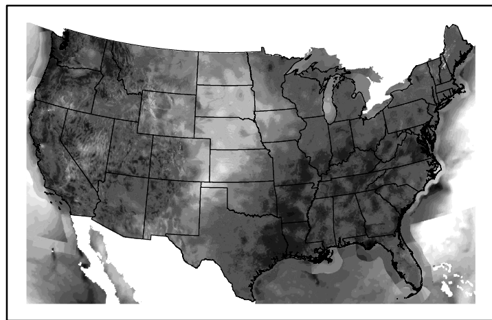
Wind Speed wspd20240805.bil
