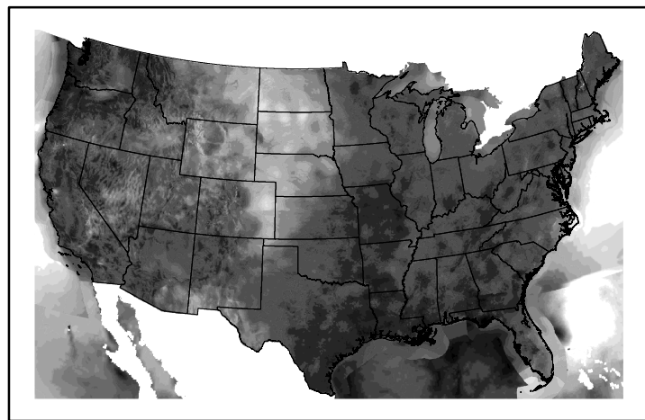
Wind Speed wspd20240804.bil
