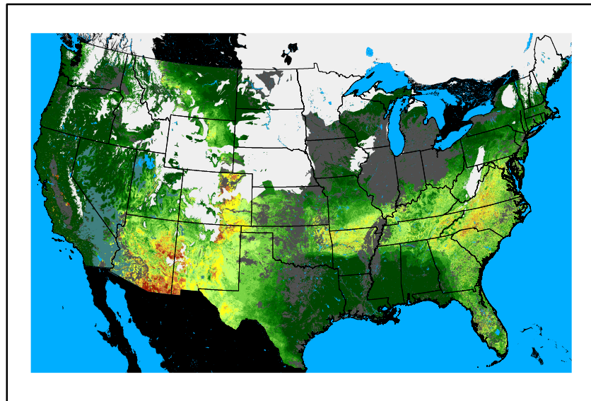
WFPI fp240103.bil
