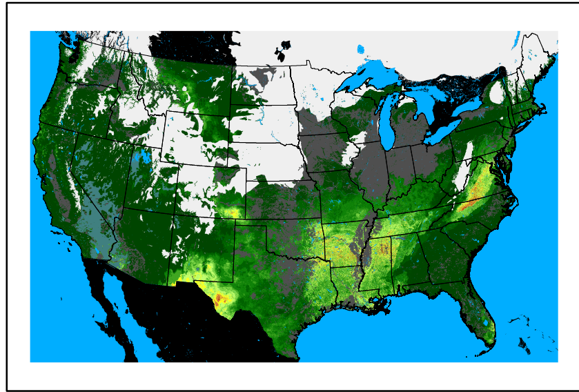
WFPI fp240104.bil
