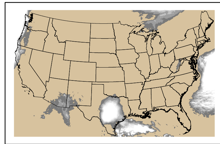
Precipitation p24m_2024010100f048.bil
