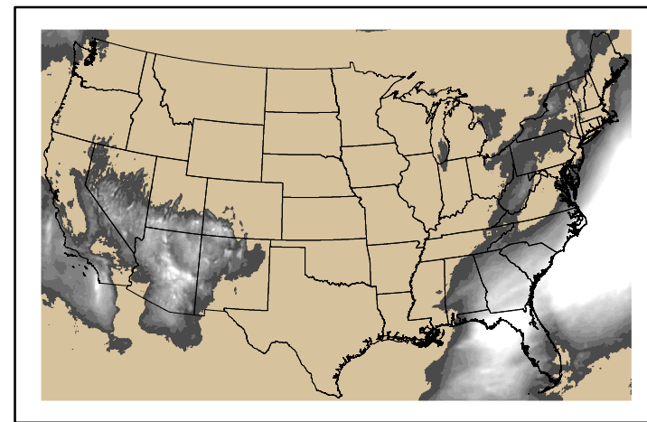
Precipitation p24m_20240100f096.bil
