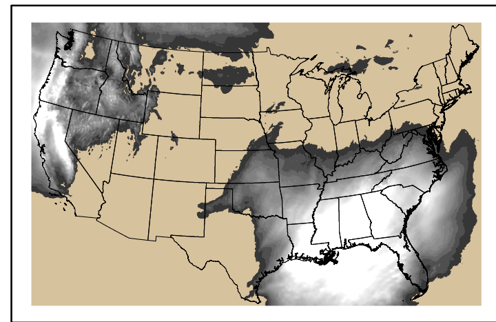
Precipitation p24m_20240100f144.bil
