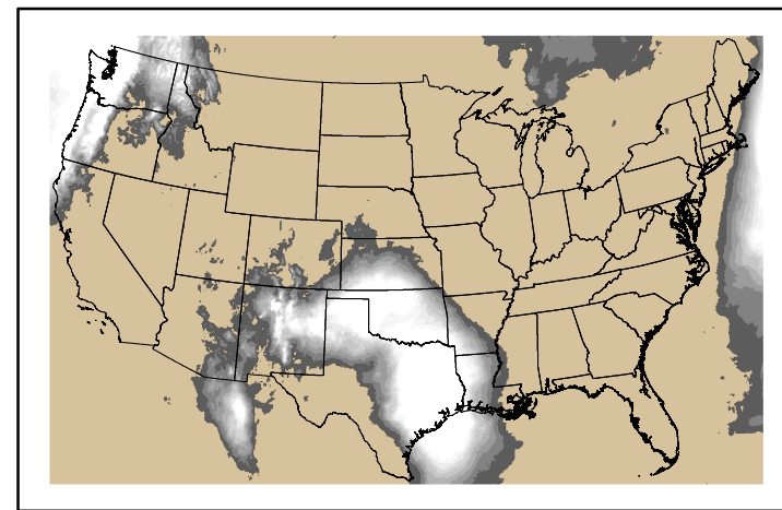
Precipitation p24m_20240100f120.bil
