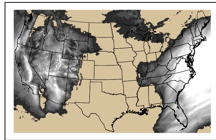
Precipitation p24m_20240100f168.bil
