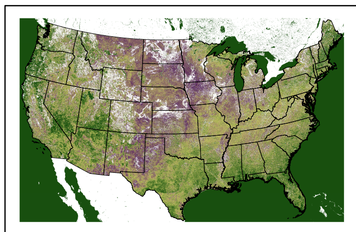
Greenness us23_359365wk_greenness.img
