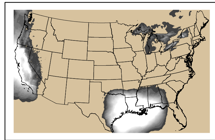
Precipitation p24m_20240100f072.bil
