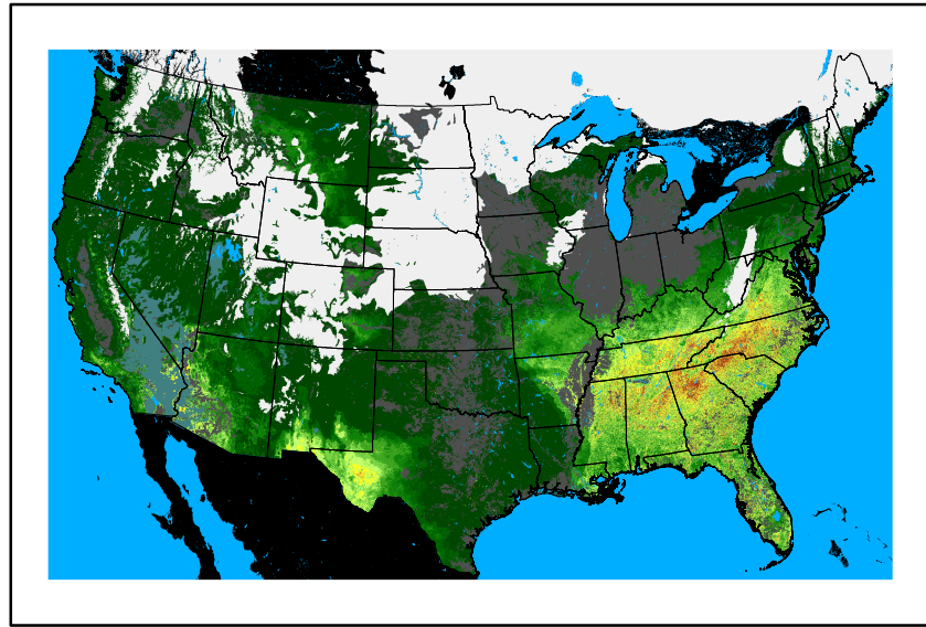
WFPI fp240105.bil
