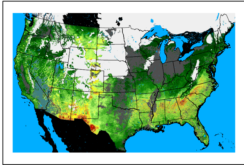
WFPI fp240101.bil
