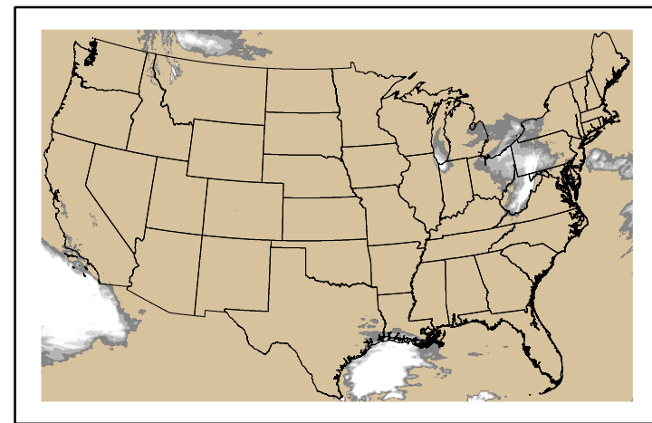
Precipitation p24m_2024010100f024.bil
