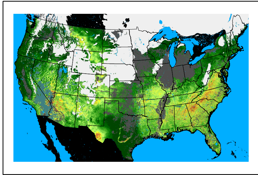
WFPI fp240102.bil
