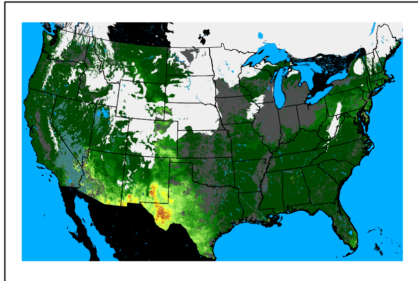
WFPI fp240106.bil
