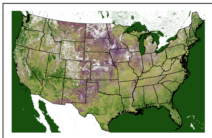
Greenness us23_359365wk_greenness.img
