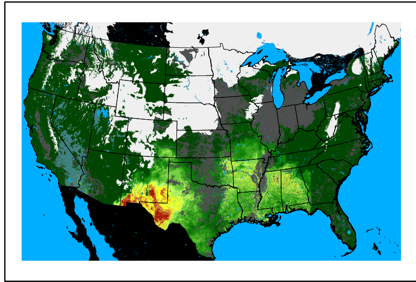
WFPI fp240107.bil
