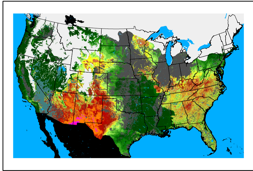
WFPI fp250303.bil
