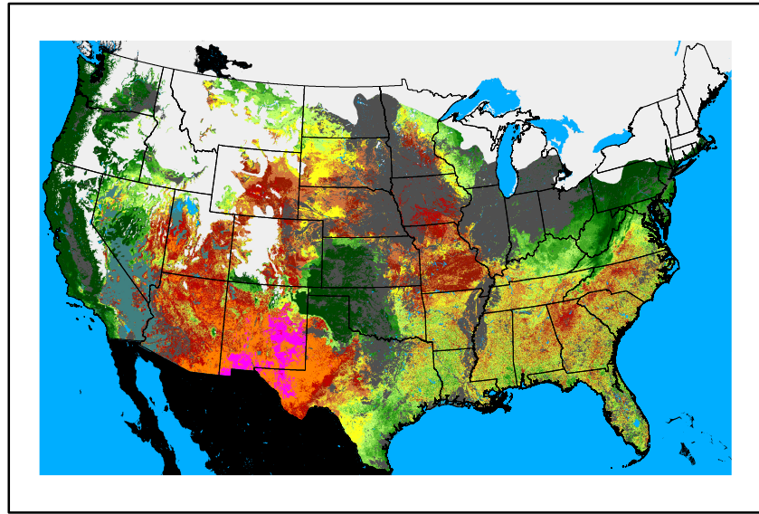
WFPI fp250302.bil
