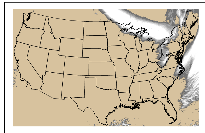
Precipitation p24m_2025022800f024.bil
