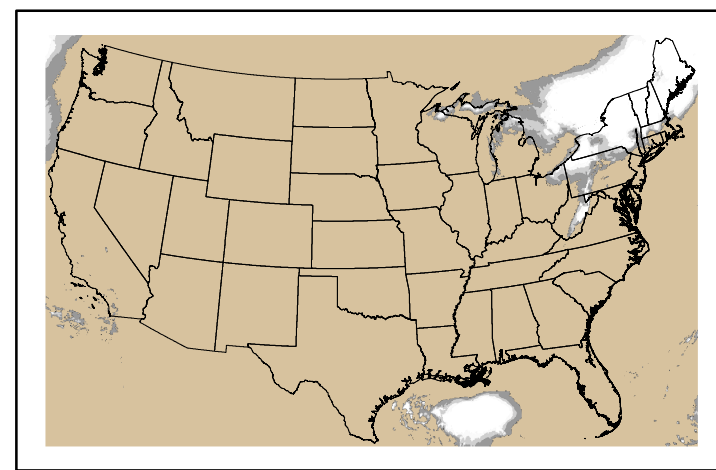
Precipitation p24m_2025022800f048.bil
