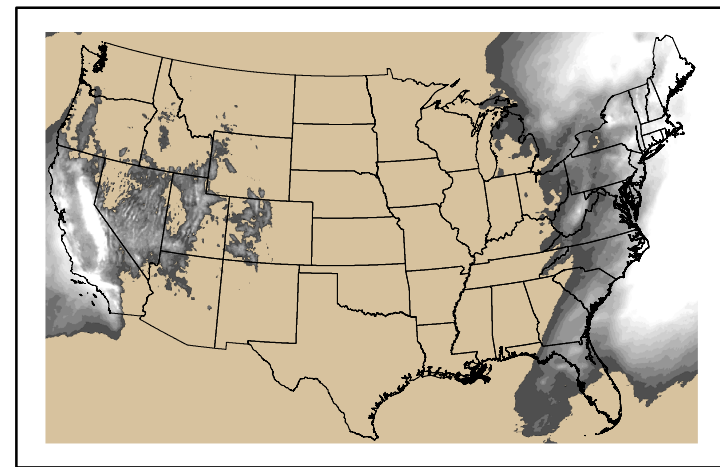
Precipitation p24m_2025022800f168.bil
