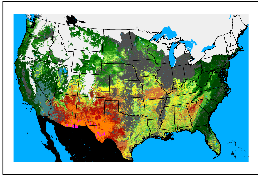
WFPI fp250306.bil
