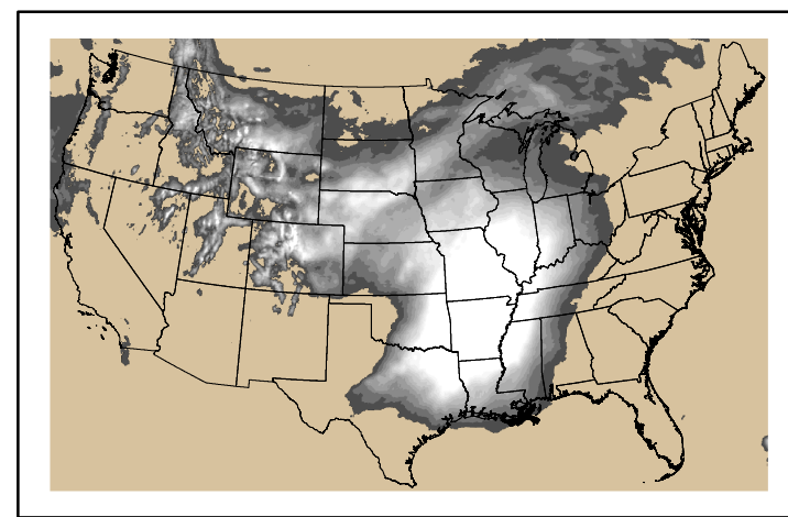
Precipitation p24m_2025022800f120.bil
