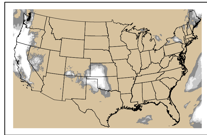
Precipitation p24m_2025022800f072.bil
