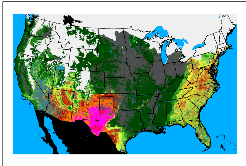
WFPI fp250304.bil
