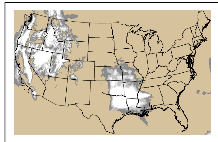
Precipitation p24m_2025022800f096.bil
