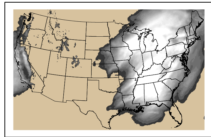
Precipitation p24m_2025022800f144.bil
