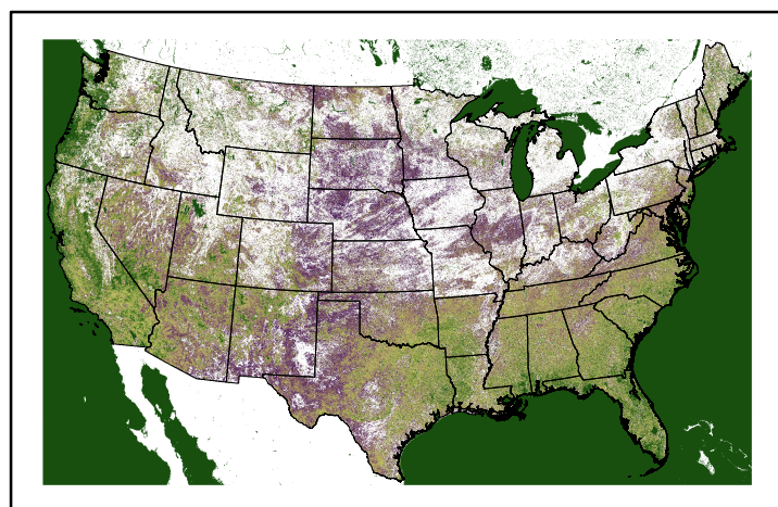
Greenness us25_048054wk_greenness.img
