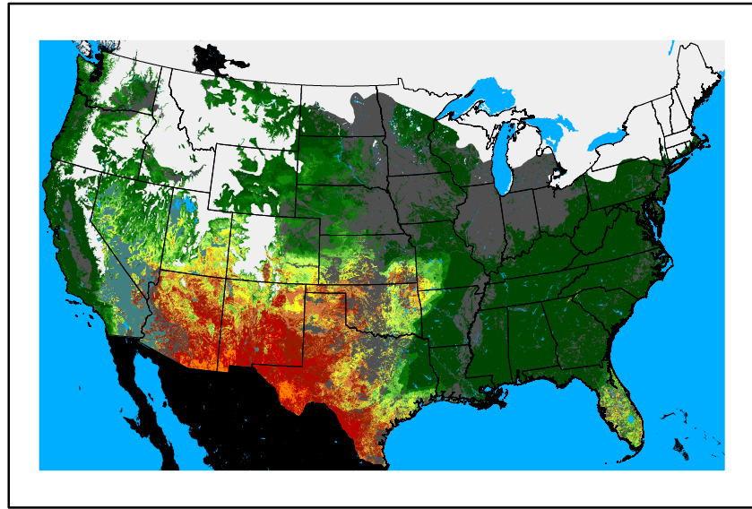
WFPI fp250305.bil
