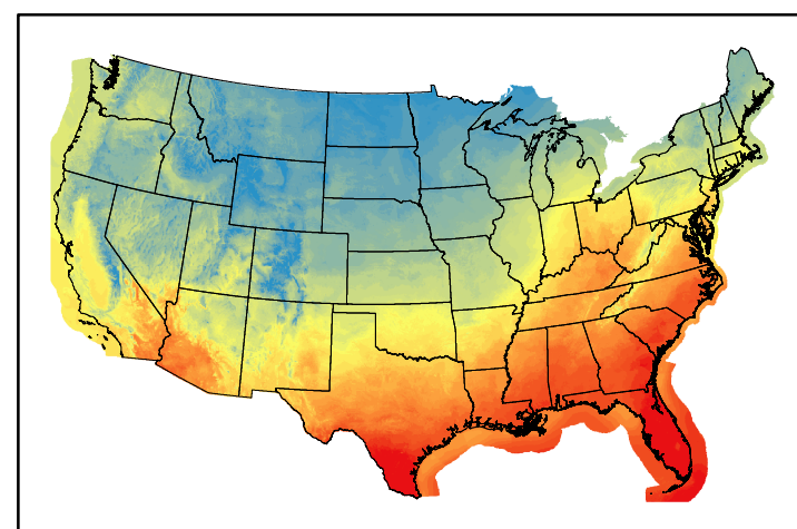
Dry Bulb Temp temp20250305.bil
