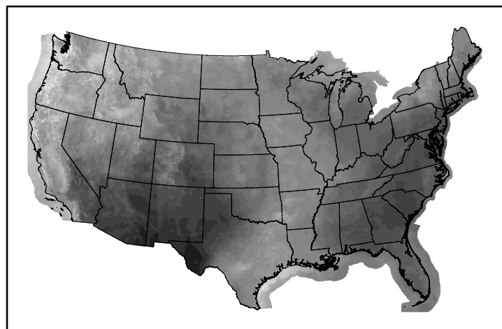
10hr Fuel Moisture mc10250303.bil
