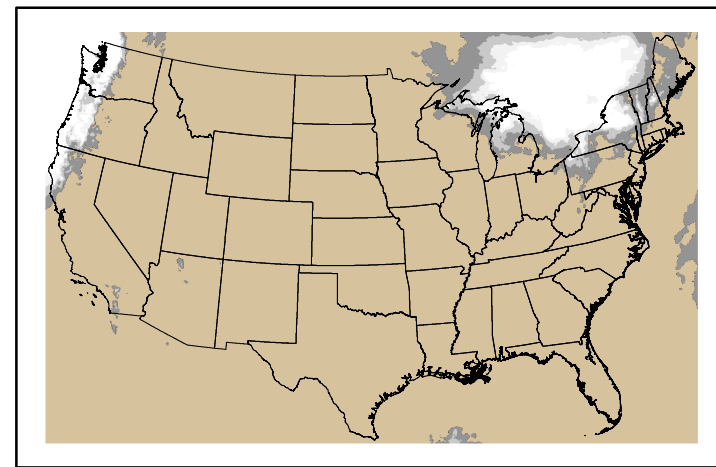
Precipitation p24m_2025022400f144.bil
