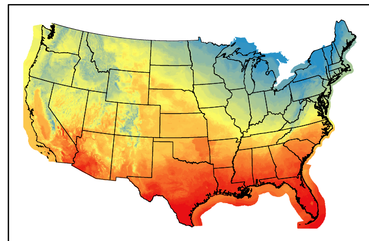
Dry Bulb Temp temp20250302.bil
