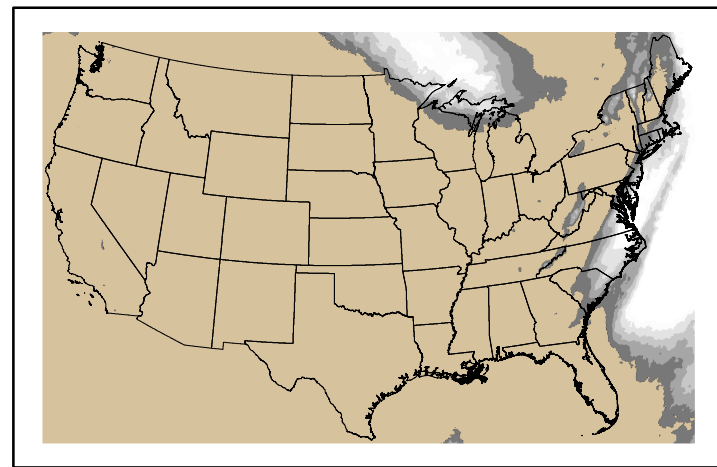
Precipitation p24m_2025022400f120.bil
