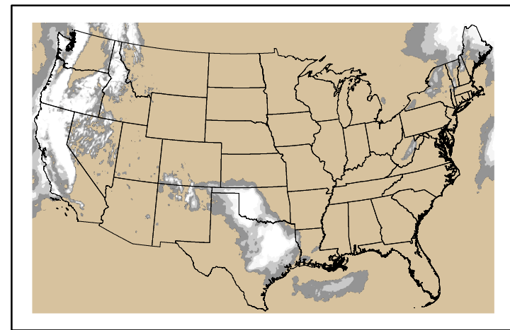
Precipitation p24m_2025022400f168.bil
