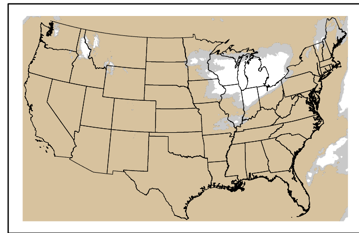
Precipitation p24m_2025022400f072.bil
