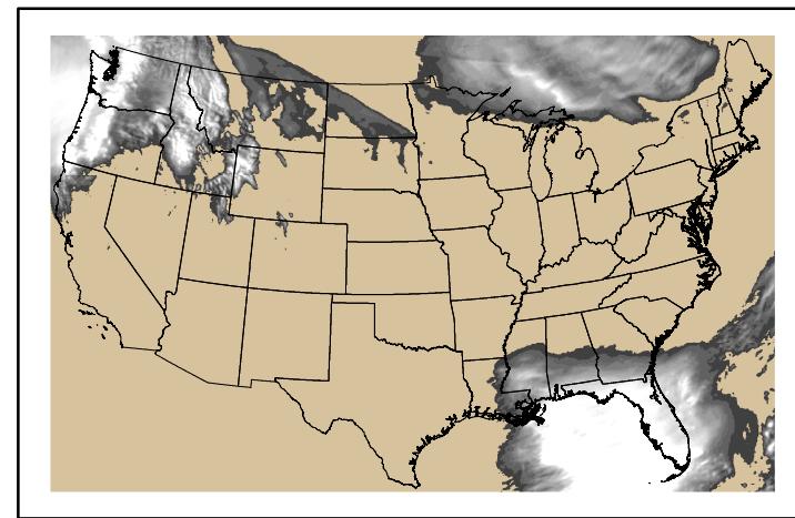
Precipitation p24m_2025022400f024.bil
