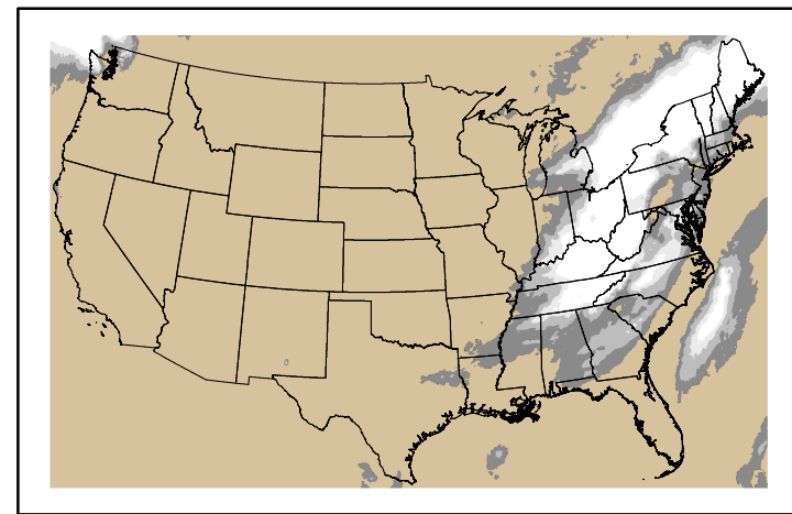
Precipitation p24m_2025022400f096.bil
