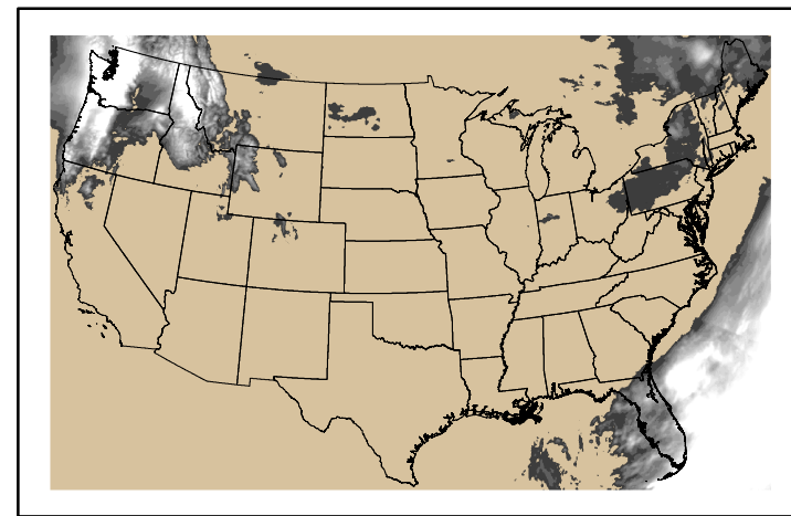
Precipitation p24m_2025022400f048.bil
