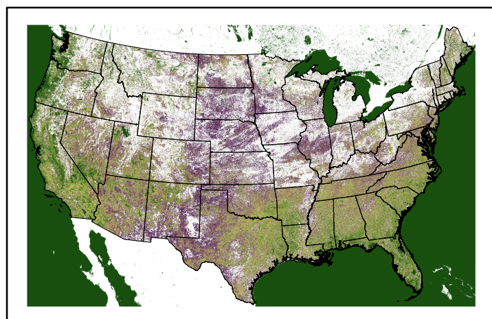
Greenness us25_048054wk_greenness.img
