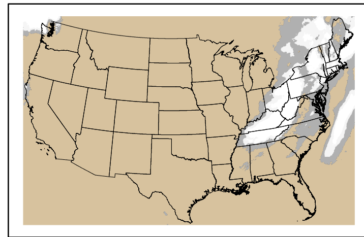
Precipitation p24m_2025022300f120.bil
