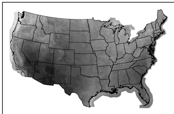
10hr Fuel Moisture mc10250301.bil
