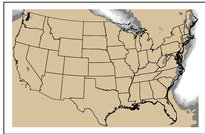
Precipitation p24m_2025022300f144.bil
