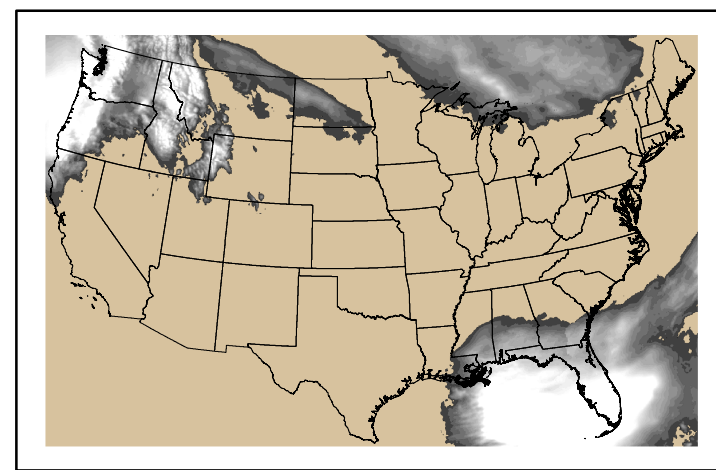
Precipitation p24m_2025022300f048.bil
