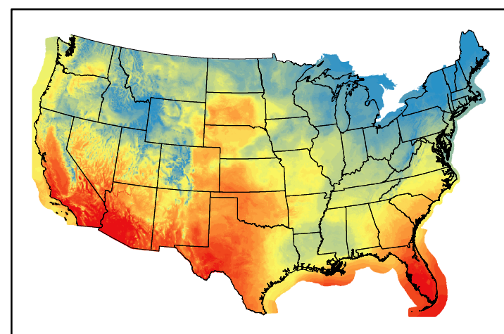
Dry Bulb Temp temp20250223.bil
