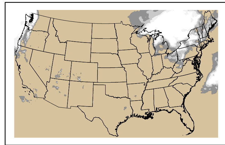
Precipitation p24m_2025022300f168.bil
