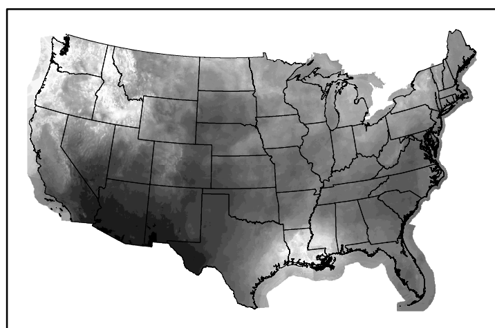
10hr Fuel Moisture mc10250223.bil
