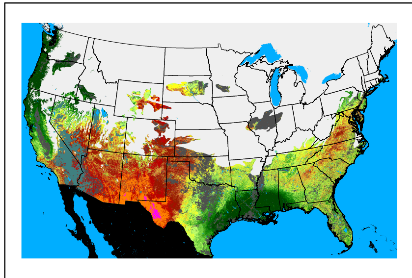
WFPI fp250223.bil
