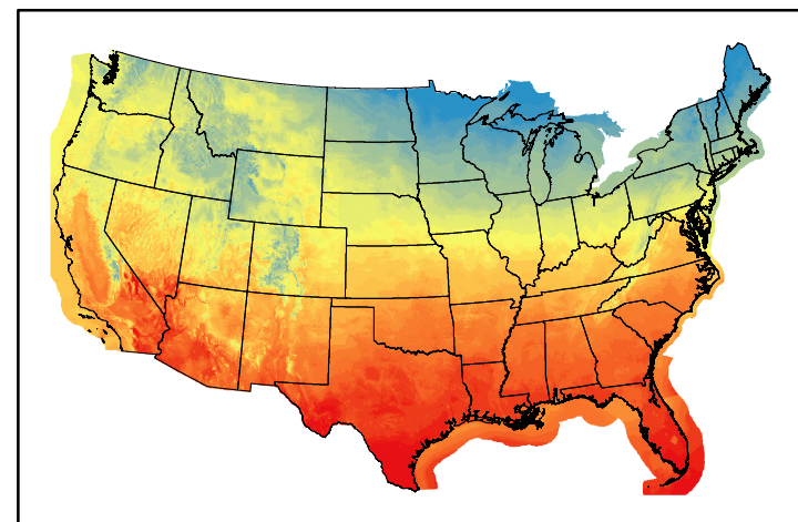
Dry Bulb Temp temp20250301.bil
