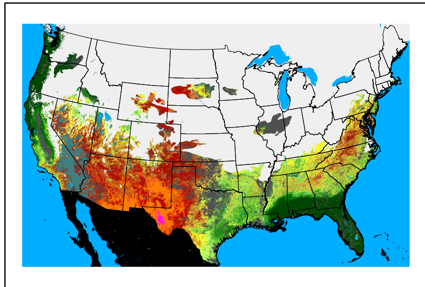
WFPI fp250224.bil
