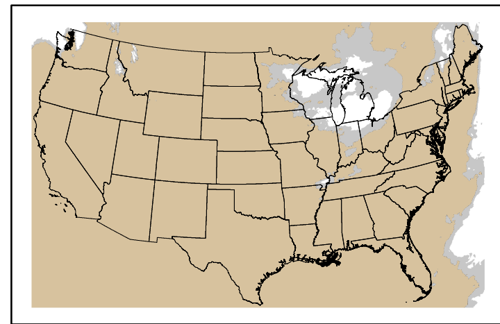
Precipitation p24m_2025022300f096.bil
