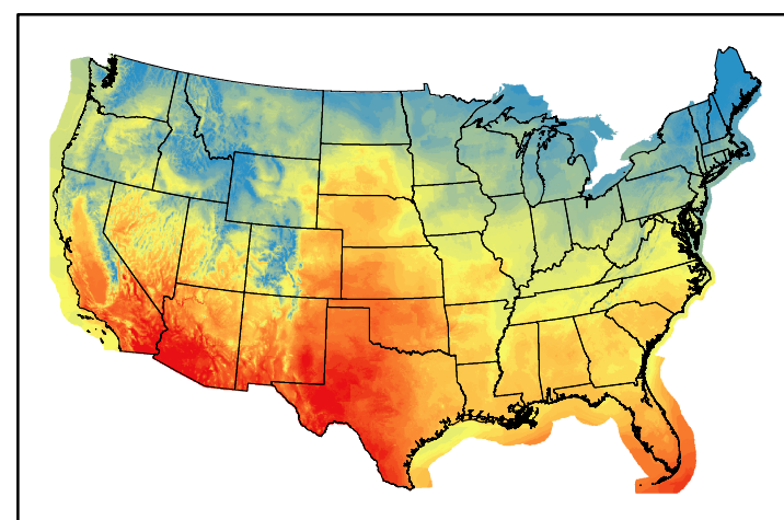
Dry Bulb Temp temp20250224.bil
