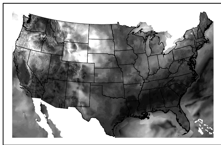
Wind Speed wspd20250224.bil
