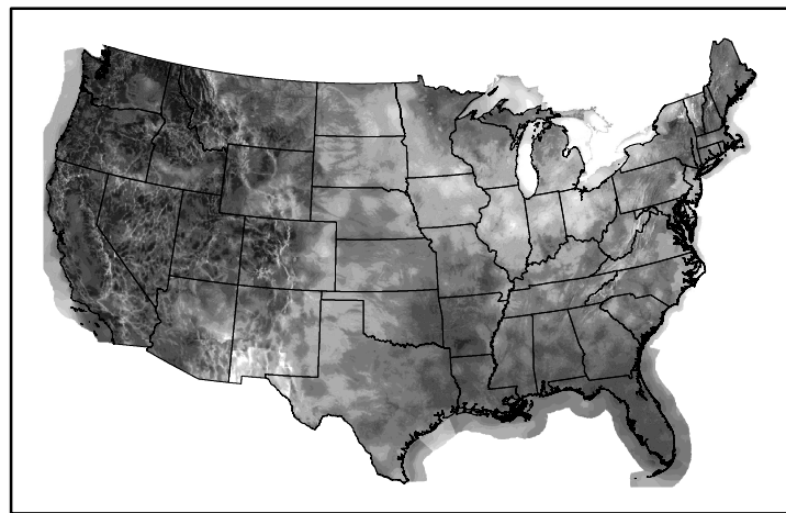
Wind Speed wspd20250301.bil
