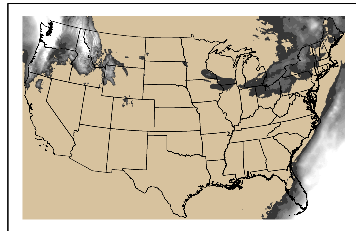
Precipitation p24m_2025022300f072.bil
