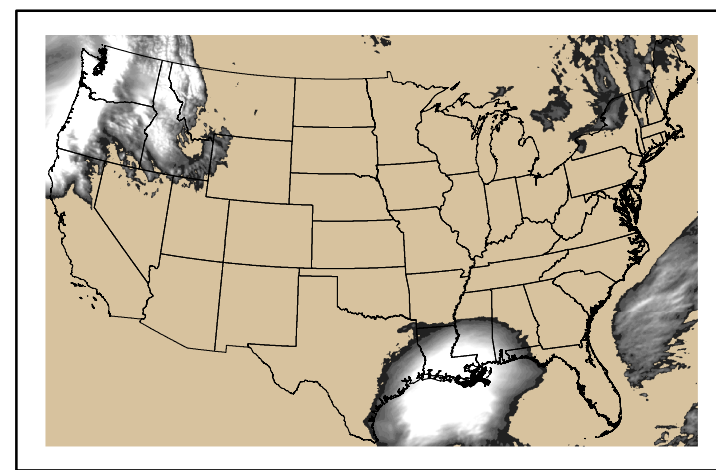
Precipitation p24m_2025022300f024.bil
