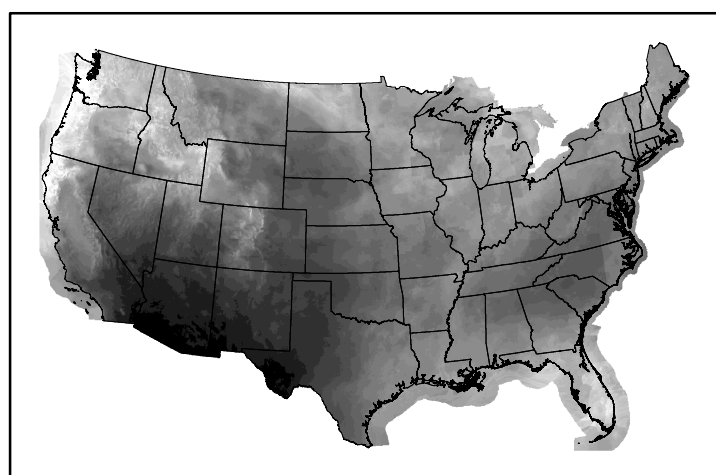
10hr Fuel Moisture mc10250224.bil
