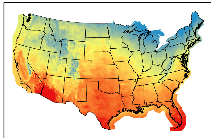
Dry Bulb Temp temp20250228.bil
