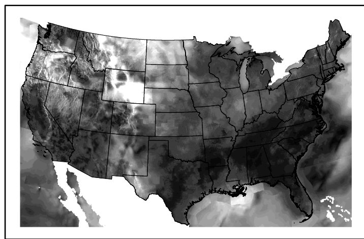
Wind Speed wspd20250223.bil
