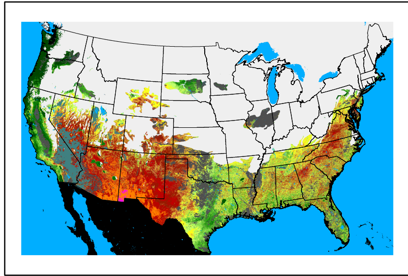
WFPI fp250301.bil
