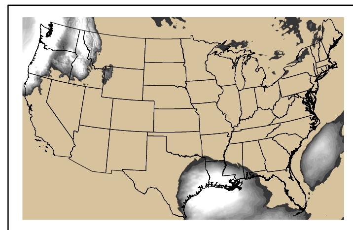
Precipitation p24m_2025022100f072.bil
