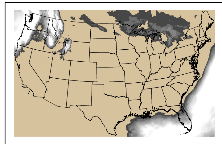
Precipitation p24m_2025022100f096.bil
