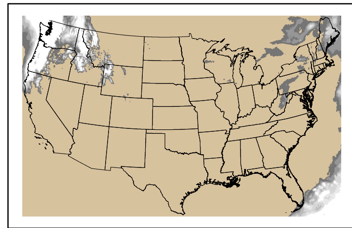
Precipitation p24m_2025022100f120.bil
