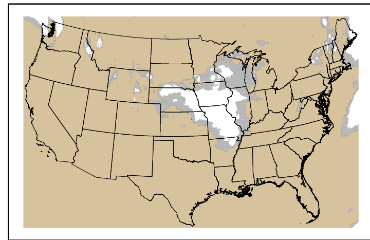
Precipitation p24m_2025022100f144.bil
