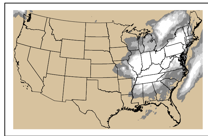
Precipitation p24m_2025022100f168.bil
