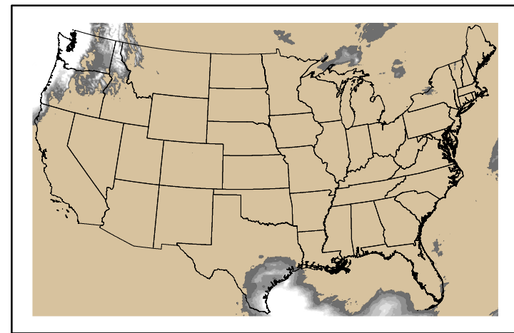
Precipitation p24m_2025022100f048.bil
