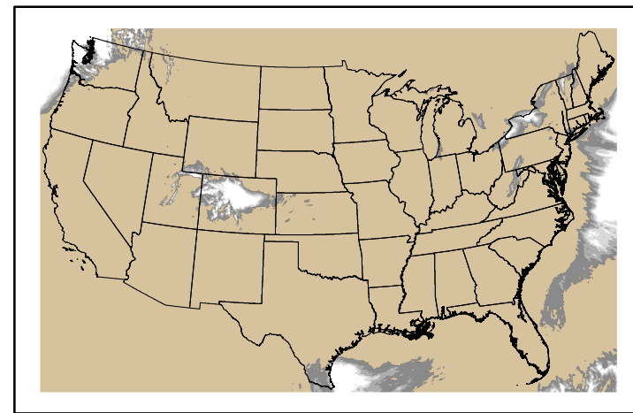
Precipitation p24m_2025022100f024.bil
