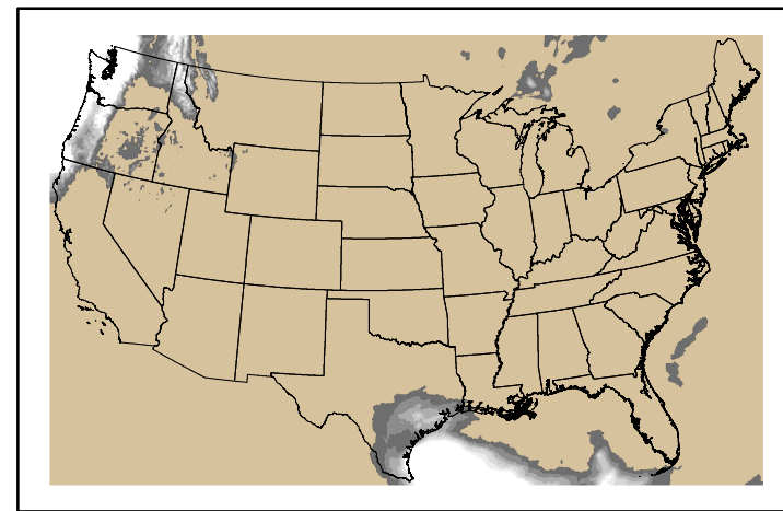
Precipitation p24m_2025022000f072.bil
