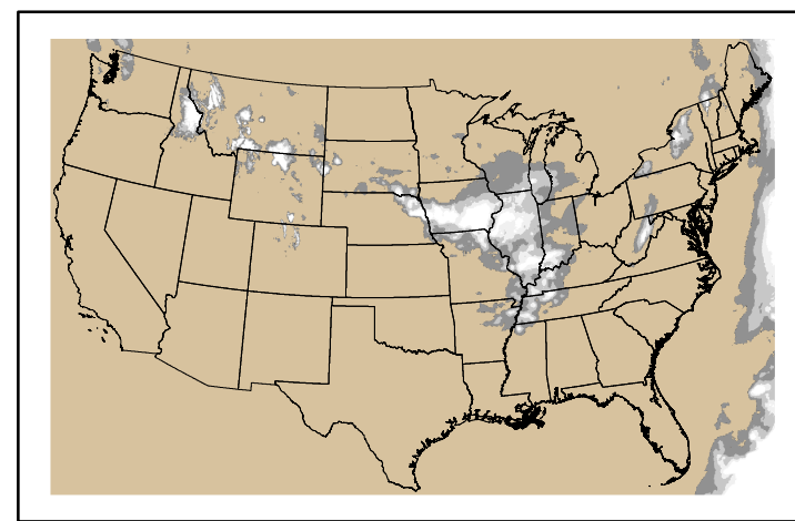
Precipitation p24m_2025022000f168.bil
