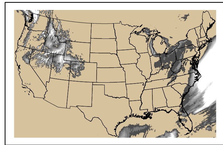
Precipitation p24m_2025022000f024.bil
