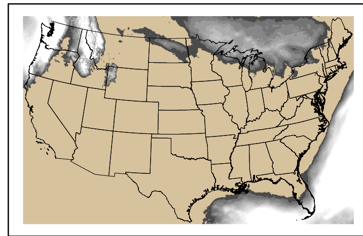
Precipitation p24m_2025022000f120.bil
