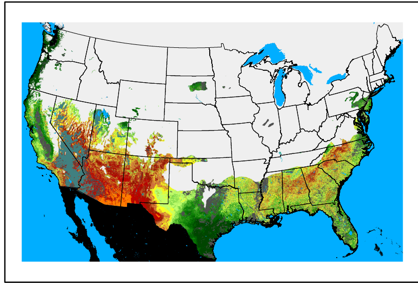
WFPI fp250222.bil
