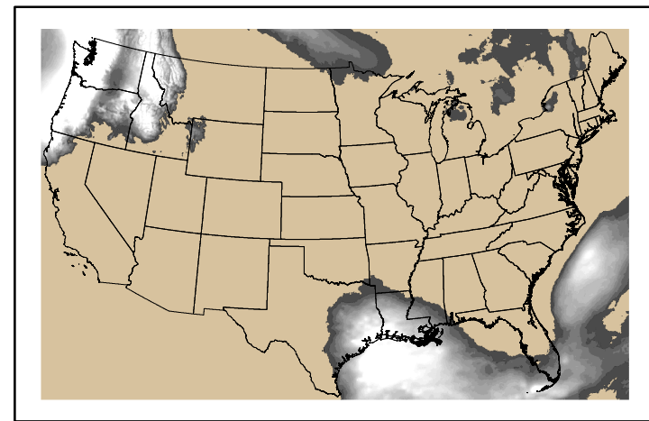
Precipitation p24m_2025022000f096.bil
