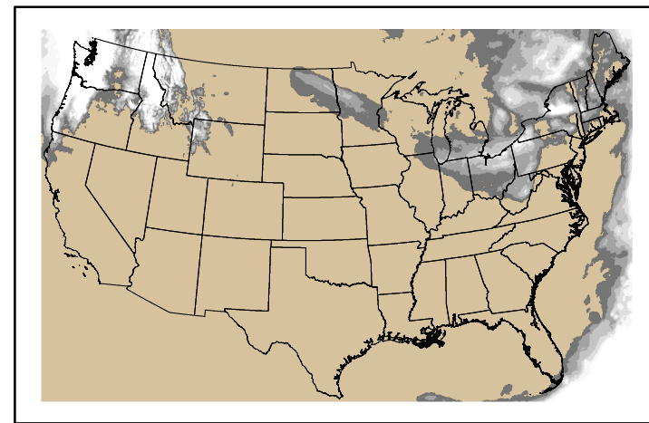
Precipitation p24m_2025022000f144.bil
