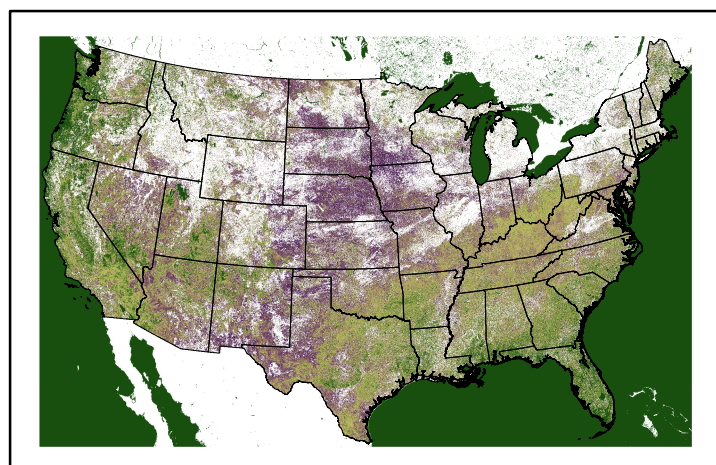
Greenness us25_041047wk_greenness.img
