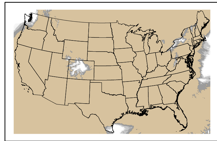
Precipitation p24m_2025022000f048.bil
