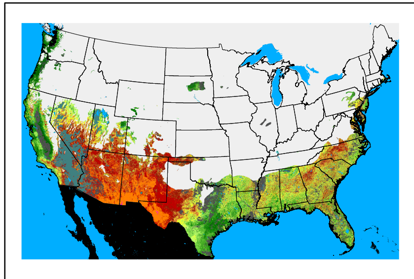
WFPI fp250226.bil
