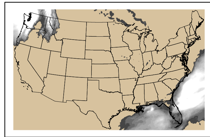
Precipitation p24m_2025021700f168.bil
