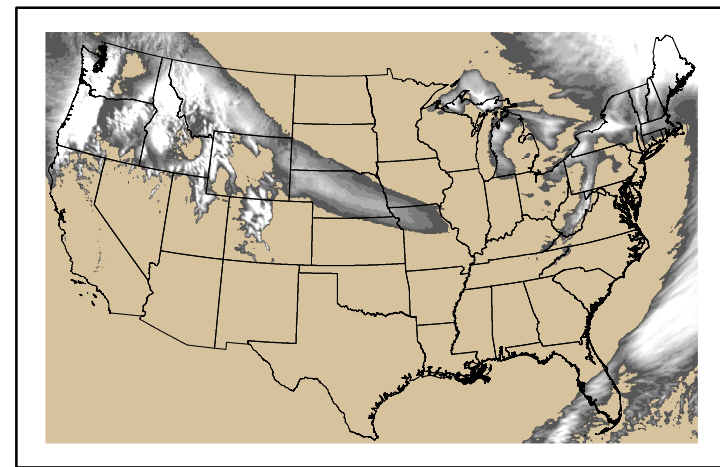
Precipitation p24m_2025021700f024.bil
