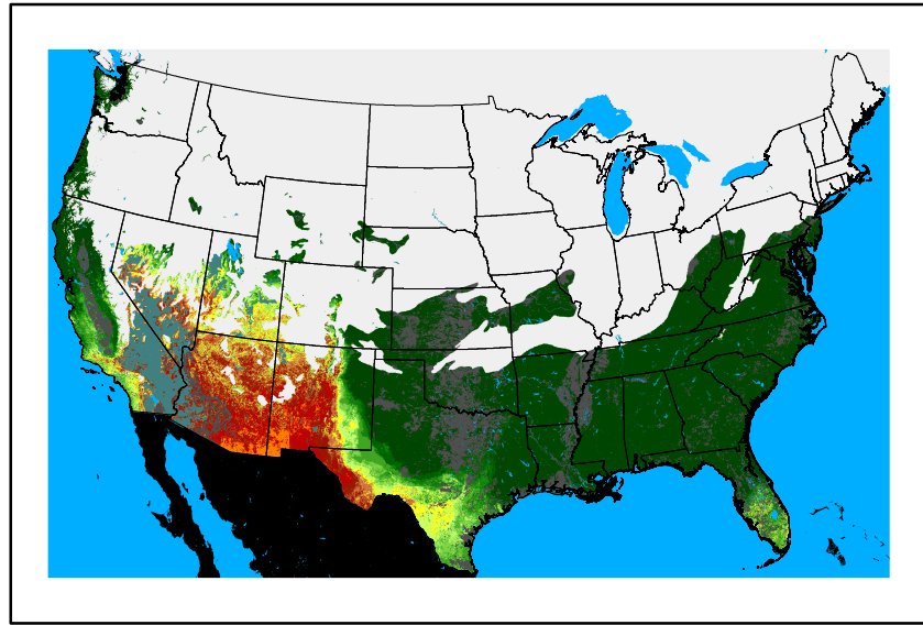
WFPI fp250219.bil
