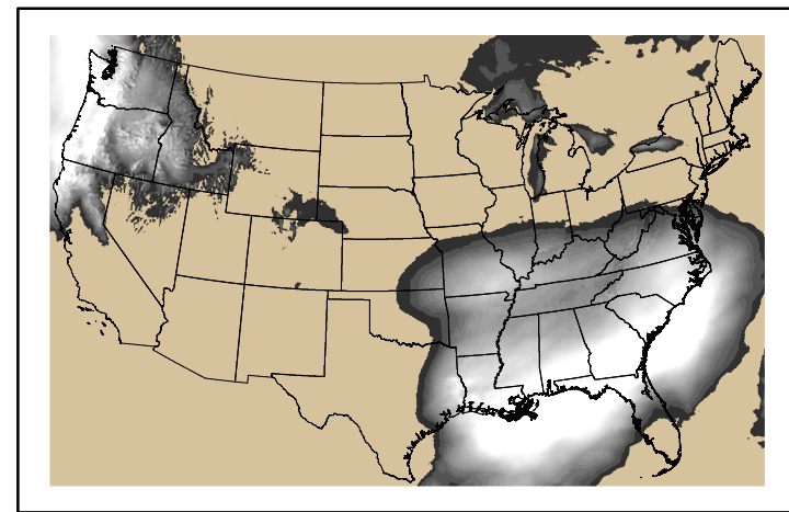
Precipitation p24m_2025021700f072.bil
