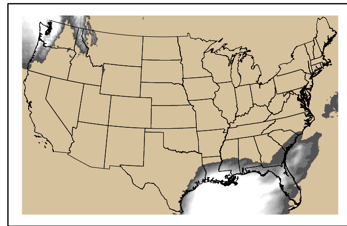
Precipitation p24m_2025021700f144.bil
