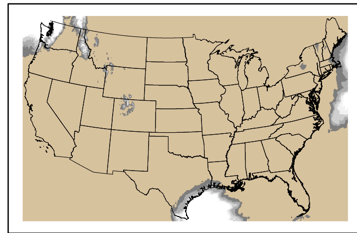
Precipitation p24m_2025021700f120.bil
