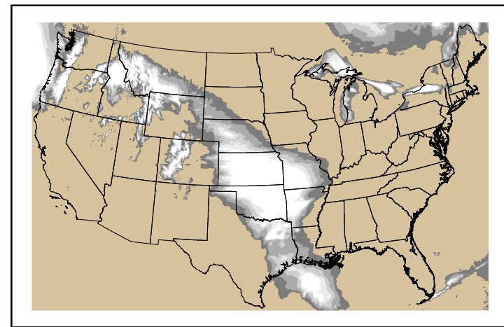
Precipitation p24m_2025021700f048.bil
