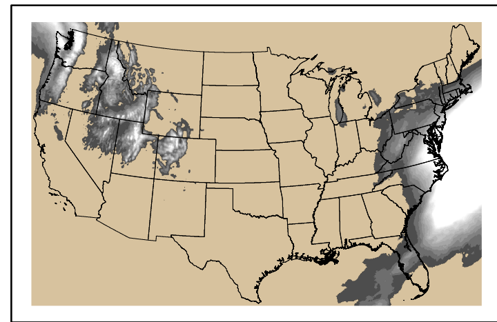
Precipitation p24m_2025021700f096.bil
