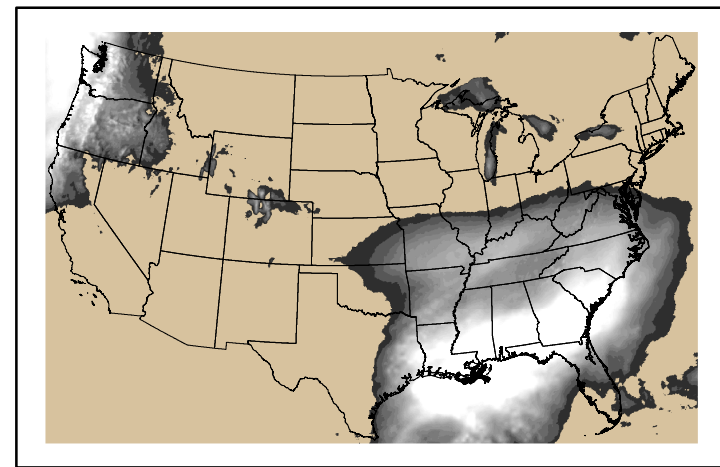
Precipitation p24m_2025021600f096.bil
