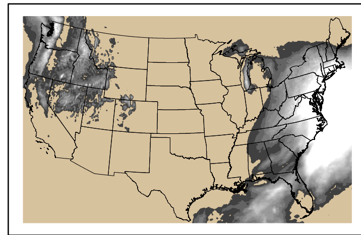
Precipitation p24m_2025021600f120.bil
