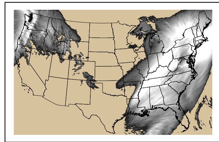
Precipitation p24m_2025021600f024.bil
