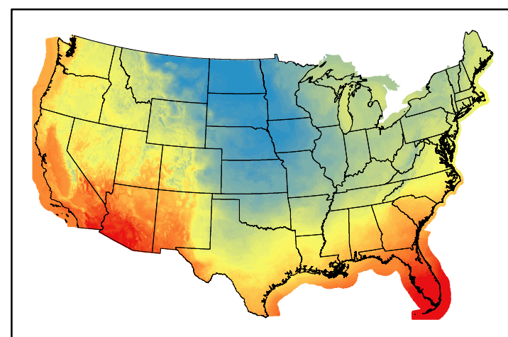
Dry Bulb Temp temp20250220.bil
