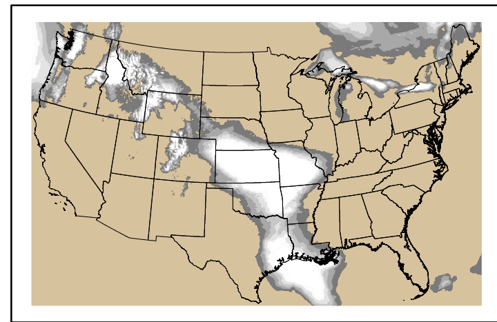
Precipitation p24m_2025021600f072.bil
