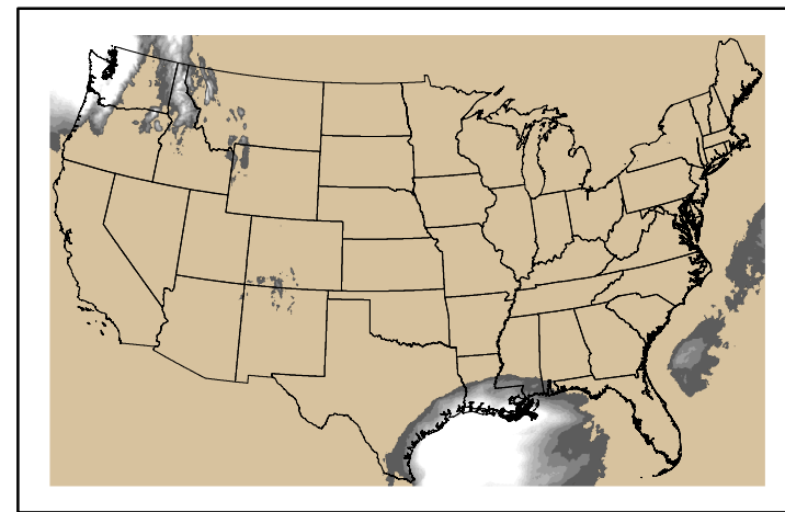
Precipitation p24m_2025021600f168.bil
