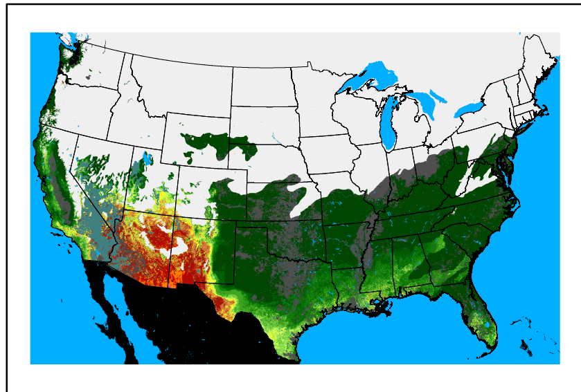
WFPI fp250220.bil
