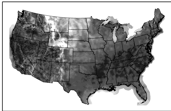
Wind Speed wspd20250222.bil
