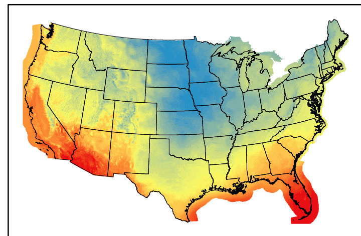
Dry Bulb Temp temp20250221.bil
