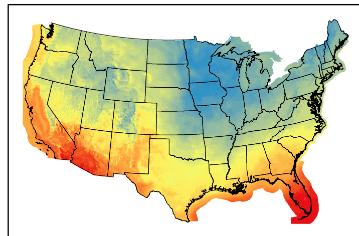
Dry Bulb Temp temp20250222.bil
