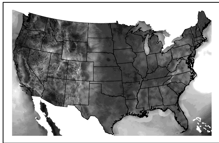
Wind Speed wspd20250220.bil
