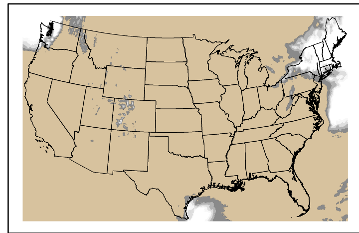
Precipitation p24m_2025021600f144.bil
