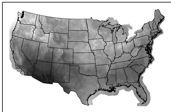
10hr Fuel Moisture mc10250222.bil
