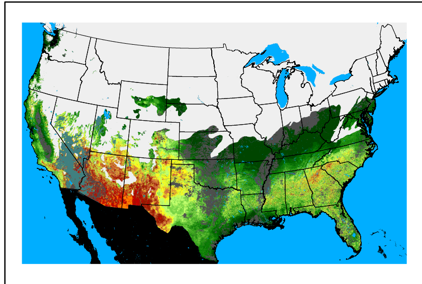
WFPI fp250222.bil
