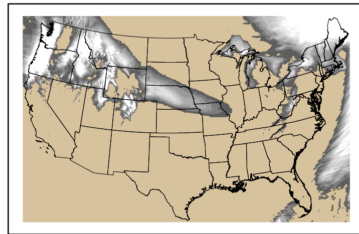
Precipitation p24m_2025021600f048.bil
