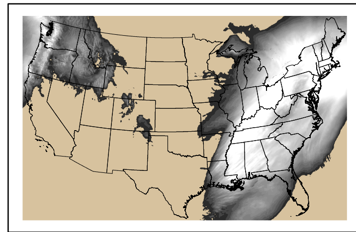
Precipitation p24m_2025021500f048.bil
