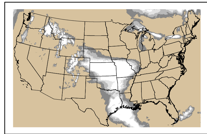
Precipitation p24m_2025021500f096.bil
