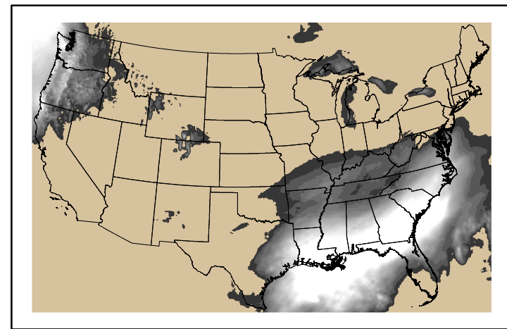
Precipitation p24m_2025021500f120.bil
