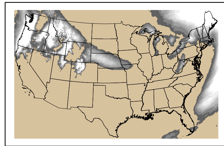
Precipitation p24m_2025021500f072.bil
