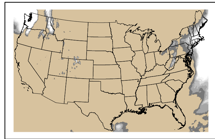
Precipitation p24m_2025021500f168.bil
