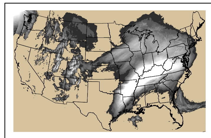
Precipitation p24m_2025021500f024.bil
