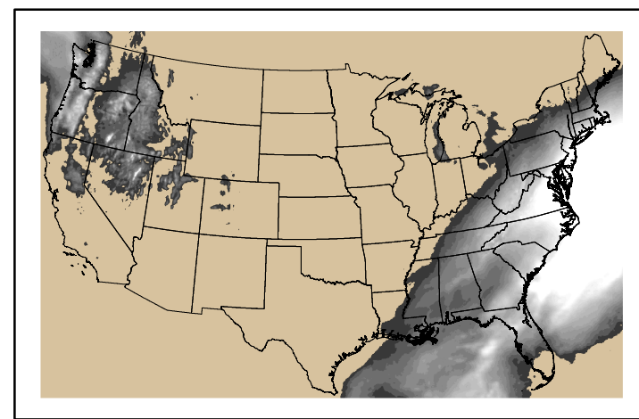
Precipitation p24m_2025021500f144.bil
