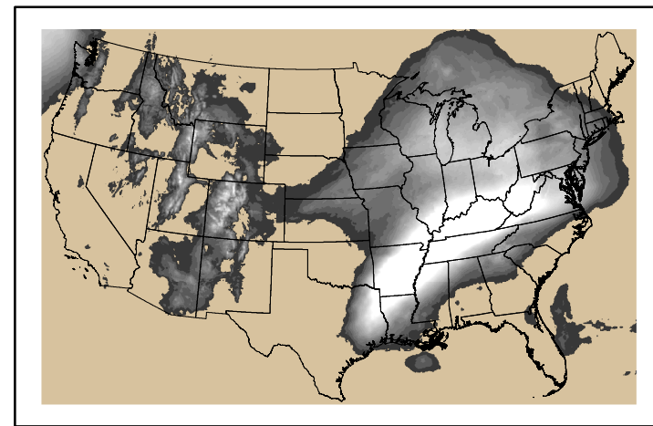
Precipitation p24m_2025021300f072.bil
