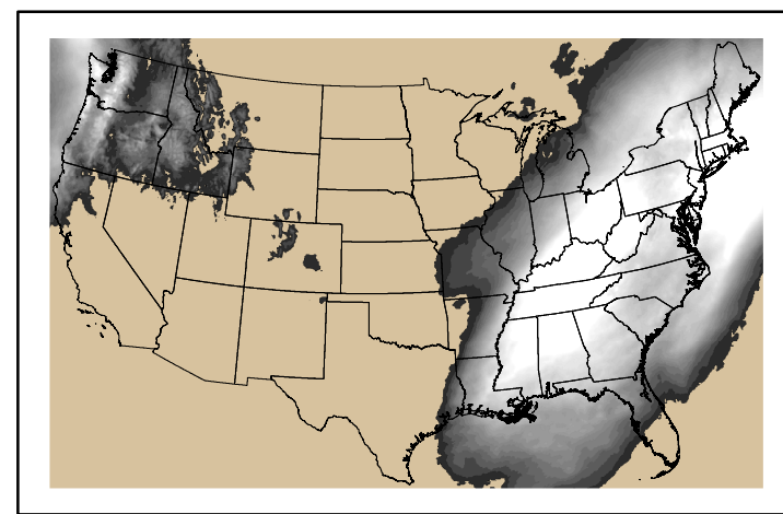
Precipitation p24m_2025021300f096.bil
