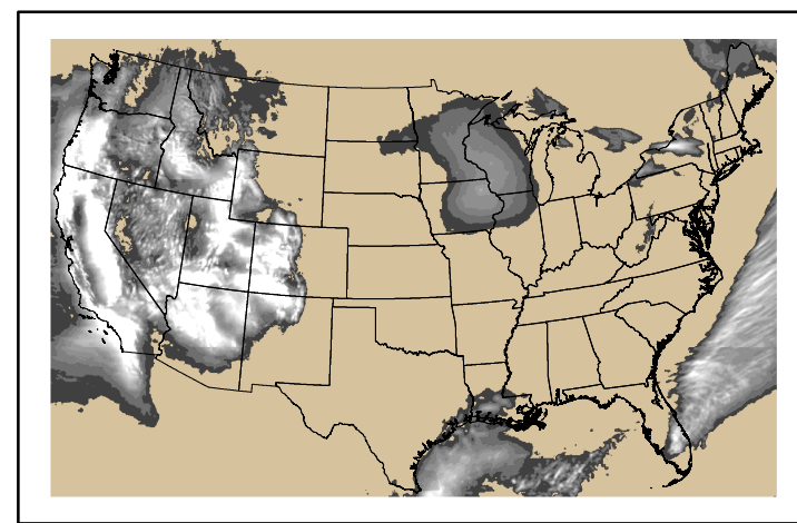
Precipitation p24m_2025021300f048.bil
