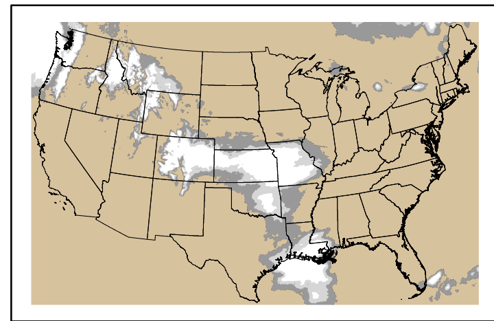
Precipitation p24m_2025021300f144.bil
