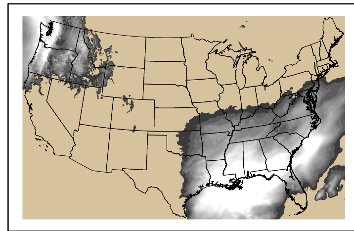
Precipitation p24m_2025021300f168.bil
