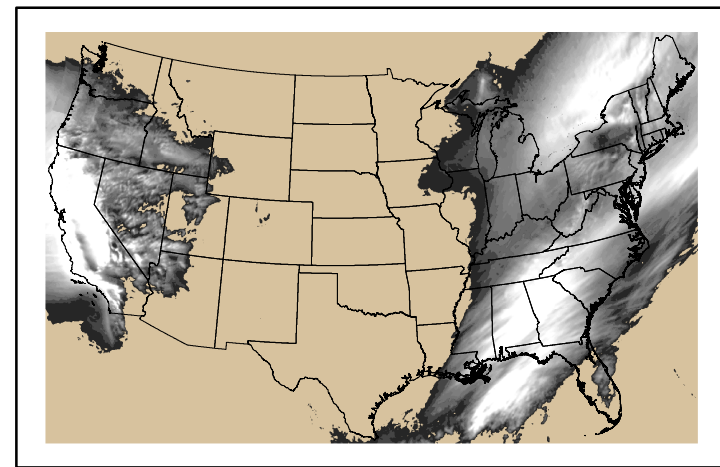
Precipitation p24m_2025021300f024.bil
