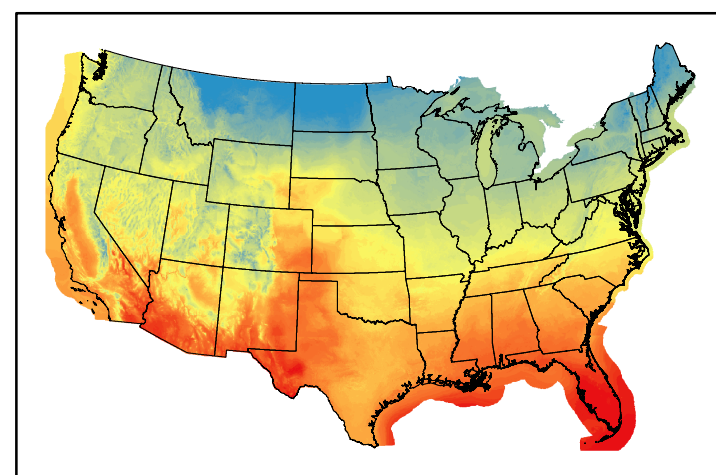
Dry Bulb Temp temp20250214.bil
