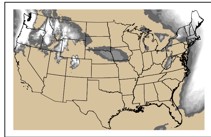
Precipitation p24m_2025021300f120.bil
