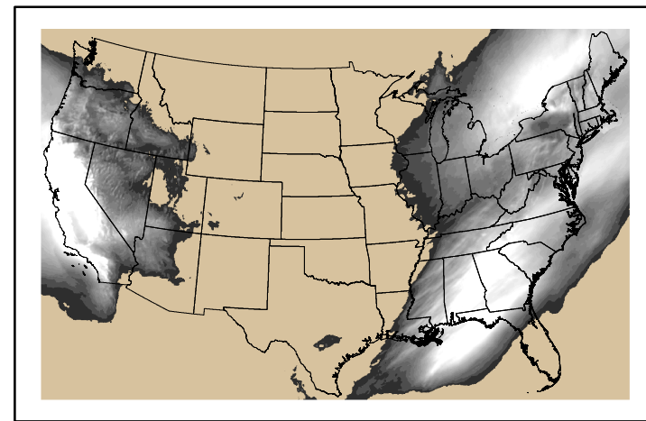
Precipitation p24m_2025021200f048.bil
