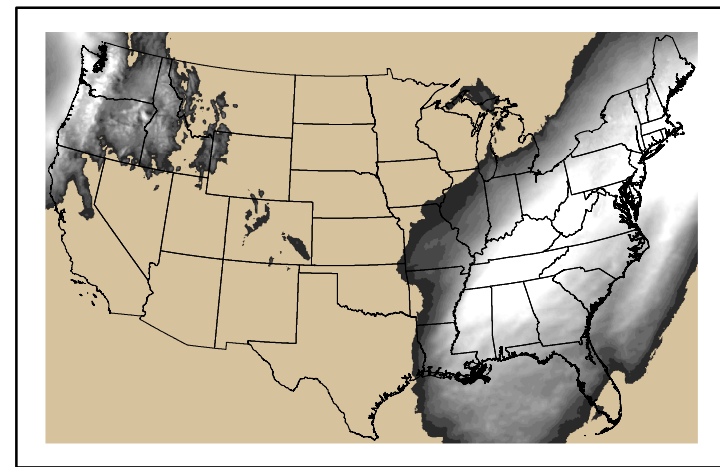
Precipitation p24m_2025021200f120.bil
