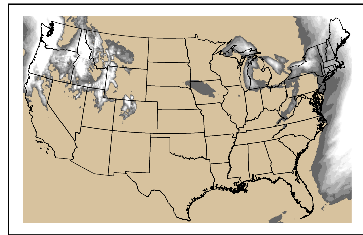
Precipitation p24m_2025021200f144.bil
