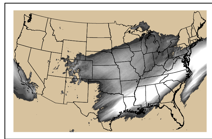
Precipitation p24m_2025021200f024.bil
