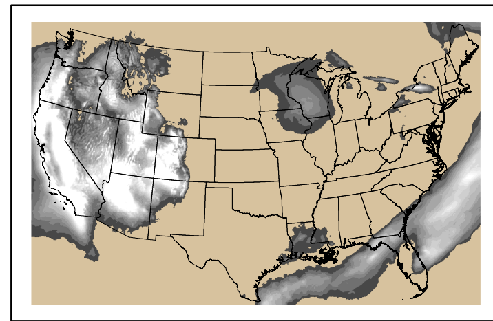
Precipitation p24m_2025021200f072.bil
