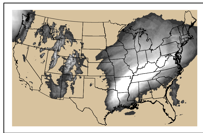
Precipitation p24m_2025021200f096.bil
