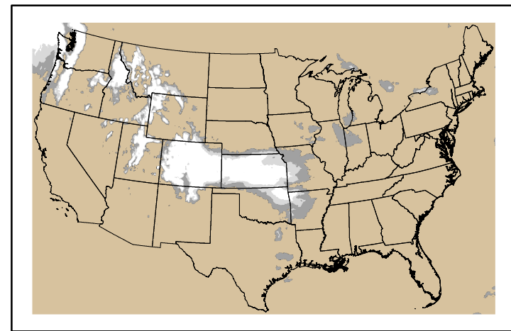
Precipitation p24m_2025021200f168.bil
