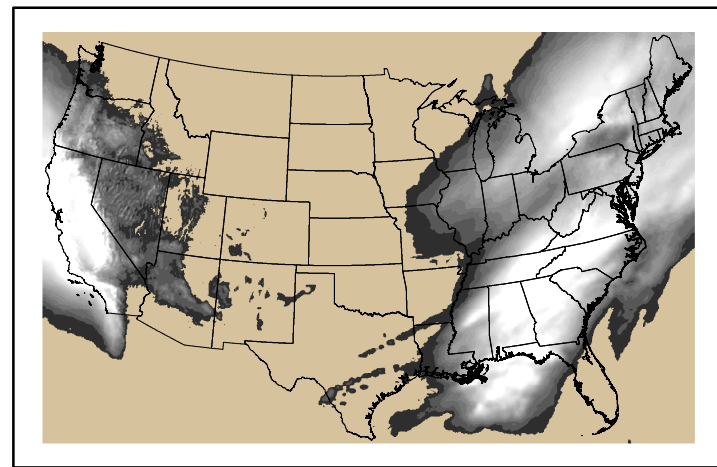
Precipitation p24m_2025021000f096.bil
