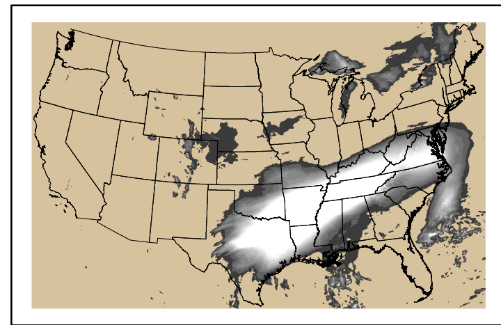
Precipitation p24m_2025021000f048.bil
