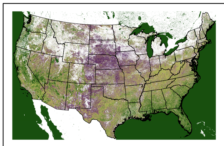
Greenness us25_034040wk_greenness.img
