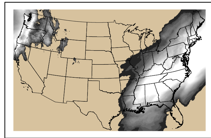
Precipitation p24m_2025021000f168.bil
