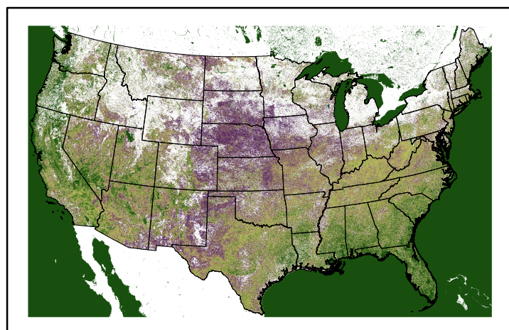
Greenness us25_034040wk_greenness.img
