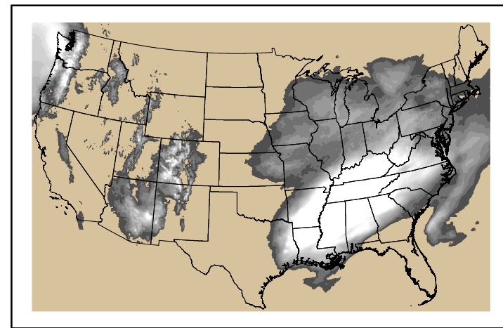
Precipitation p24m_2025021000f144.bil
