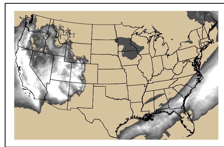
Precipitation p24m_2025021000f120.bil
