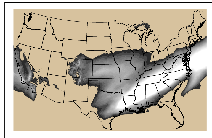
Precipitation p24m_2025021000f072.bil
