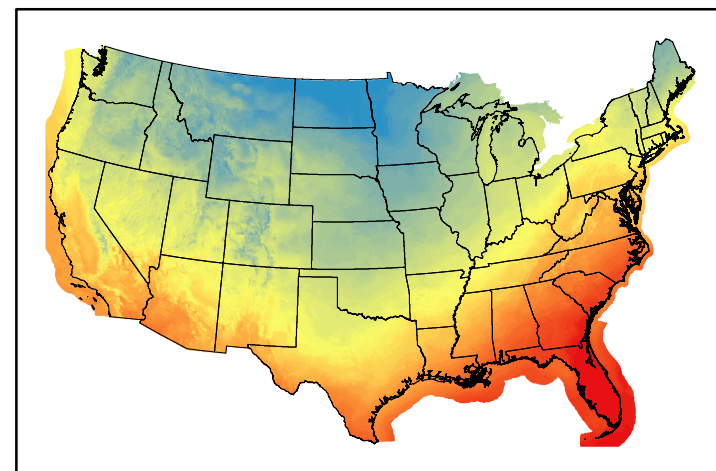
Dry Bulb Temp temp20250213.bil
