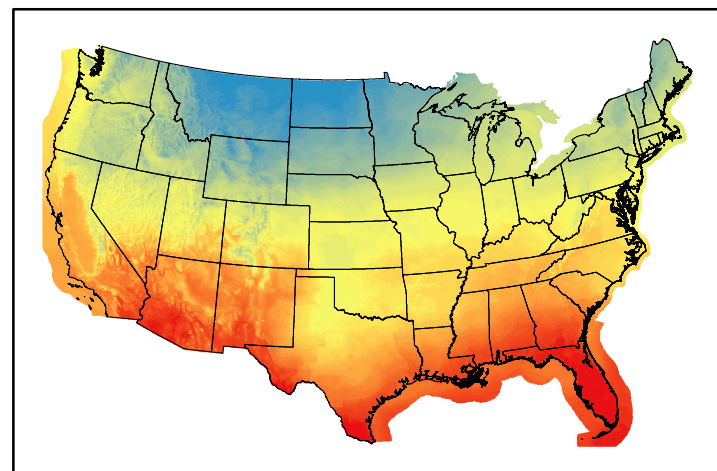
Dry Bulb Temp temp20250210.bil
