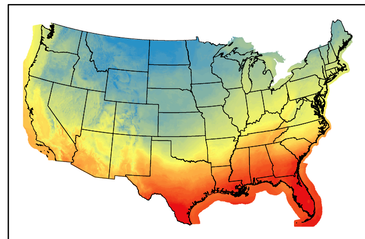
Dry Bulb Temp temp20250212.bil
