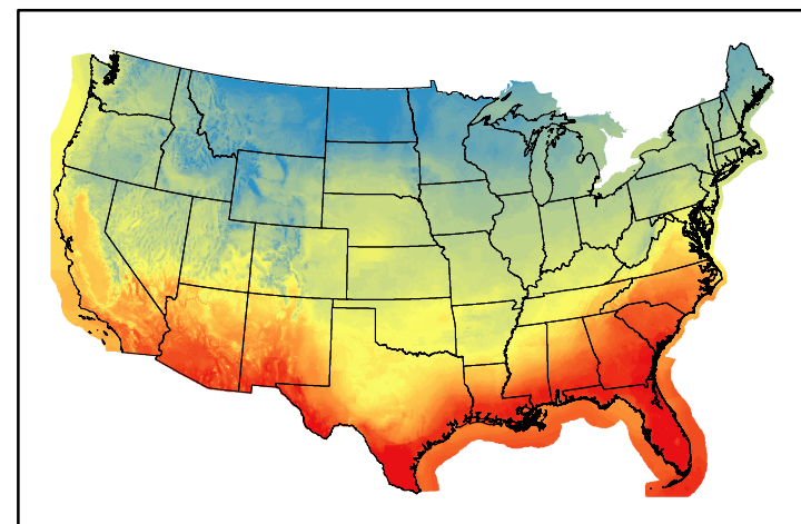
Dry Bulb Temp temp20250209.bil
