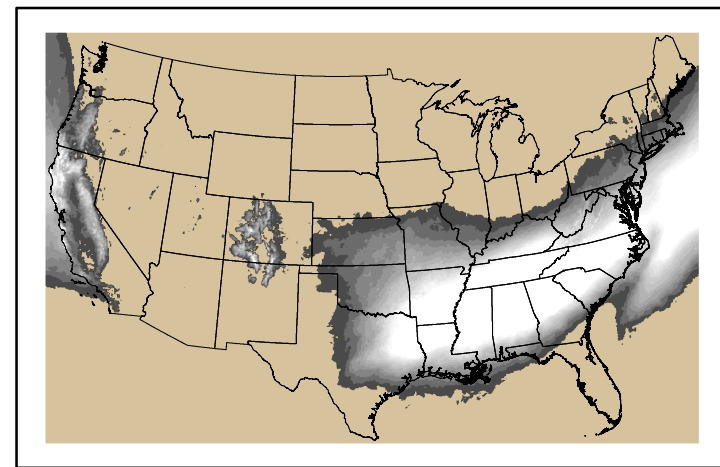
Precipitation p24m_2025020700f144.bil
