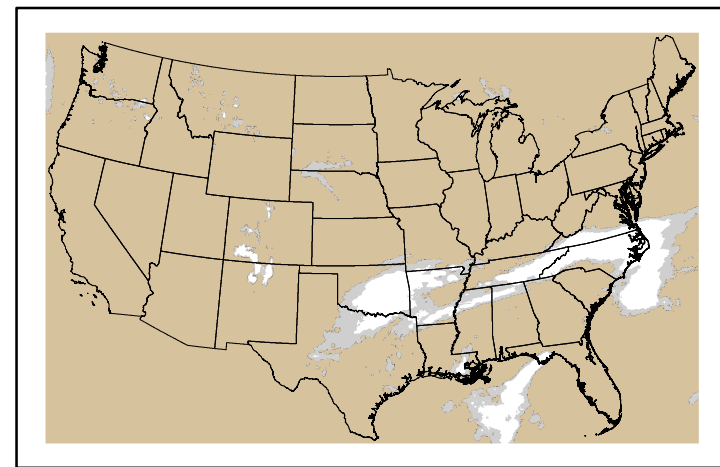
Precipitation p24m_2025020700f096.bil
