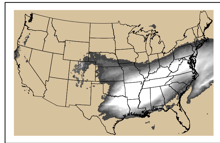
Precipitation p24m_2025020700f120.bil
