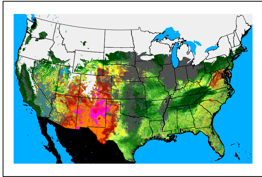
WFPI fp250207.bil
