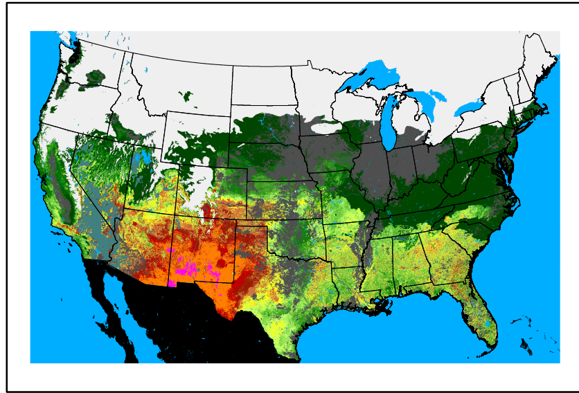
WFPI fp250208.bil
