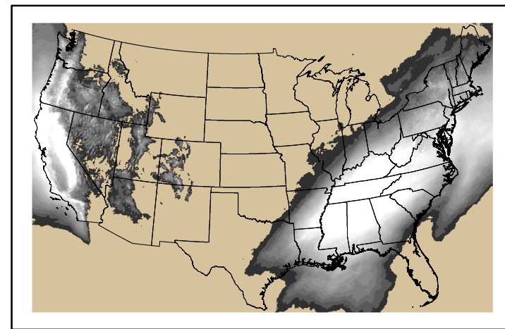
Precipitation p24m_2025020700f168.bil
