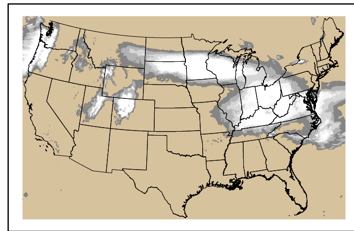
Precipitation p24m_2025020700f048.bil
