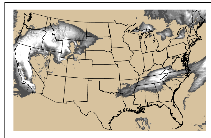
Precipitation p24m_2025020700f024.bil
