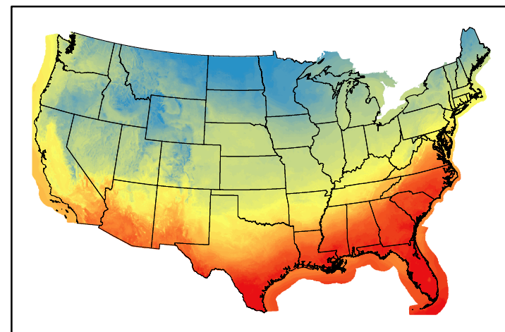
Dry Bulb Temp temp20250209.bil
