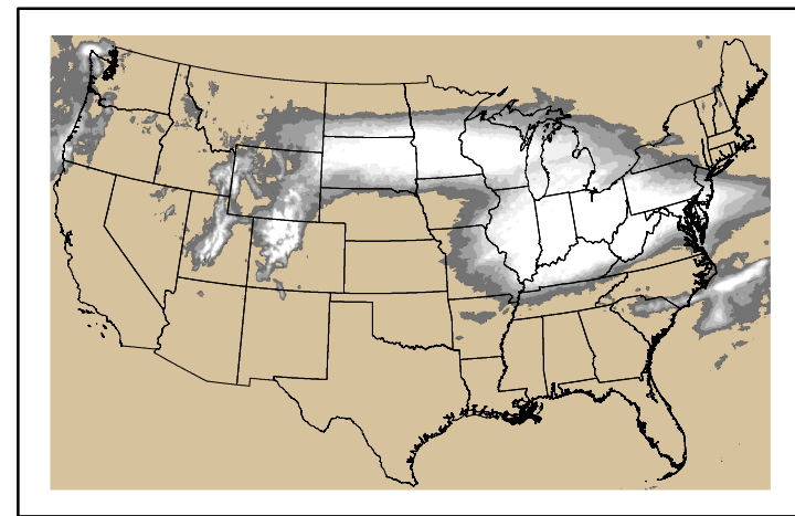
Precipitation p24m_2025020500f096.bil
