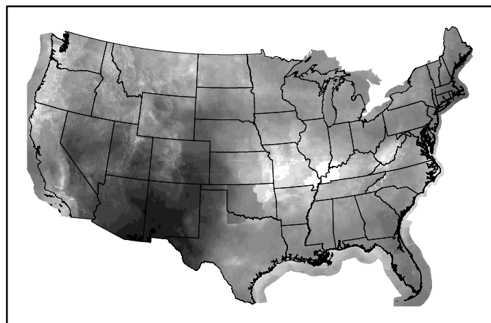
10hr Fuel Moisture mc10250205.bil
