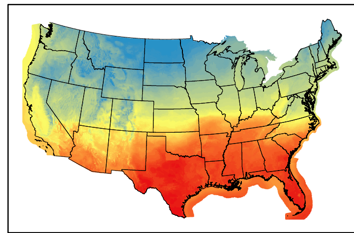
Dry Bulb Temp temp20250208.bil
