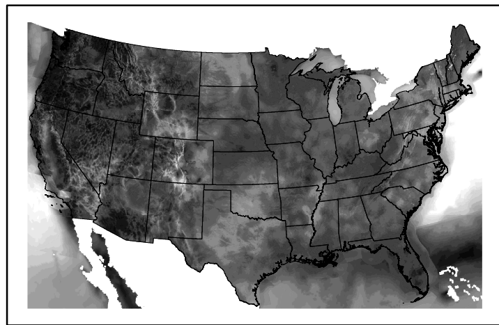
Wind Speed wspd20250209.bil
