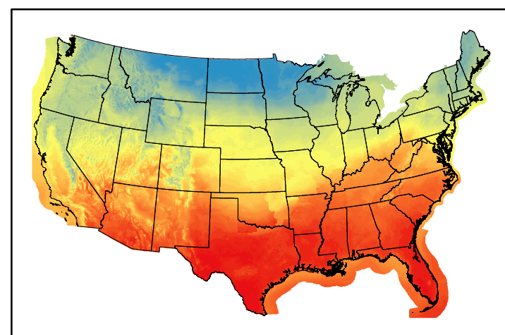
Dry Bulb Temp temp20250206.bil
