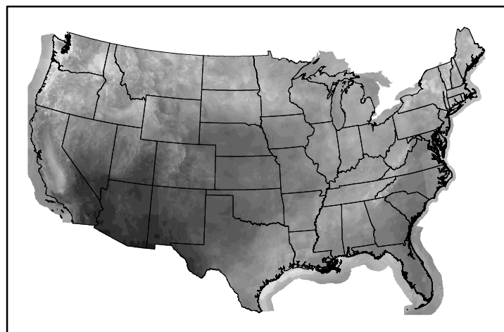
10hr Fuel Moisture mc10250209.bil
