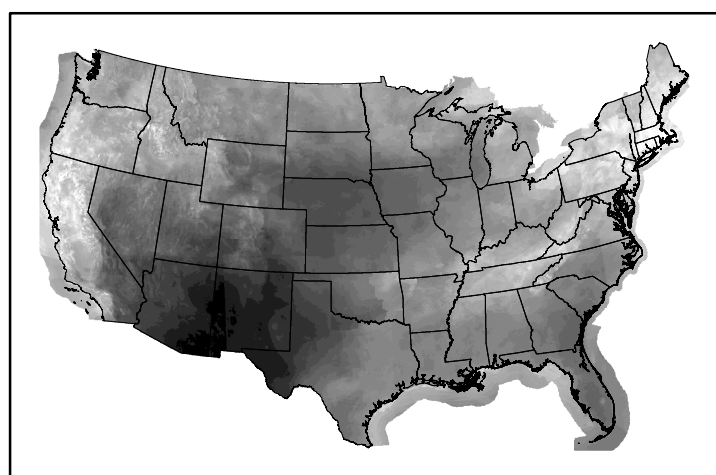
10hr Fuel Moisture mc10250206.bil
