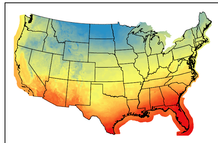
Dry Bulb Temp temp20250210.bil
