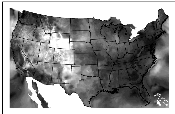
Wind Speed wspd20250205.bil
