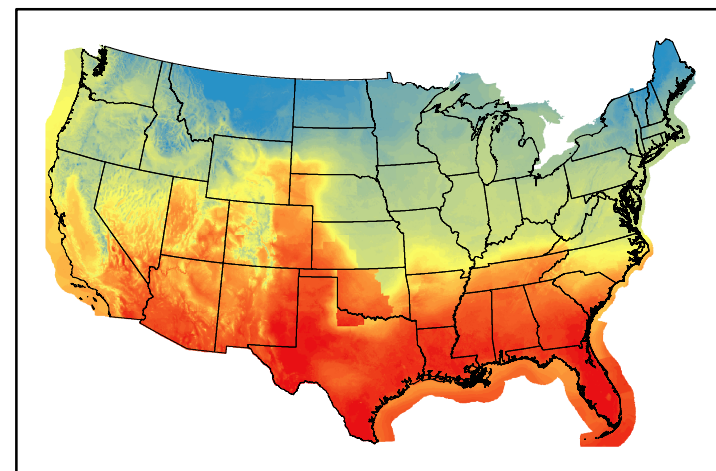
Dry Bulb Temp temp20250205.bil
