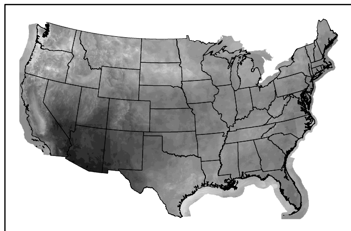
10hr Fuel Moisture mc10250210.bil
