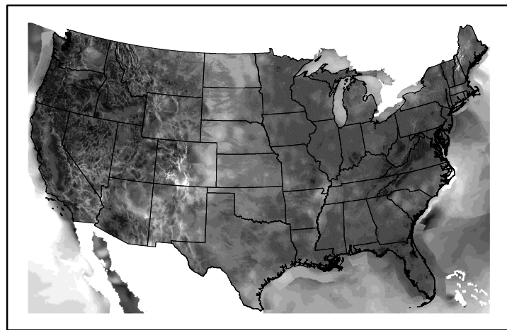
Wind Speed wspd20250210.bil
