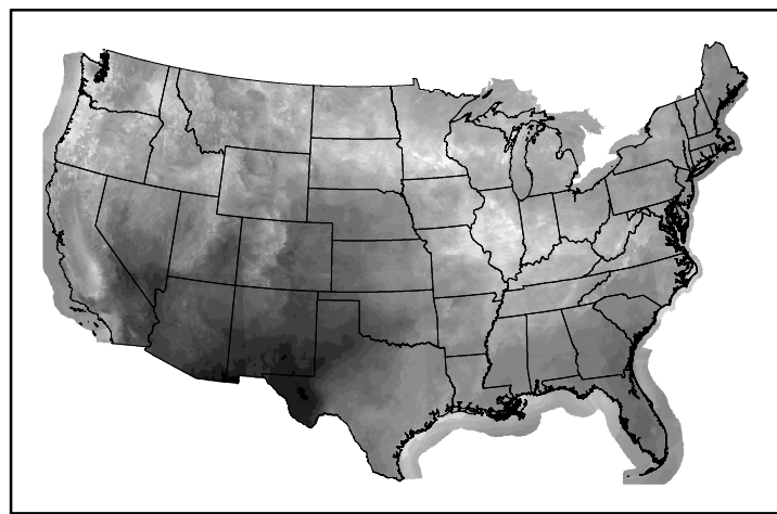
10hr Fuel Moisture mc10250208.bil
