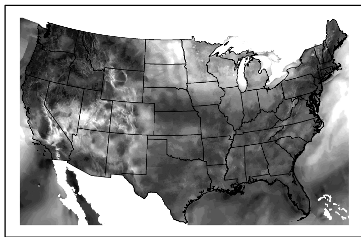
Wind Speed wspd20250206.bil
