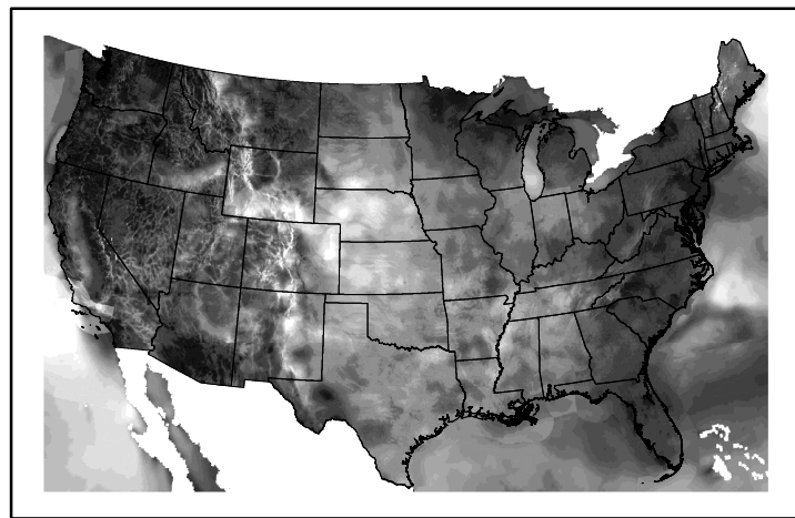
Wind Speed wspd20250208.bil
