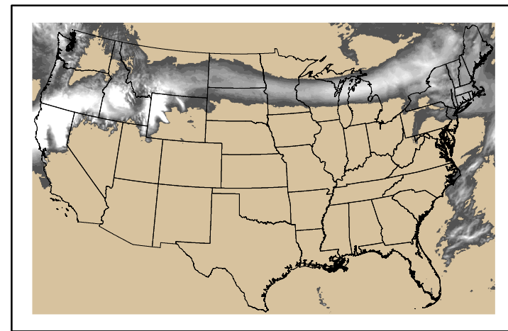
Precipitation p24m_2025020300f024.bil
