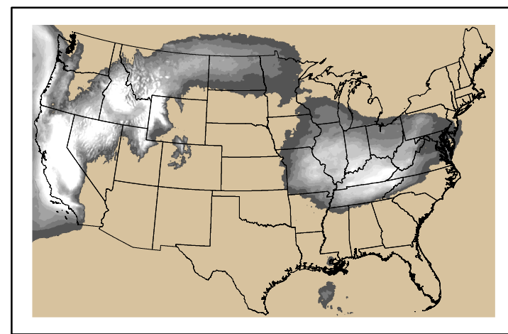
Precipitation p24m_2025020300f072.bil
