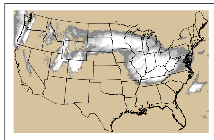
Precipitation p24m_2025020300f144.bil
