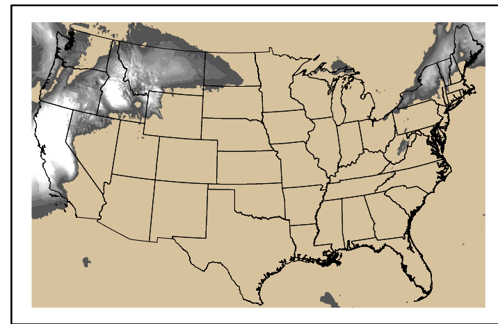
Precipitation p24m_2025020300f048.bil
