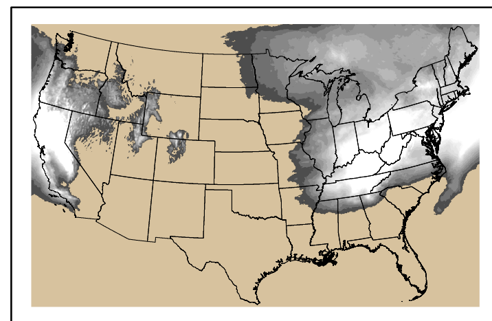
Precipitation p24m_2025020300f096.bil
