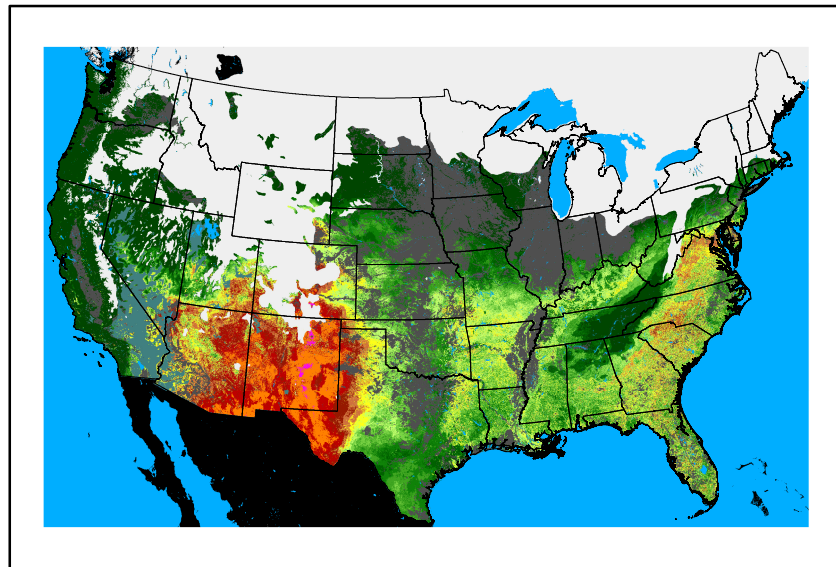
WFPI fp250207.bil
