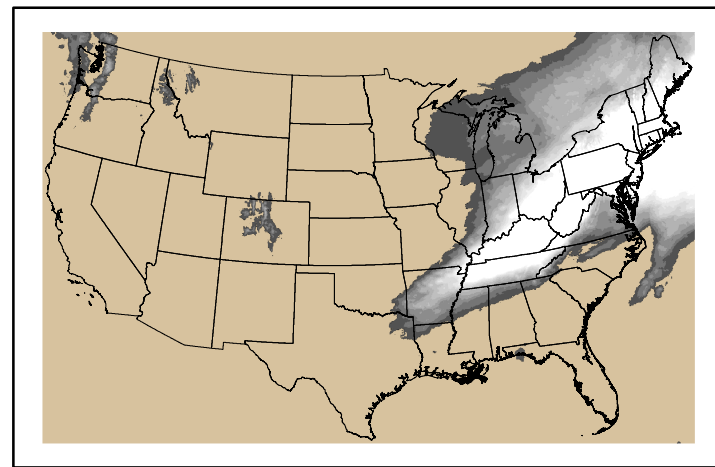
Precipitation p24m_2025020300f168.bil
