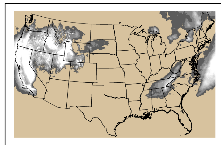
Precipitation p24m_2025020300f120.bil
