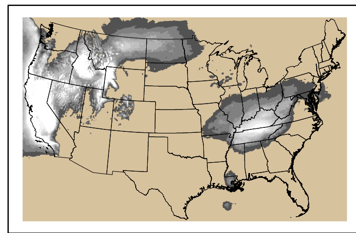
Precipitation p24m_20250200f096.bil
