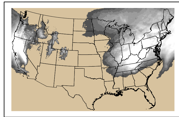
Precipitation p24m_2025020200f120.bil
