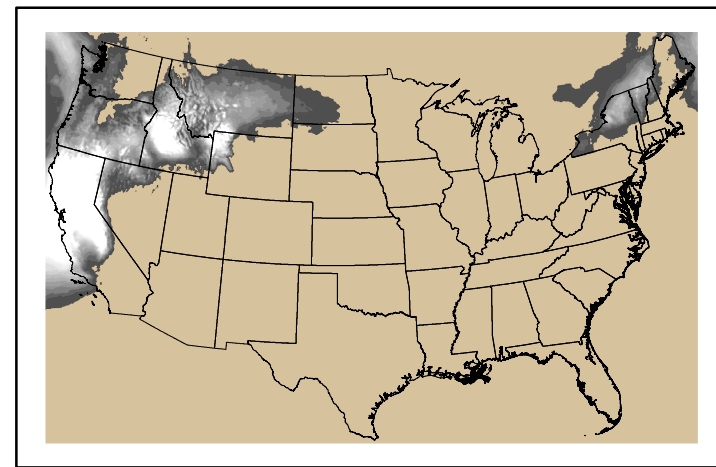
Precipitation p24m_20250200f072.bil
