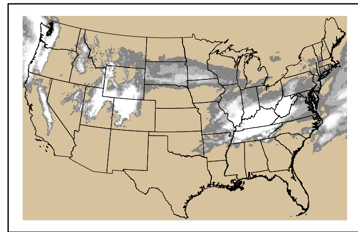
Precipitation p24m_20250200f168.bil
