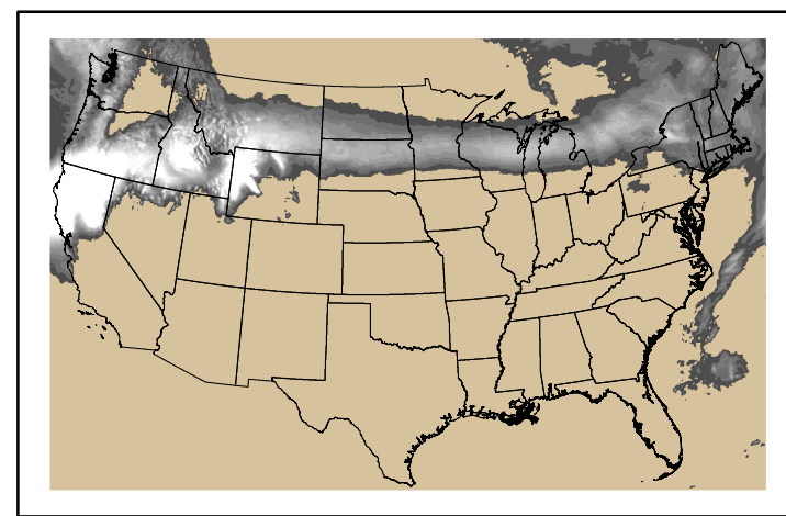
Precipitation p24m_20250200f048.bil
