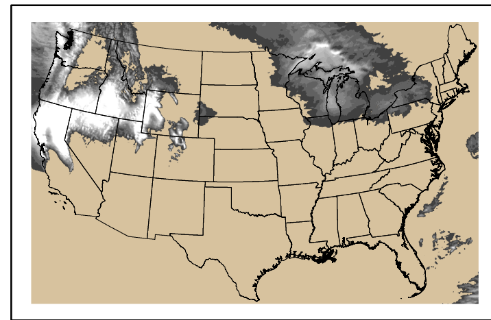
Precipitation p24m_2025020200f024.bil
