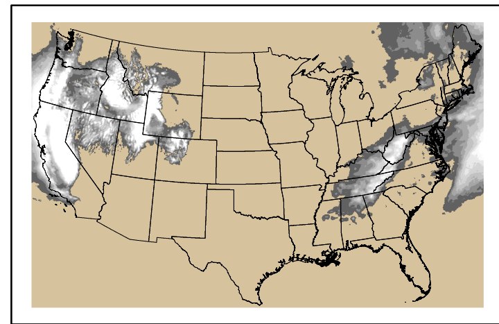
Precipitation p24m_20250200f144.bil
