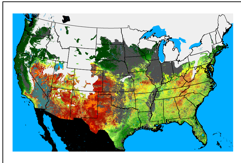
WFPI fp250203.bil
