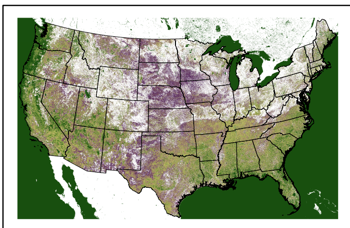
Greenness us25_020026wk_greenness.img
