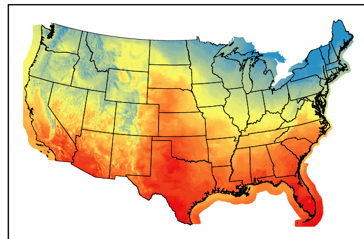
Dry Bulb Temp temp20250201.bil
