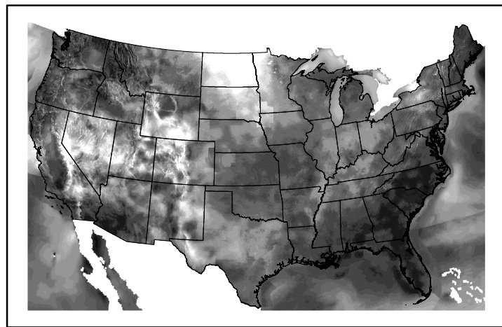
Wind Speed wspd20250202.bil
