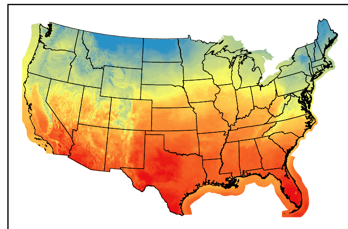
Dry Bulb Temp temp20250202.bil
