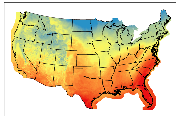
Dry Bulb Temp temp20250131.bil
