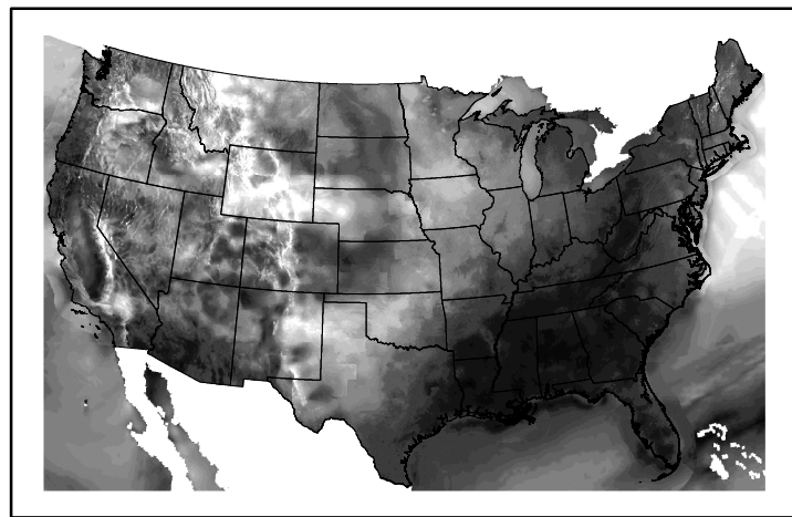
Wind Speed wspd20250201.bil
