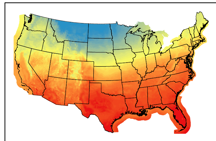
Dry Bulb Temp temp20250203.bil
