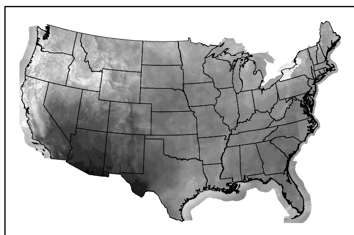
10hr Fuel Moisture mc10250204.bil
