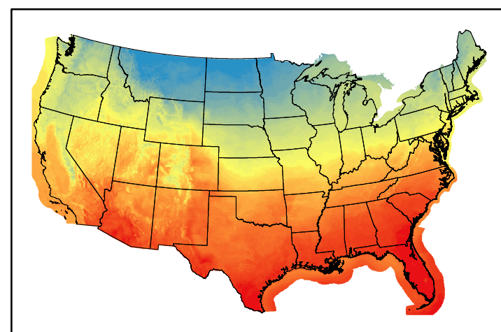
Dry Bulb Temp temp20250204.bil
