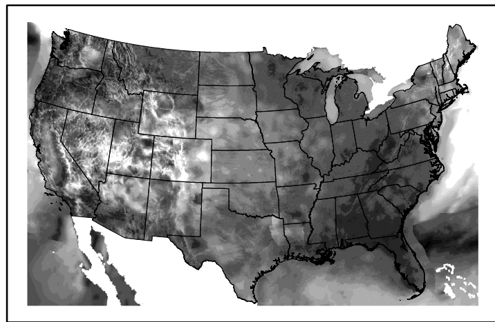
Wind Speed wspd20250204.bil
