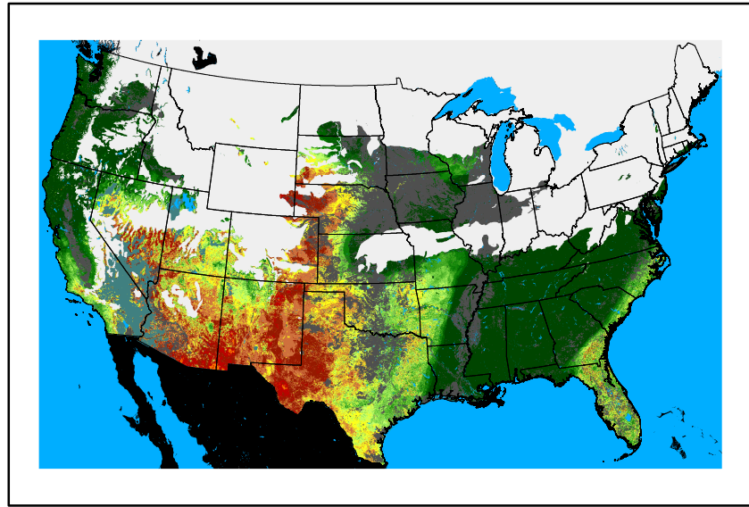
WFPI fp250131.bil
