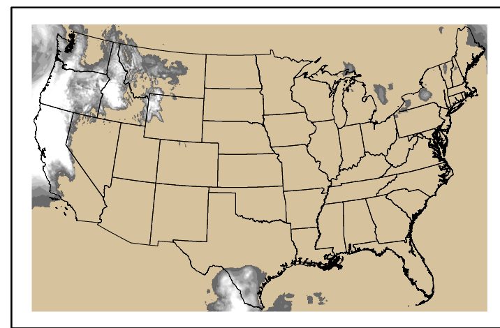
Precipitation p24m_2025012900f168.bil
