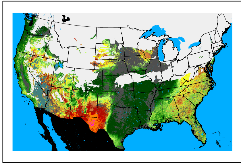
WFPI fp250130.bil
