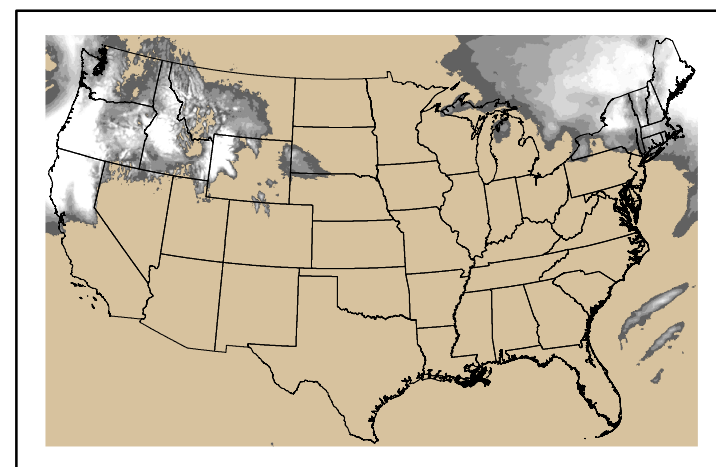
Precipitation p24m_2025012900f144.bil
