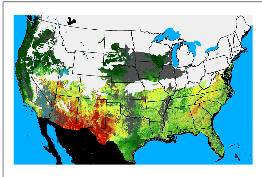
WFPI fp250203.bil
