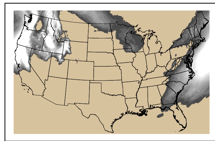
Precipitation p24m_2025012900f096.bil
