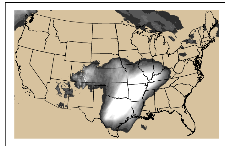
Precipitation p24m_2025012900f048.bil
