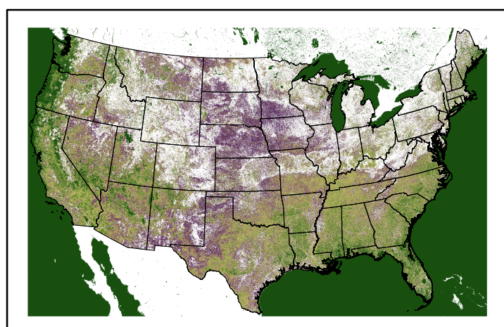
Greenness us25_020026wk_greenness.img
