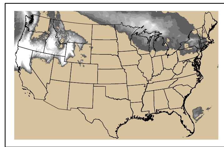
Precipitation p24m_2025012900f120.bil
