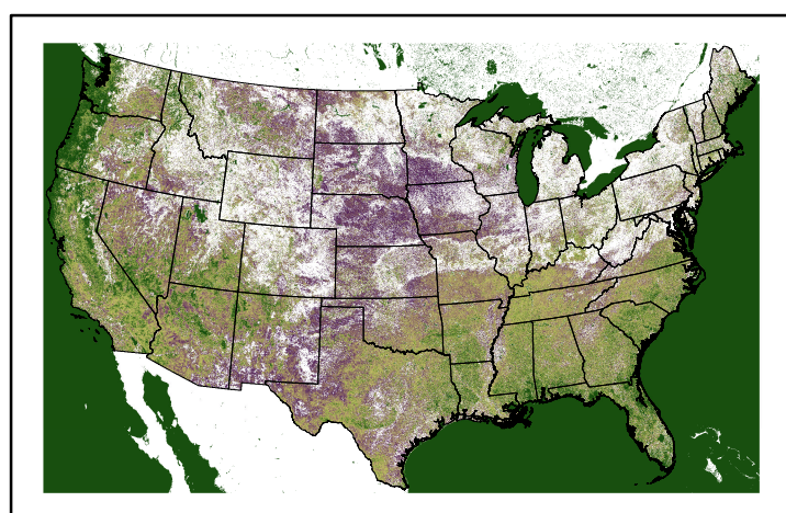
Greenness us25_020026wk_greenness.img
