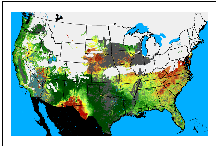
WFPI fp250129.bil
