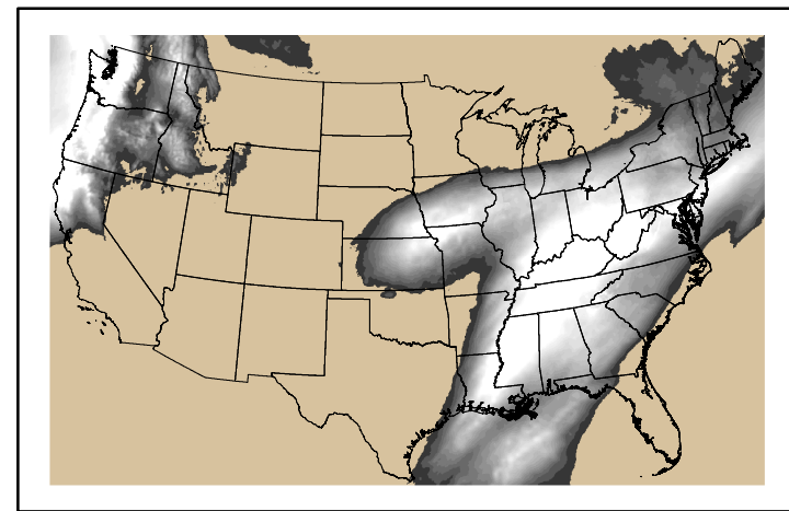
Precipitation p24m_2025012900f072.bil
