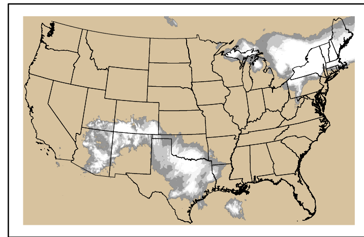
Precipitation p24m_2025012900f024.bil
