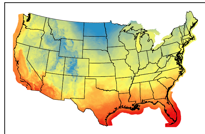
Dry Bulb Temp temp20250112.bil
