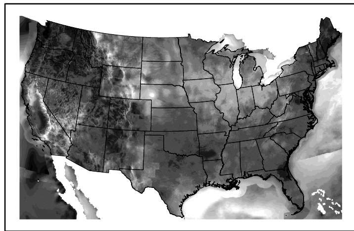
Wind Speed wspd20250113.bil
