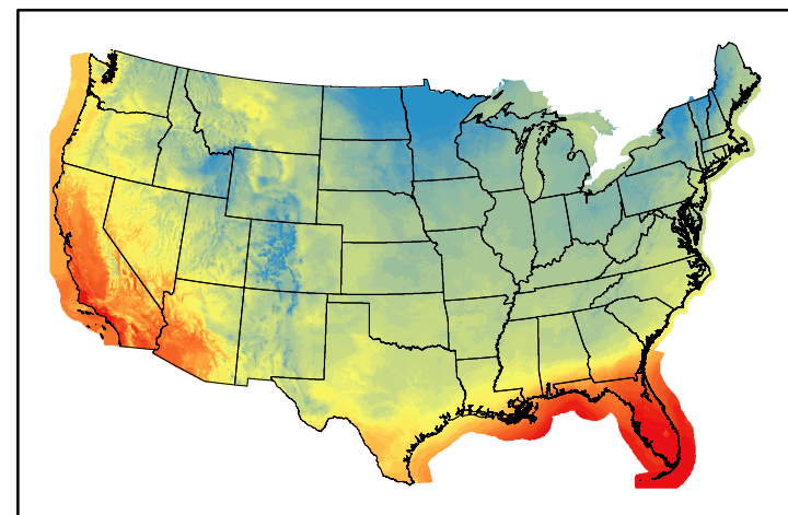
Dry Bulb Temp temp20250110.bil
