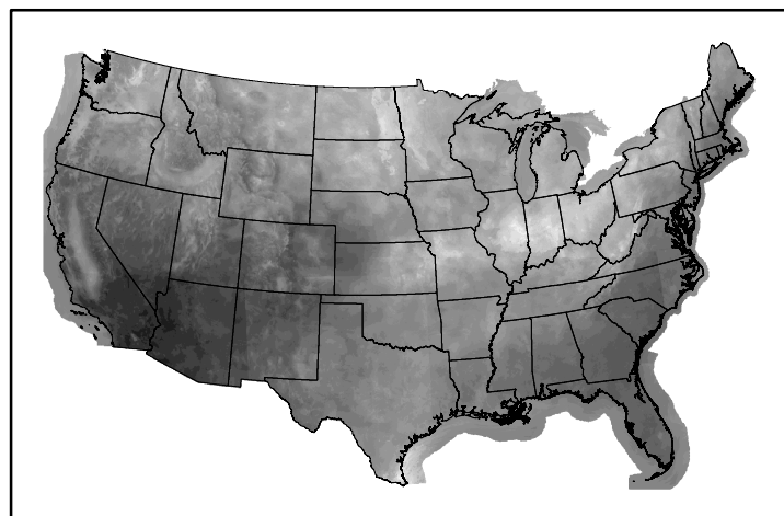
10hr Fuel Moisture mc10250115.bil
