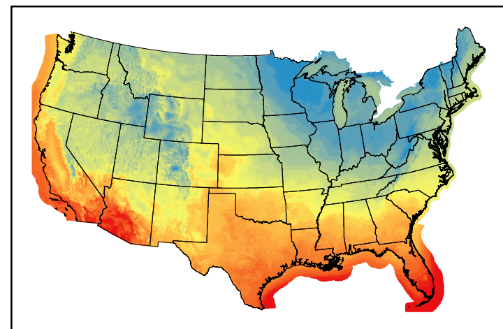
Dry Bulb Temp temp20250115.bil
