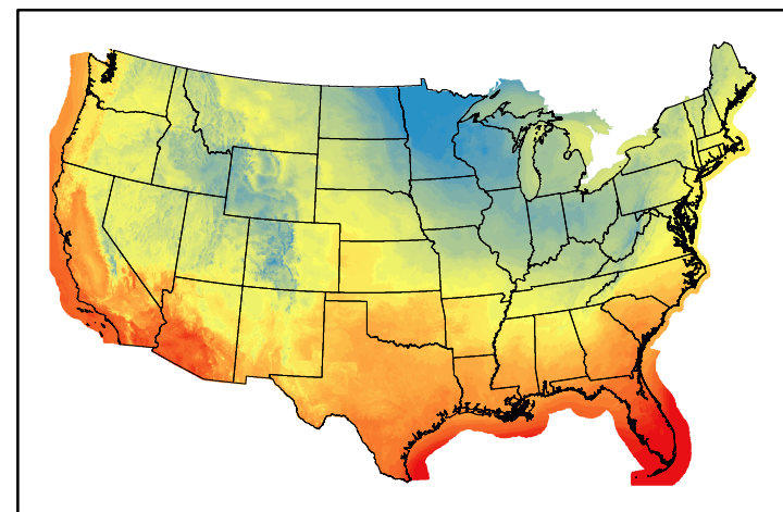
Dry Bulb Temp temp20250114.bil
