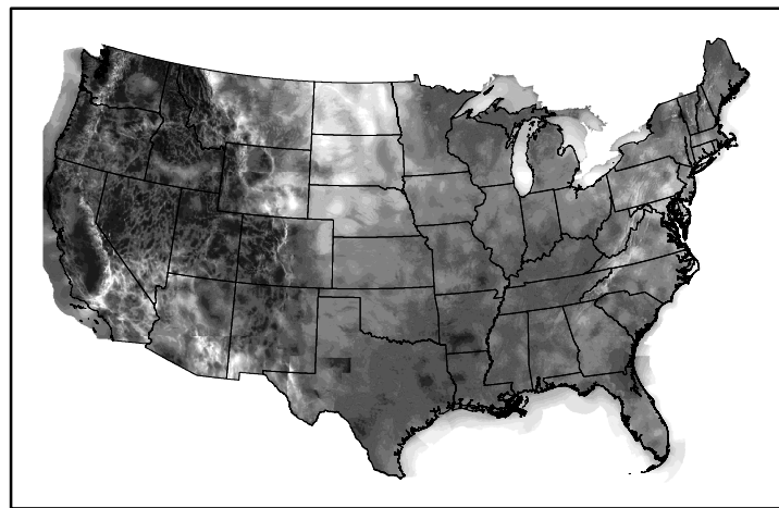
Wind Speed wspd20250115.bil
