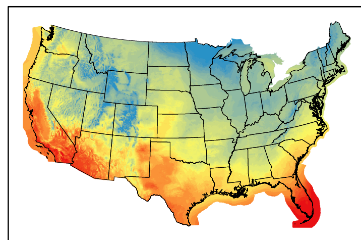
Dry Bulb Temp temp20250111.bil
