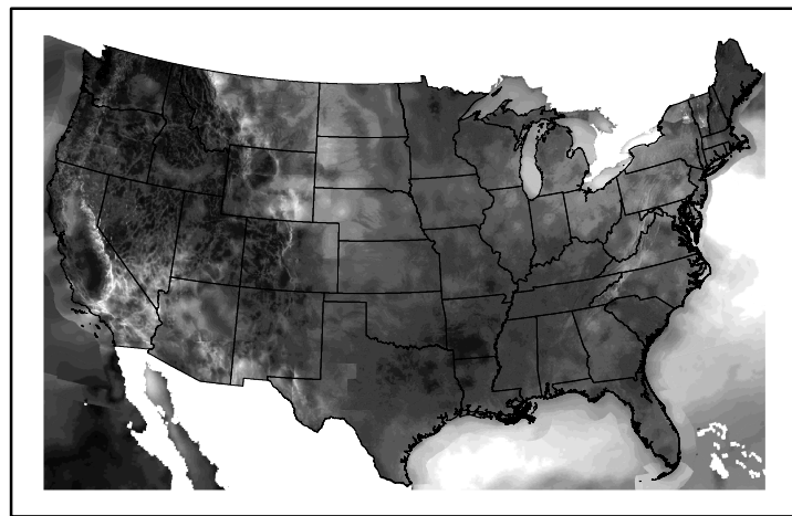
Wind Speed wspd20250114.bil
