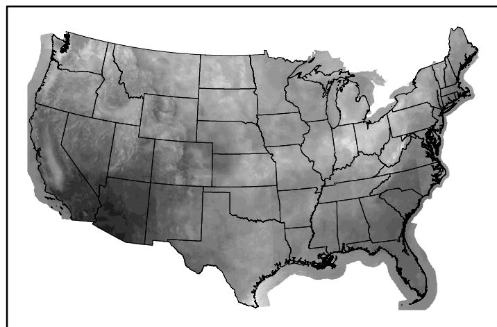
10hr Fuel Moisture mc10250114.bil
