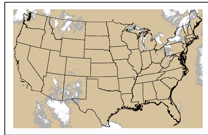
Precipitation p24m_2025010800f024.bil
