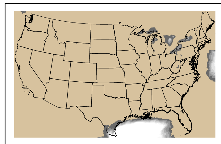
Precipitation p24m_2025010800f168.bil
