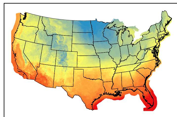
Dry Bulb Temp temp20250114.bil
