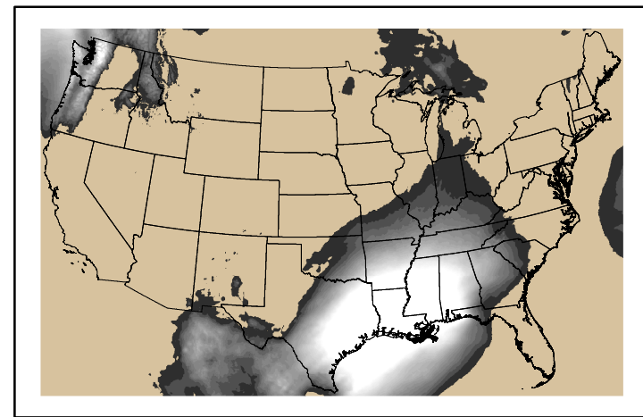
Precipitation p24m_2025010800f072.bil
