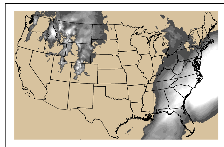
Precipitation p24m_2025010800f096.bil
