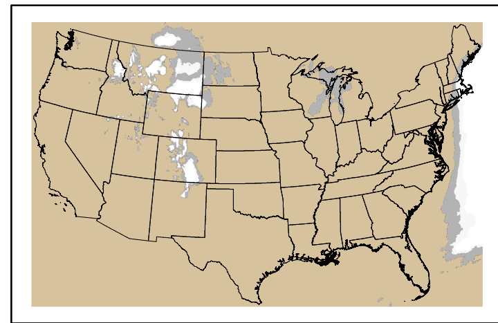
Precipitation p24m_2025010800f120.bil
