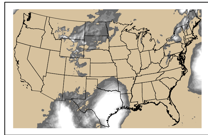
Precipitation p24m_2025010800f048.bil
