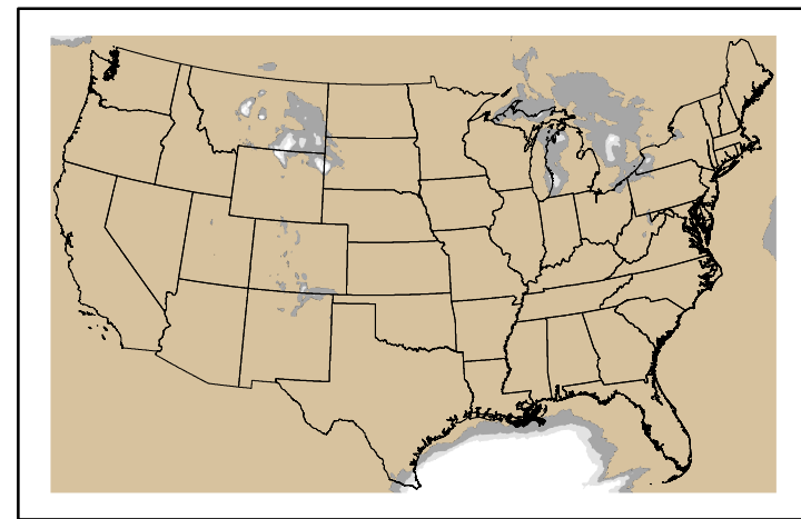
Precipitation p24m_2025010800f144.bil
