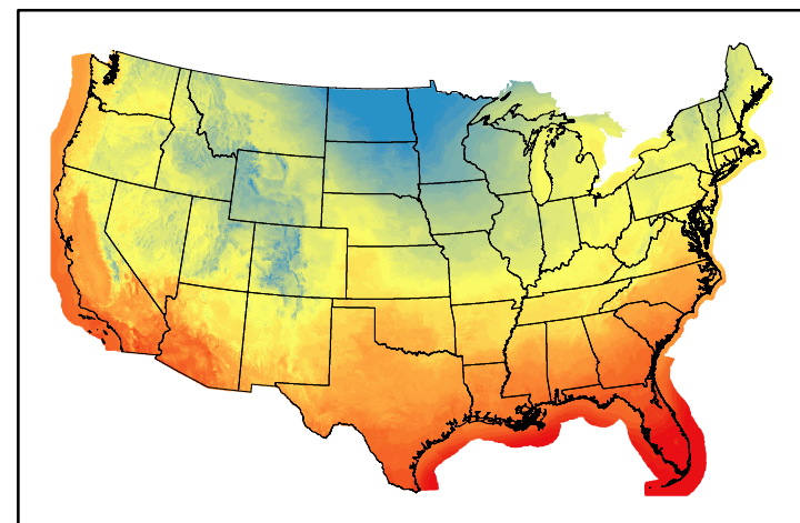
Dry Bulb Temp temp20250113.bil
