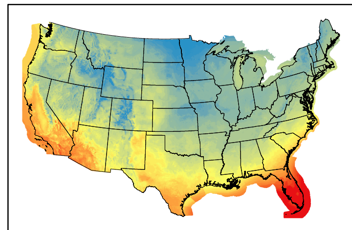
Dry Bulb Temp temp20250111.bil
