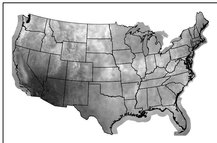
10hr Fuel Moisture mc10250111.bil
