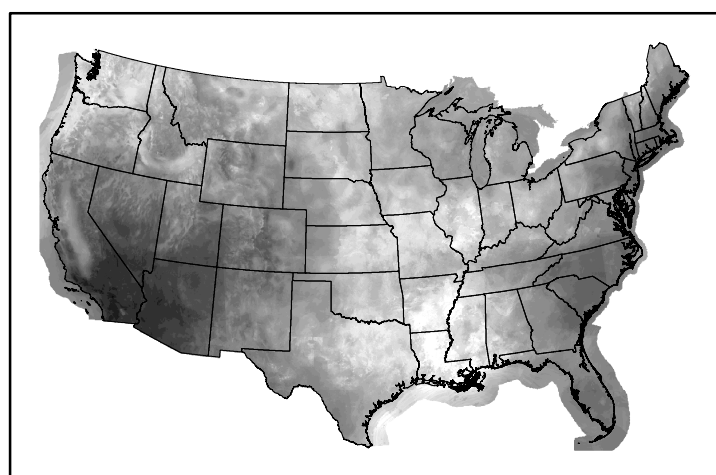
10hr Fuel Moisture mc10250110.bil
