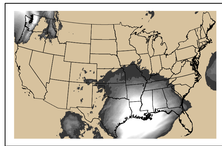
Precipitation p24m_2025010700f096.bil
