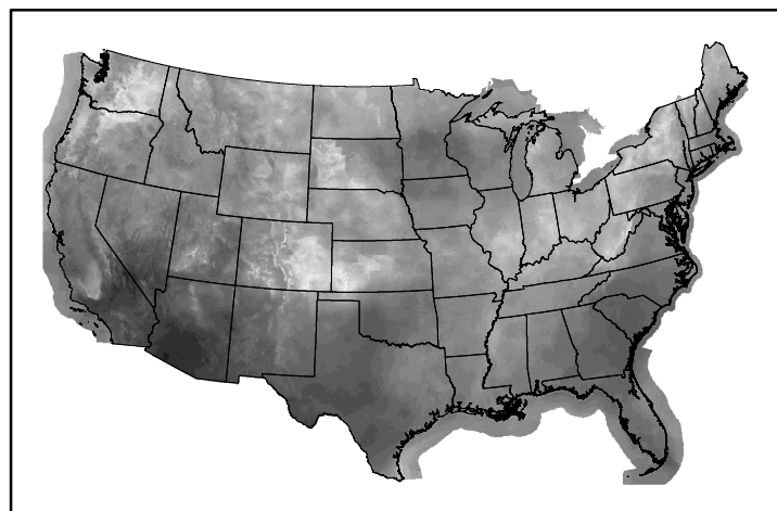
10hr Fuel Moisture mc10250107.bil
