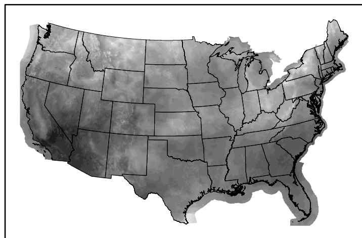
10hr Fuel Moisture mc10250108.bil
