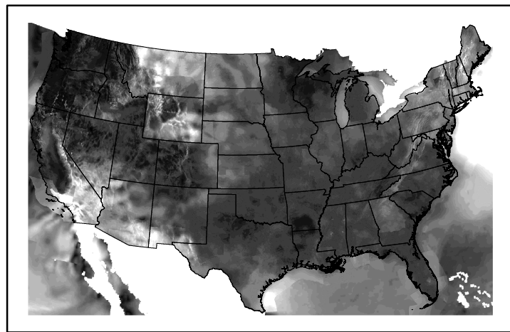
Wind Speed wspd20250108.bil
