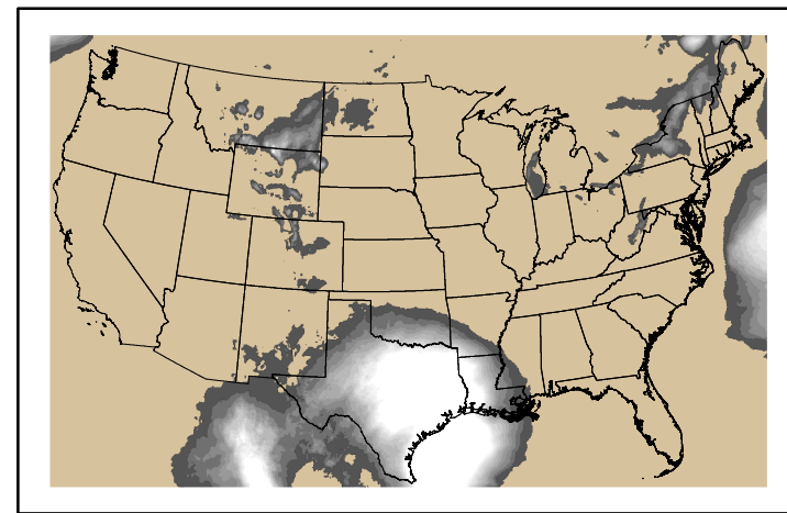
Precipitation p24m_2025010700f072.bil
