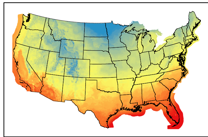
Dry Bulb Temp temp20250113.bil
