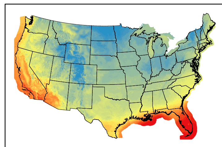
Dry Bulb Temp temp20250110.bil
