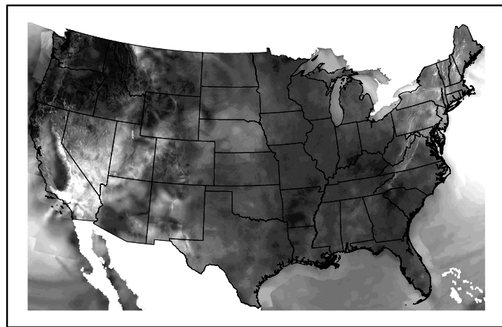
Wind Speed wspd20250107.bil
