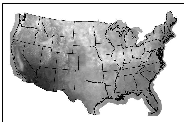
10hr Fuel Moisture mc10250112.bil
