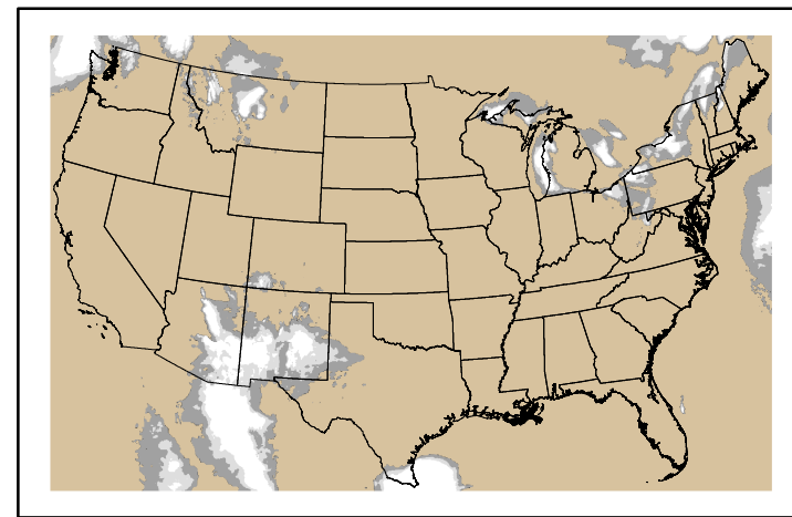
Precipitation p24m_2025010700f048.bil
