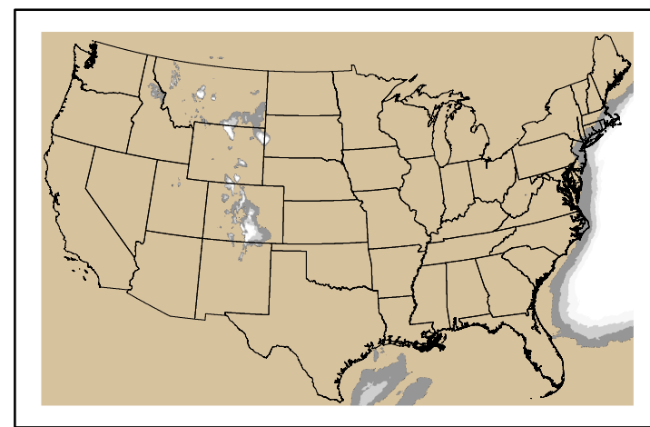
Precipitation p24m_2025010700f144.bil
