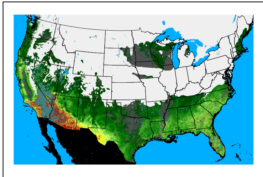
WFPI fp250112.bil
