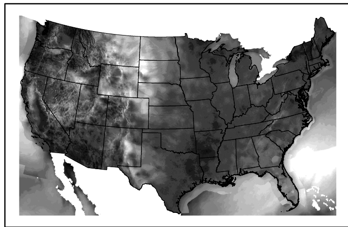
Wind Speed wspd20250111.bil
