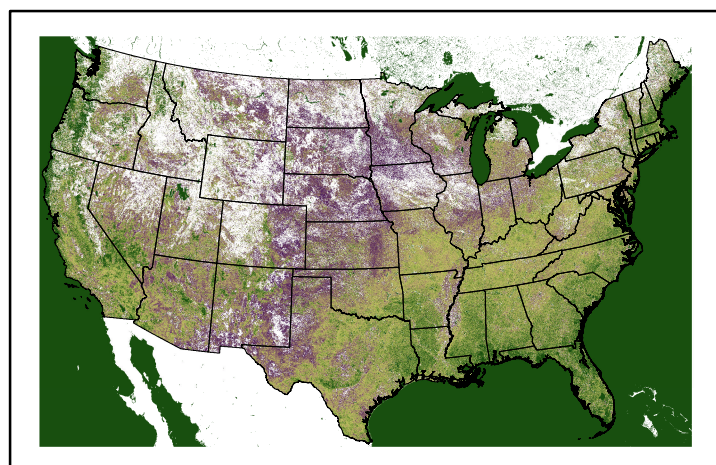
Greenness us25_365005wk_greenness.img
