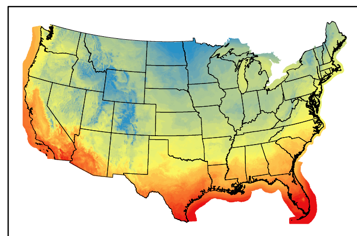
Dry Bulb Temp temp20250112.bil
