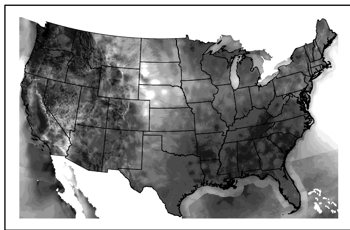
Wind Speed wspd20250112.bil
