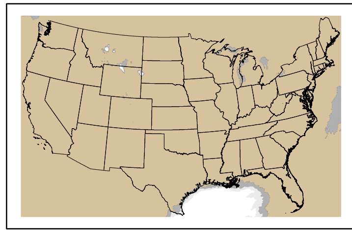
Precipitation p24m_2025010700f168.bil
