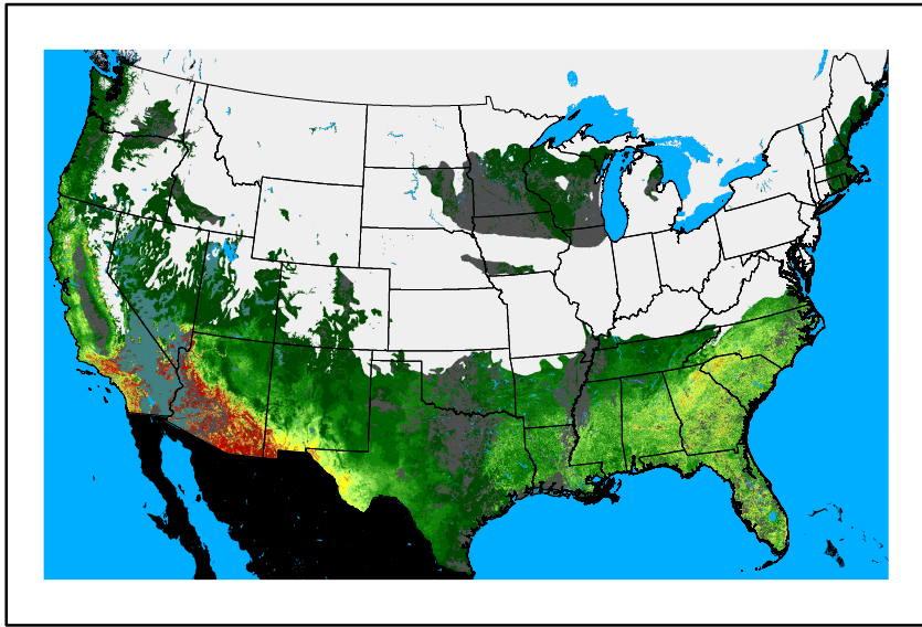
WFPI fp250113.bil
