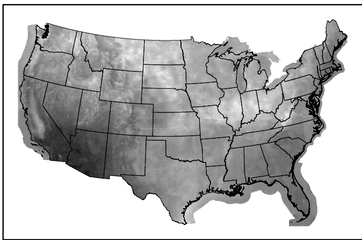
10hr Fuel Moisture mc10250113.bil
