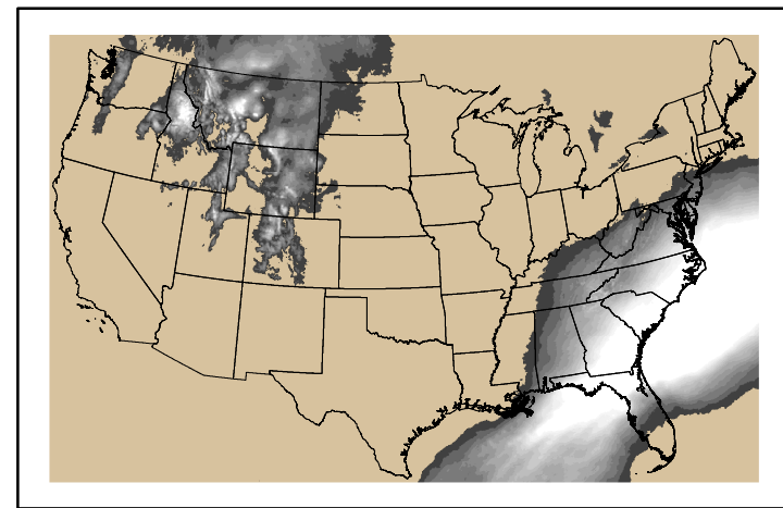
Precipitation p24m_2025010700f120.bil
