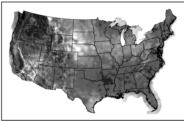
Wind Speed wspd20250113.bil
