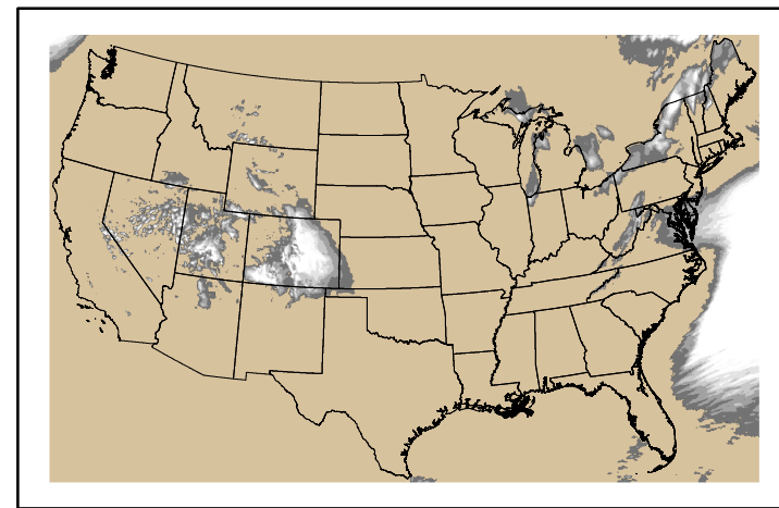
Precipitation p24m_2025010700f024.bil
