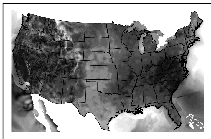
Wind Speed wspd20250110.bil
