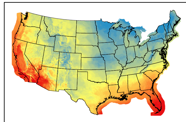
Dry Bulb Temp temp20250108.bil
