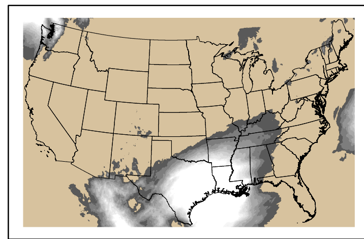
Precipitation p24m_2025010500f144.bil
