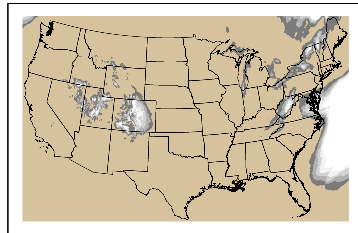
Precipitation p24m_2025010500f072.bil
