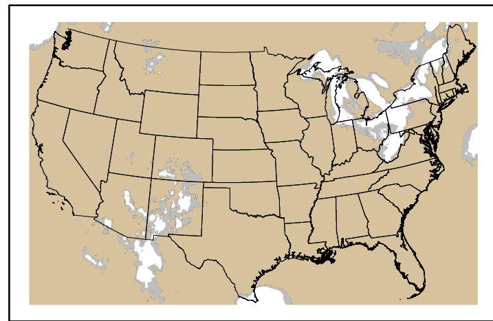
Precipitation p24m_2025010500f096.bil
