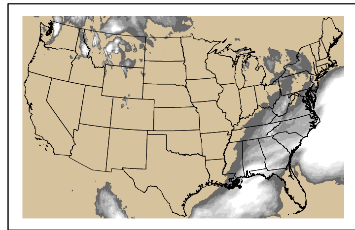
Precipitation p24m_2025010500f168.bil
