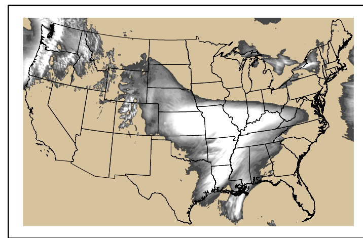
Precipitation p24m_2025010500f024.bil
