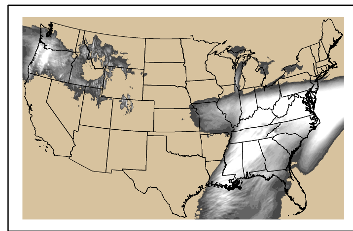
Precipitation p24m_2025010500f048.bil
