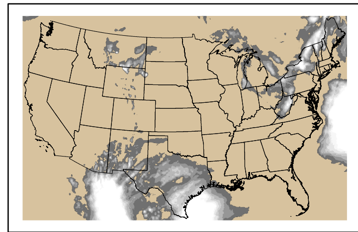
Precipitation p24m_2025010500f120.bil
