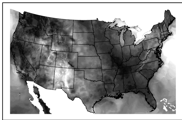
Wind Speed wspd20250104.bil
