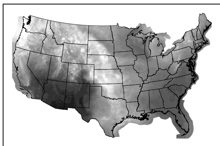
10hr Fuel Moisture mc10250104.bil
