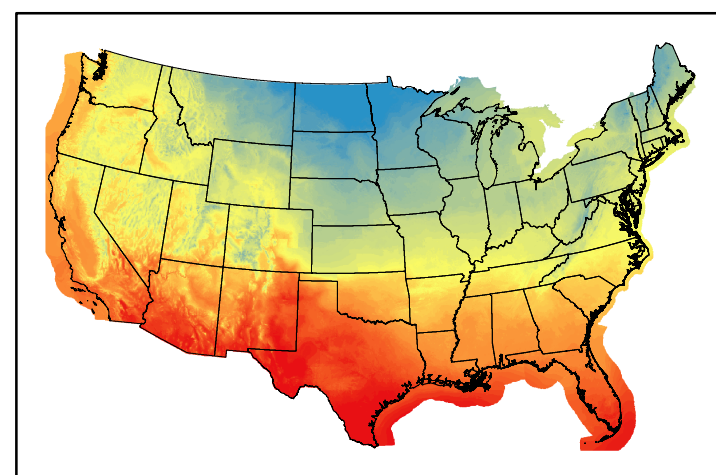
Dry Bulb Temp temp20250104.bil
