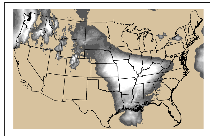
Precipitation p24m_2025010200f096.bil
