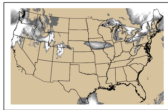
Precipitation p24m_2025010200f024.bil
