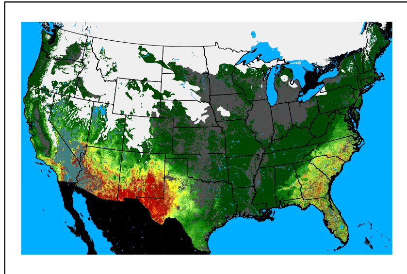
WFPI fp250105.bil
