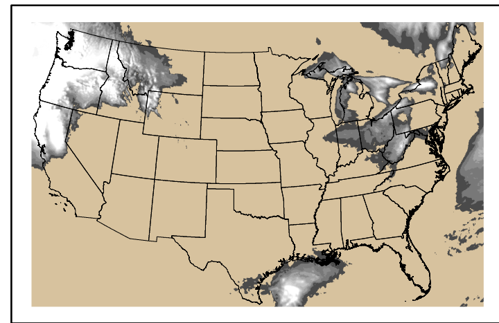
Precipitation p24m_2025010200f048.bil
