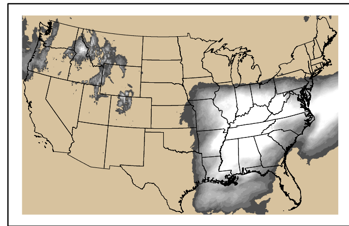
Precipitation p24m_2025010200f120.bil
