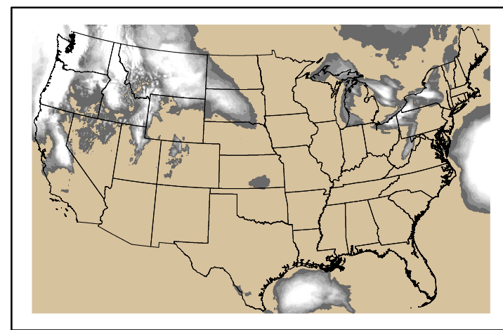
Precipitation p24m_2025010200f072.bil
