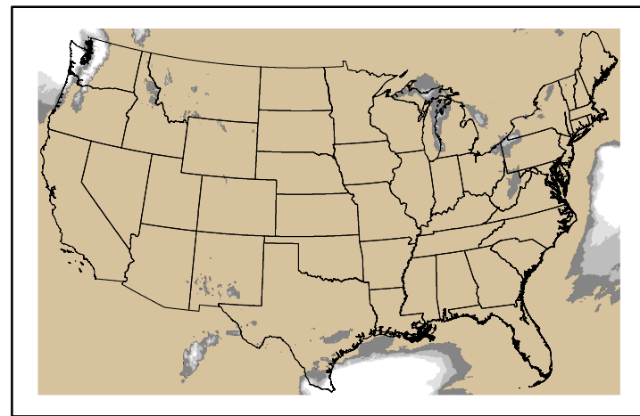
Precipitation p24m_2025010200f168.bil
