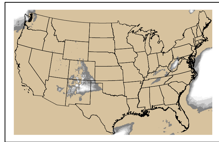
Precipitation p24m_2025010200f144.bil
