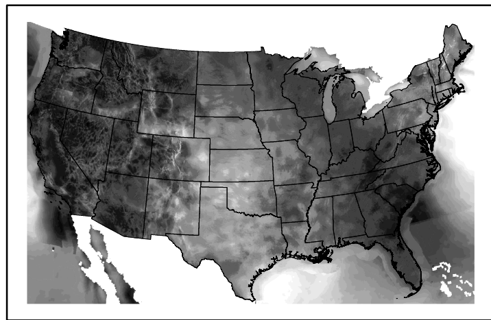
Wind Speed wspd20250105.bil
