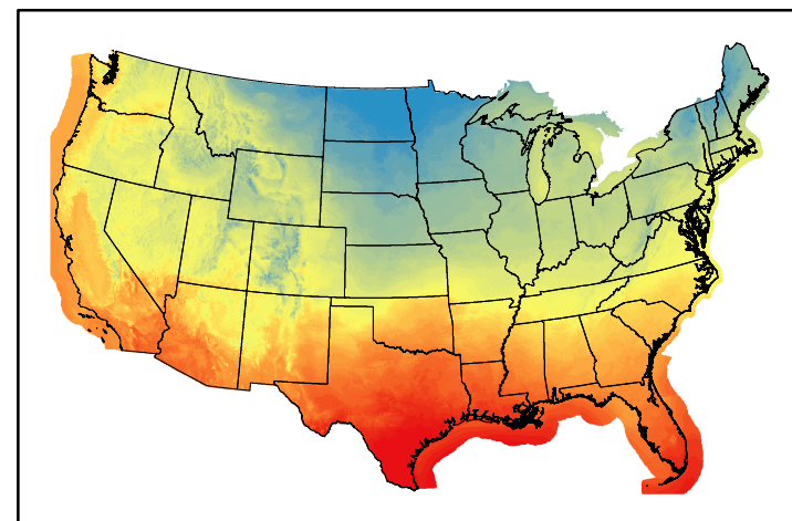
Dry Bulb Temp temp20250105.bil
