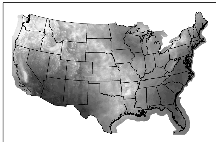
10hr Fuel Moisture mc10250105.bil
