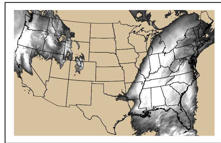
Precipitation p24m_2024122900f024.bil
