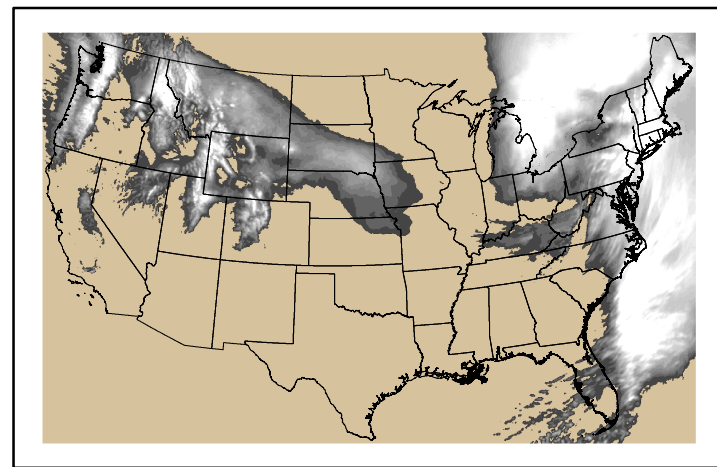
Precipitation p24m_2024122900f048.bil
