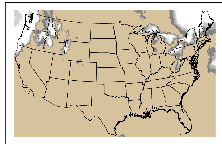
Precipitation p24m_2024122900f120.bil
