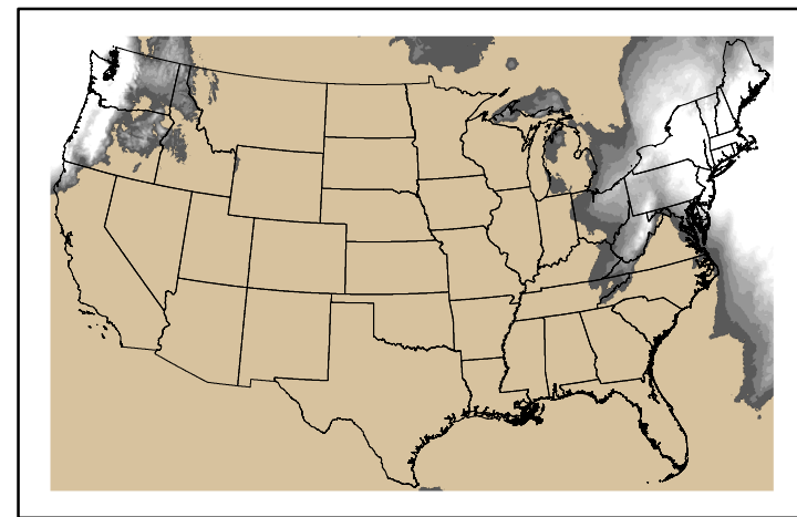
Precipitation p24m_2024122900f096.bil
