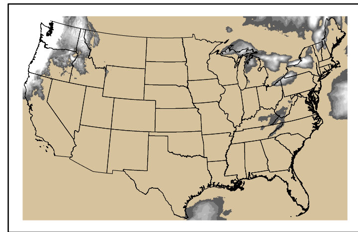
Precipitation p24m_2024122900f144.bil
