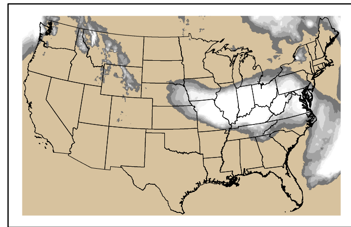
Precipitation p24m_2024122900f072.bil
