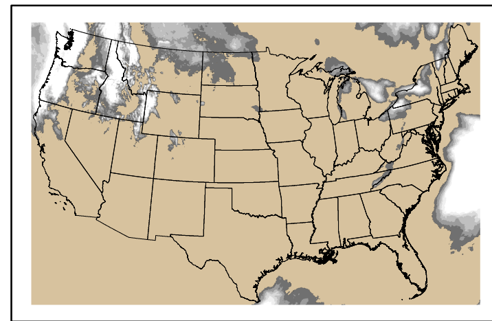
Precipitation p24m_2024122900f168.bil
