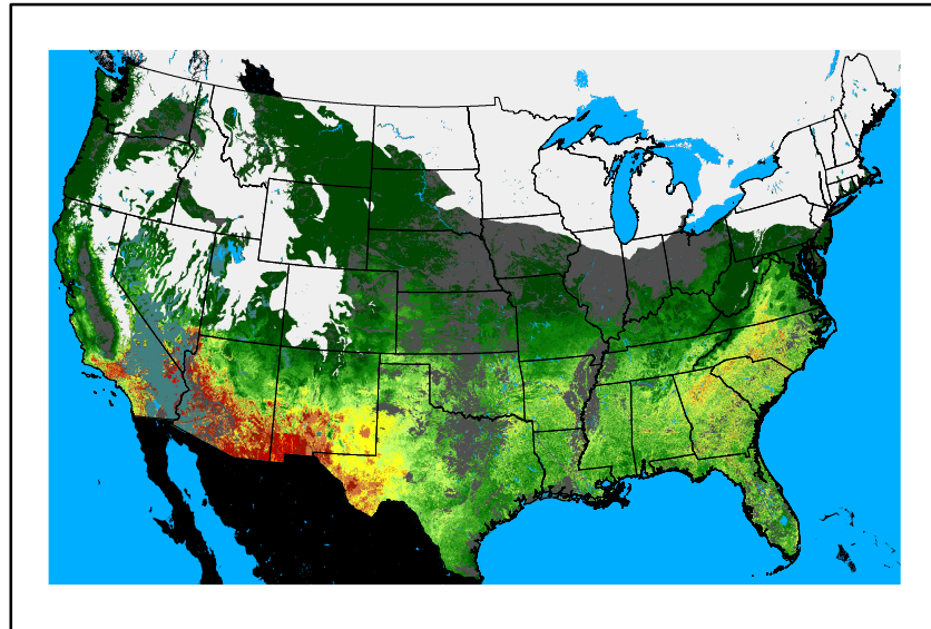
WFPI fp250101.bil
