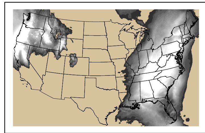
Precipitation p24m_2024122700f072.bil
