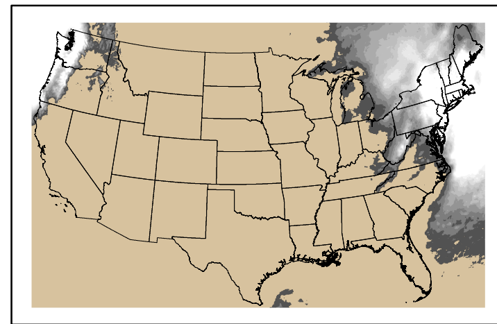
Precipitation p24m_2024122700f144.bil
