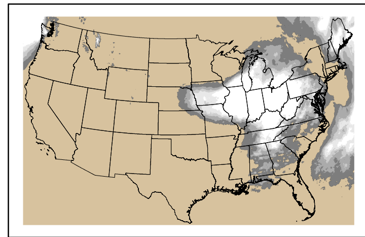
Precipitation p24m_2024122700f120.bil
