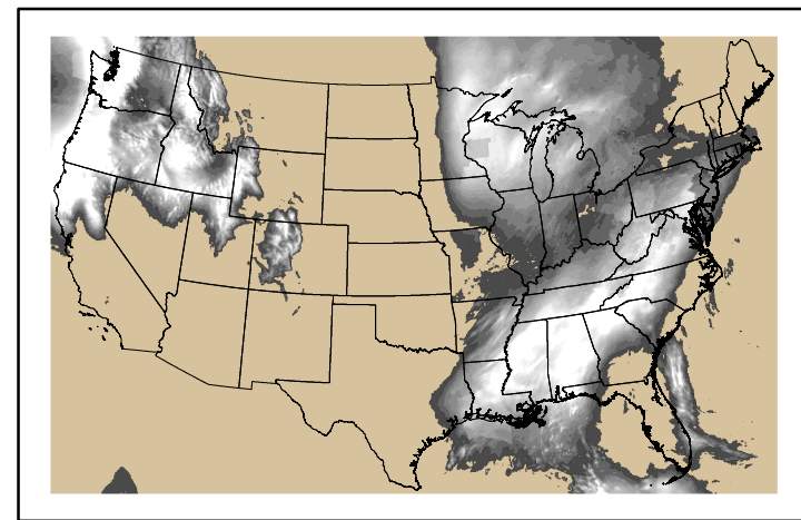
Precipitation p24m_2024122700f048.bil
