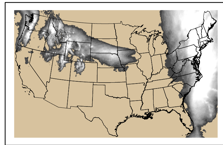
Precipitation p24m_2024122700f096.bil
