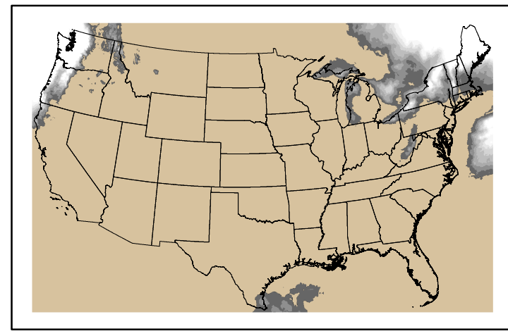
Precipitation p24m_2024122700f168.bil
