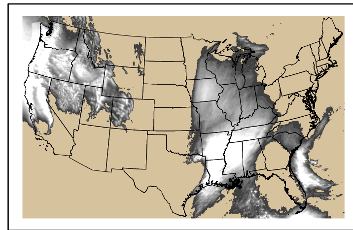
Precipitation p24m_2024122700f024.bil
