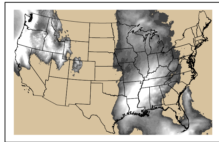
Precipitation p24m_2024122500f096.bil
