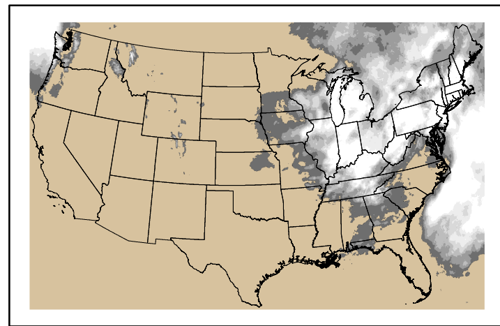
Precipitation p24m_2024122500f168.bil
