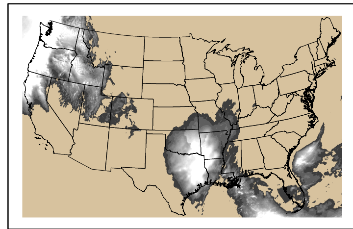
Precipitation p24m_2024122500f048.bil
