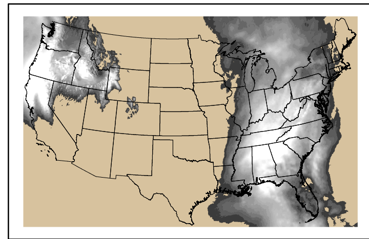
Precipitation p24m_2024122500f120.bil
