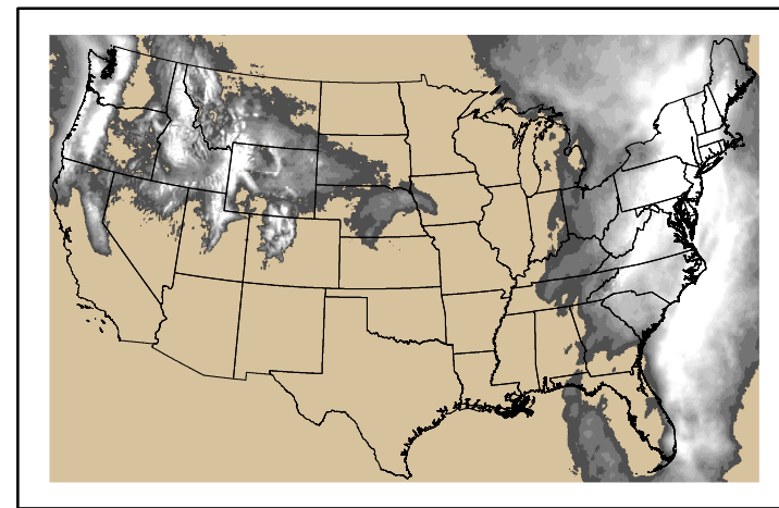
Precipitation p24m_2024122500f144.bil
