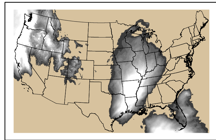
Precipitation p24m_2024122500f072.bil
