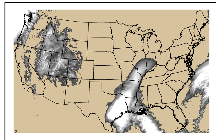
Precipitation p24m_2024122500f024.bil
