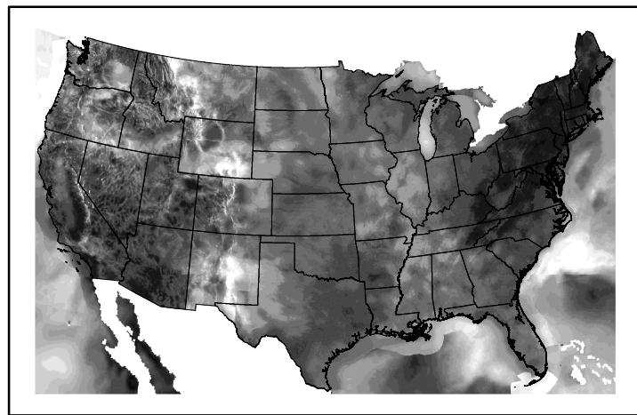
Wind Speed wspd20241227.bil
