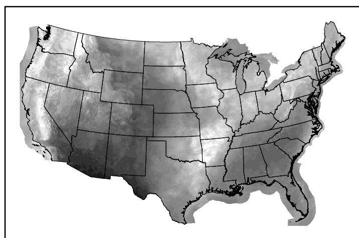
10hr Fuel Moisture mc10241224.bil
