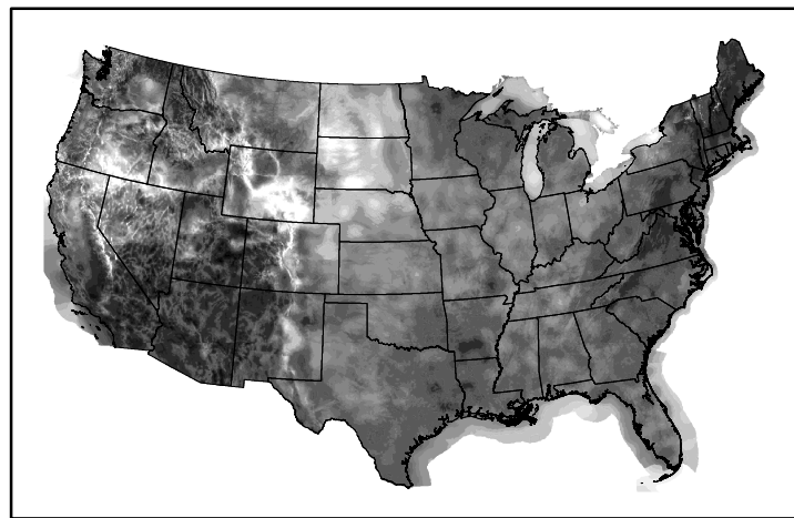
Wind Speed wspd20241229.bil
