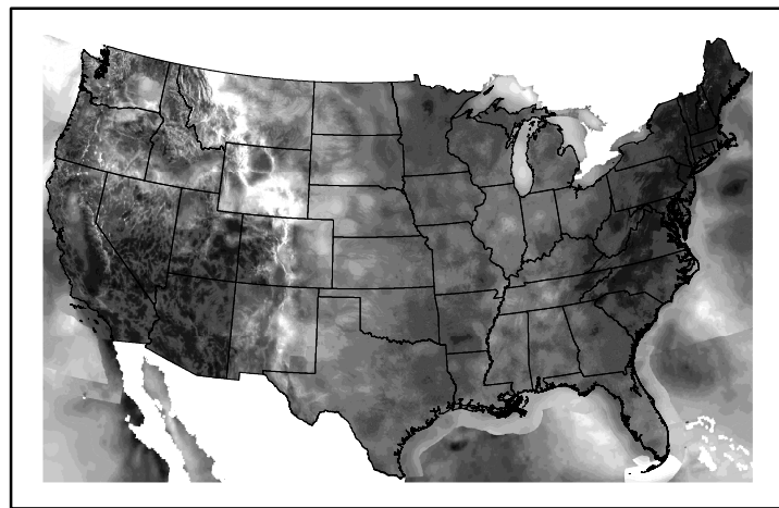
Wind Speed wspd20241228.bil
