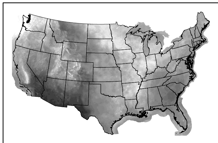
10hr Fuel Moisture mc10241225.bil
