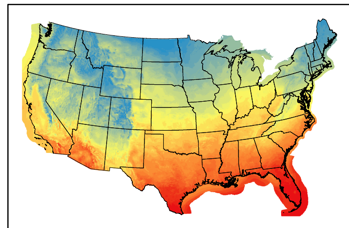
Dry Bulb Temp temp20241229.bil
