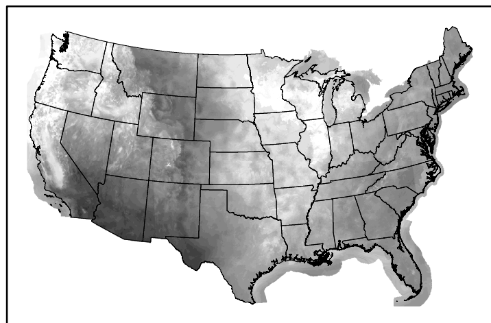
10hr Fuel Moisture mc10241227.bil
