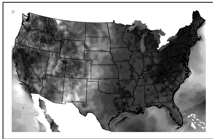
Wind Speed wspd20241225.bil
