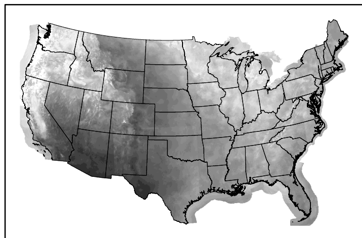
10hr Fuel Moisture mc10241229.bil
