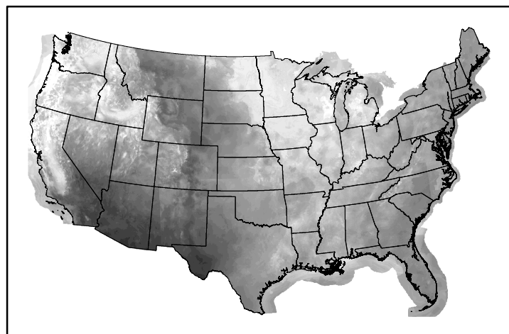
10hr Fuel Moisture mc10241228.bil
