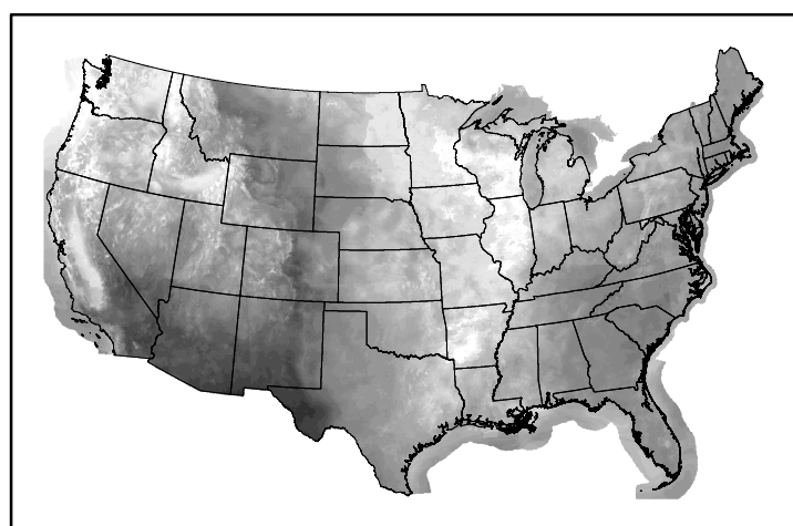
10hr Fuel Moisture mc10241226.bil
