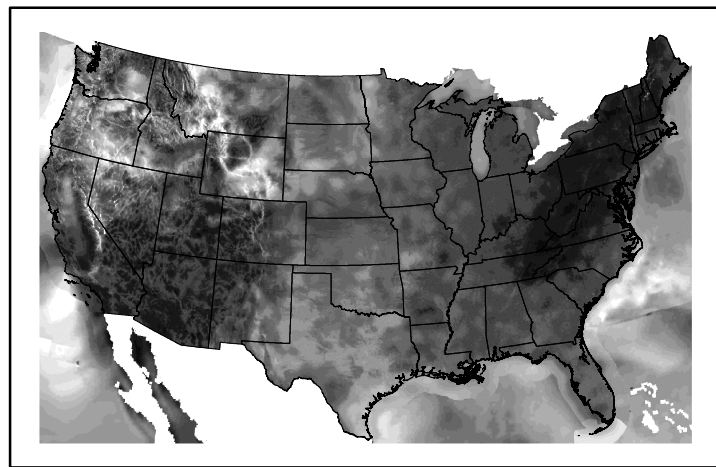
Wind Speed wspd20241226.bil
