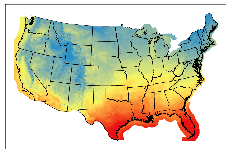
Dry Bulb Temp temp20241226.bil
