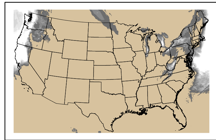
Precipitation p24m_2024122000f048.bil
