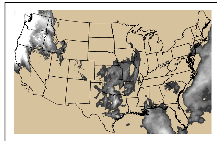
Precipitation p24m_2024122000f168.bil
