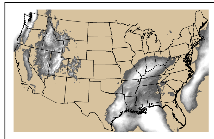
Precipitation p24m_2024122000f144.bil
