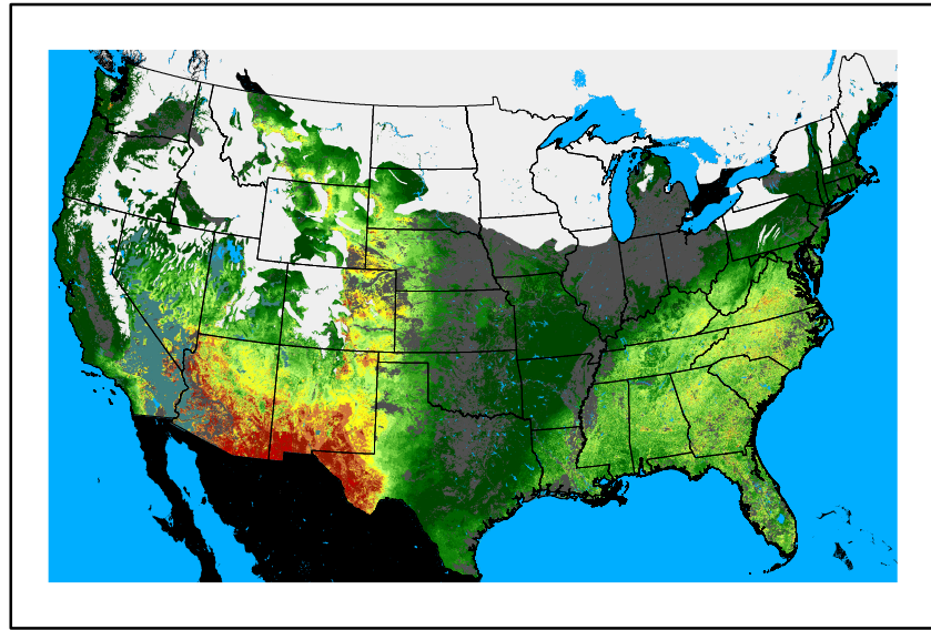
WFPI fp241224.bil
