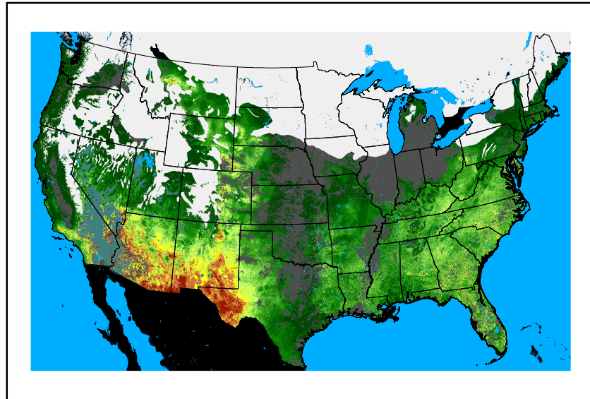
WFPI fp241226.bil
