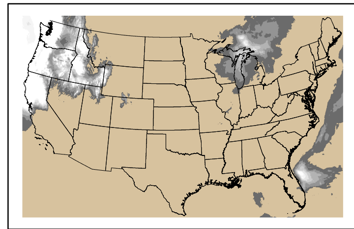
Precipitation p24m_2024122000f096.bil
