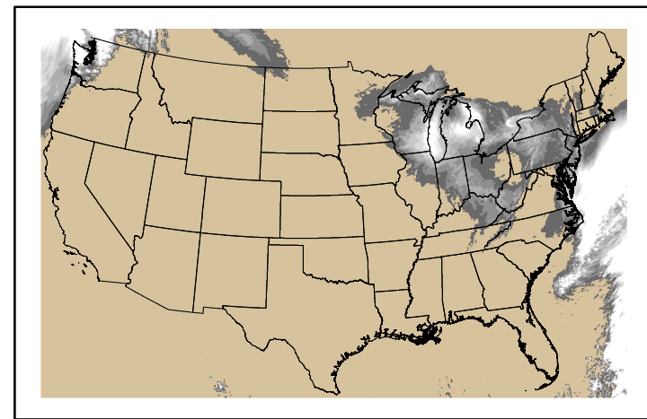
Precipitation p24m_2024122000f024.bil
