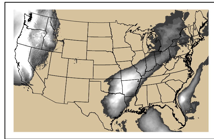
Precipitation p24m_2024122000f120.bil
