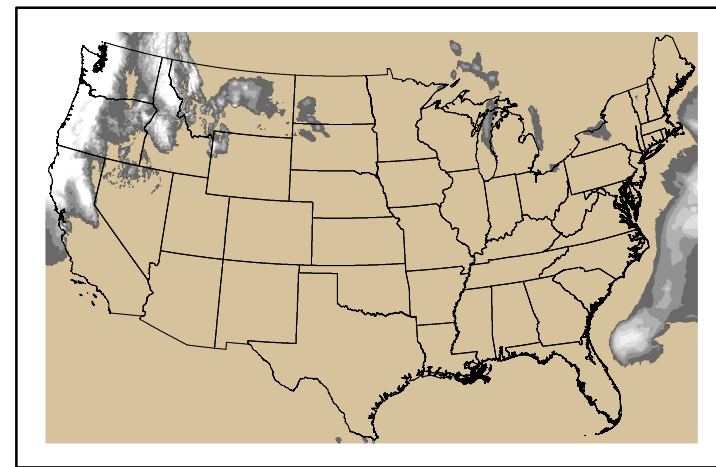
Precipitation p24m_2024122000f072.bil
