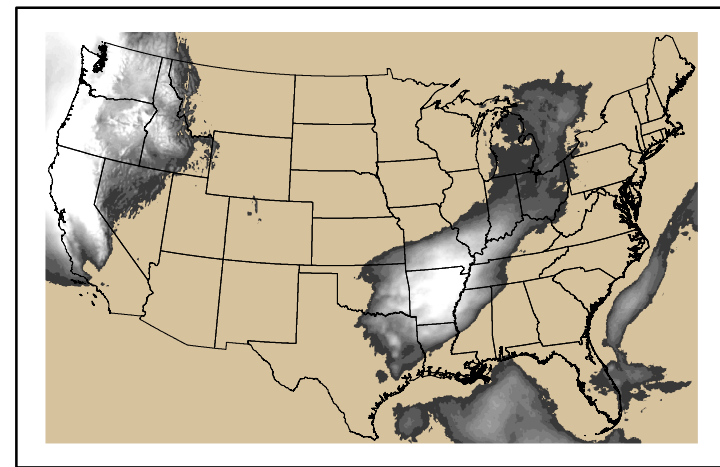
Precipitation p24m_2024121900f144.bil
