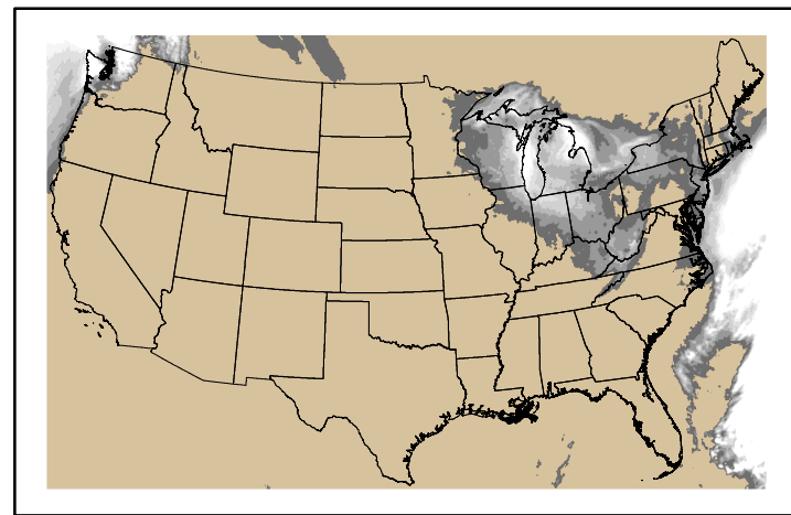
Precipitation p24m_2024121900f048.bil
