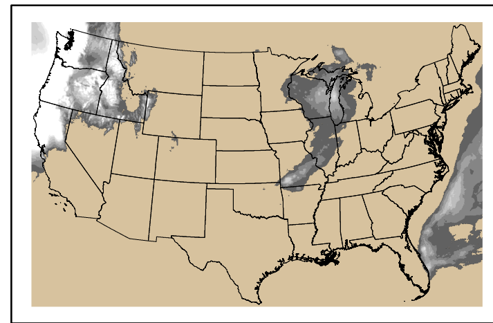
Precipitation p24m_2024121900f120.bil
