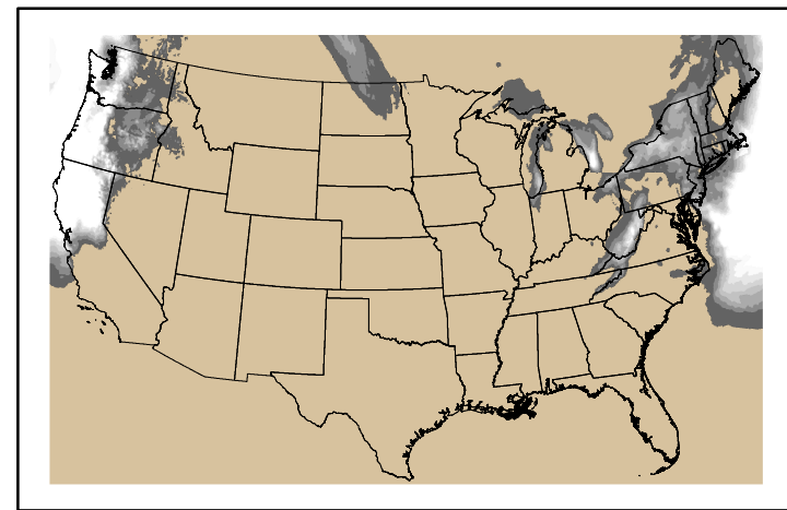
Precipitation p24m_2024121900f072.bil
