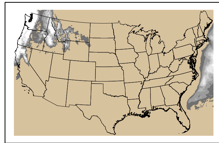
Precipitation p24m_2024121900f096.bil
