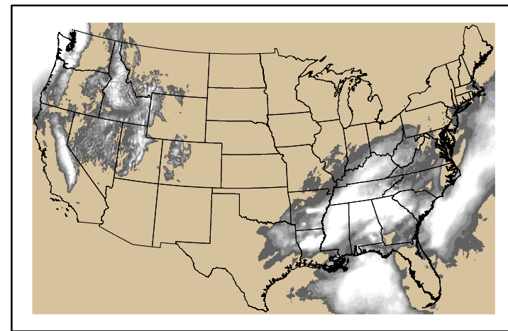
Precipitation p24m_2024121900f168.bil
