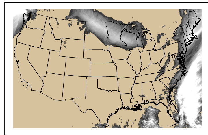
Precipitation p24m_2024121900f024.bil
