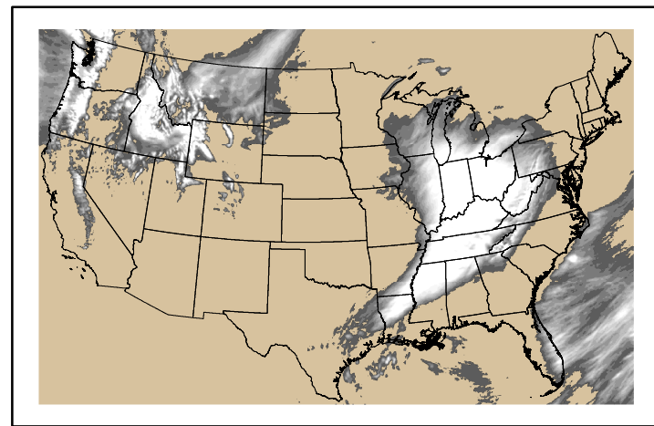
Precipitation p24m_2024121500f024.bil
