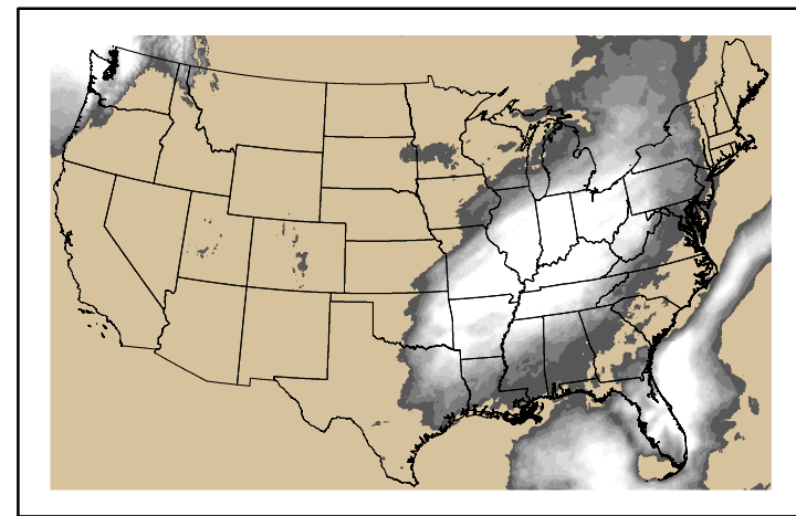
Precipitation p24m_2024121500f096.bil
