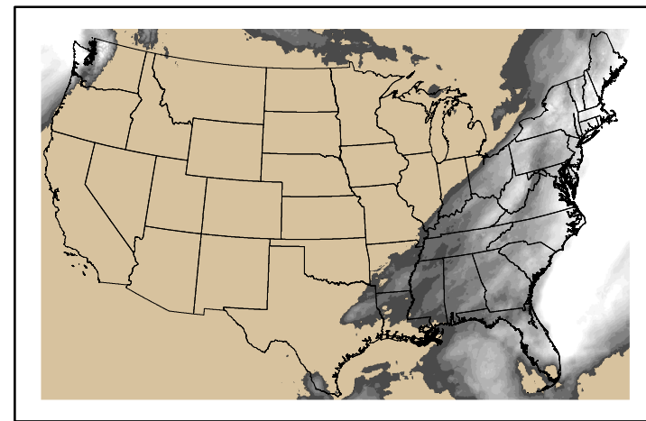
Precipitation p24m_2024121500f120.bil
