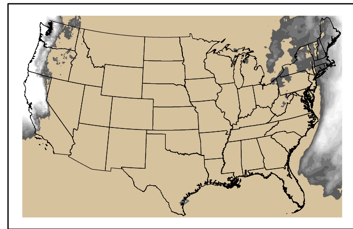
Precipitation p24m_2024121500f168.bil
