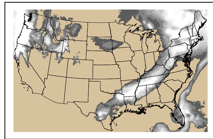
Precipitation p24m_2024121500f072.bil
