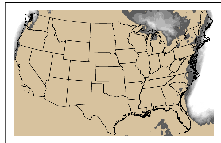
Precipitation p24m_2024121500f144.bil
