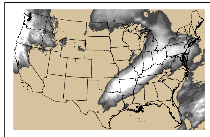
Precipitation p24m_2024121500f048.bil
