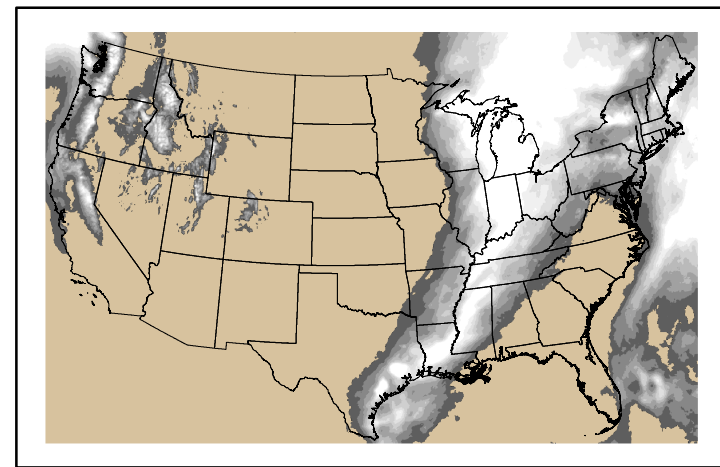
Precipitation p24m_2024121200f144.bil
