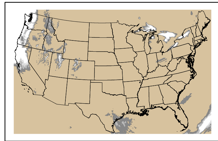
Precipitation p24m_2024121200f048.bil
