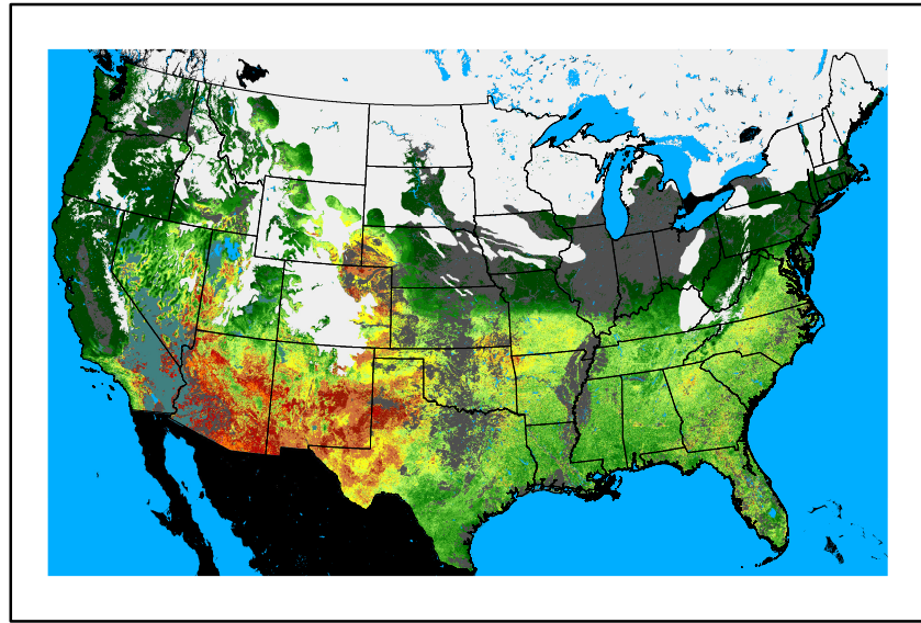
WFPI fp241212.bil
