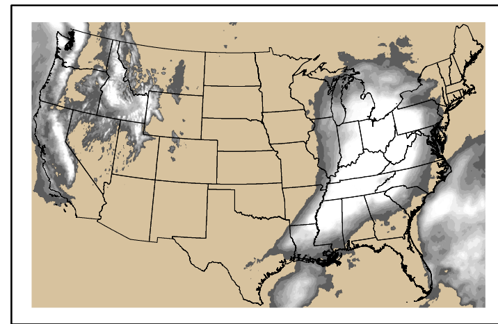
Precipitation p24m_2024121200f096.bil
