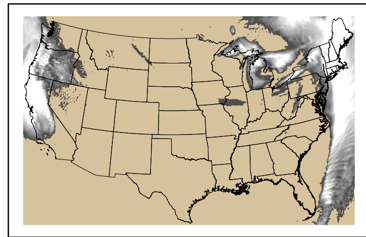
Precipitation p24m_2024121200f024.bil
