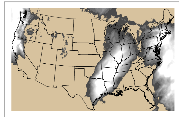
Precipitation p24m_2024121200f120.bil
