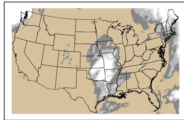
Precipitation p24m_2024121200f168.bil
