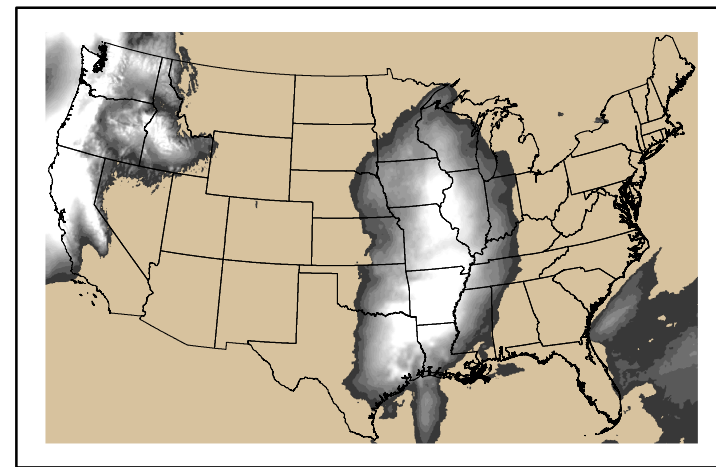
Precipitation p24m_2024121200f072.bil
