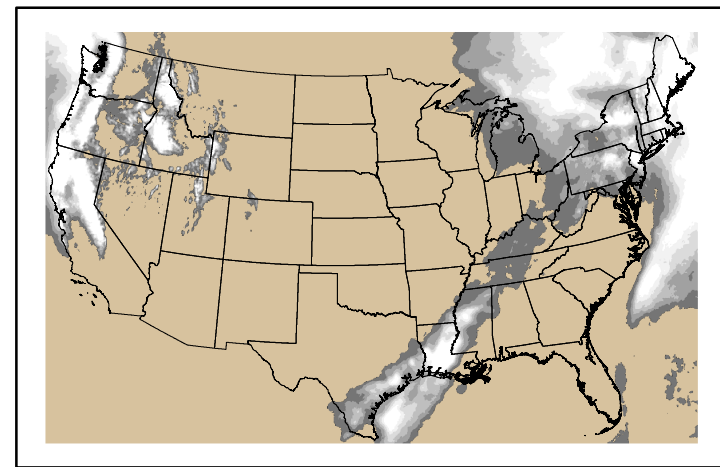
Precipitation p24m_2024121100f168.bil
