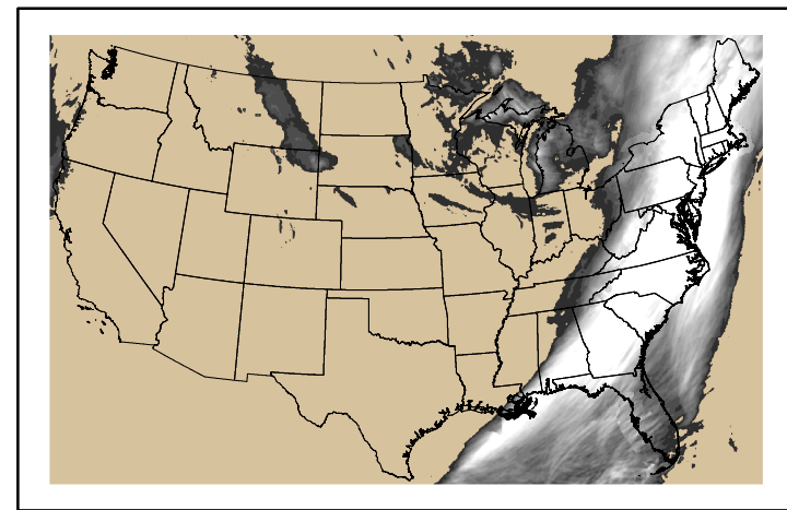
Precipitation p24m_2024121100f024.bil
