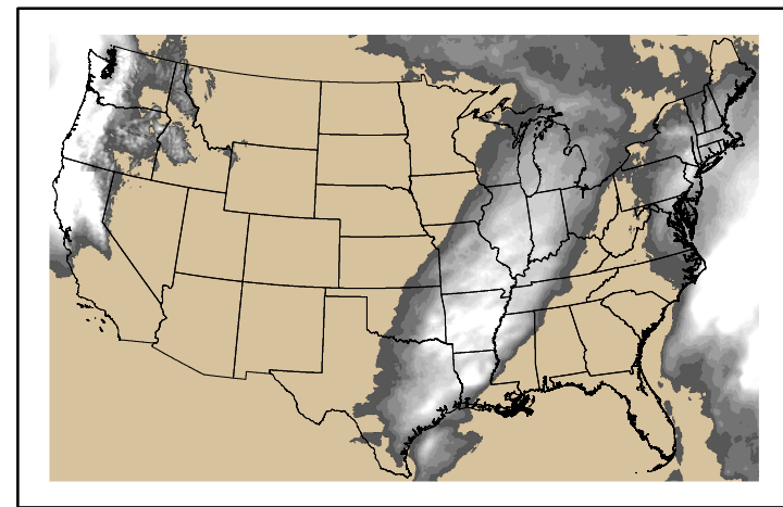
Precipitation p24m_2024121100f144.bil
