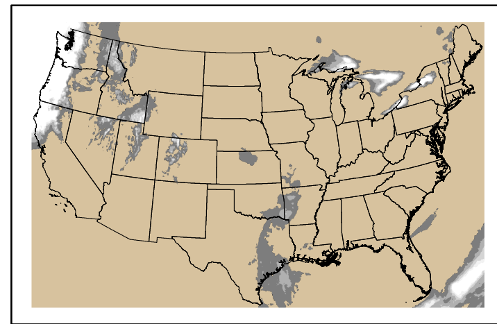
Precipitation p24m_2024121100f072.bil
