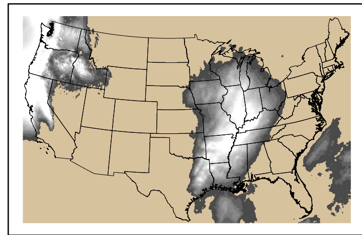
Precipitation p24m_2024121100f096.bil
