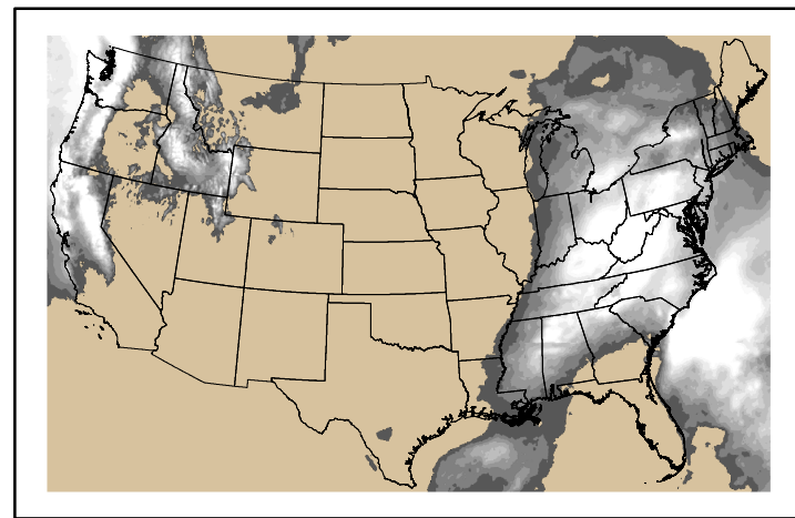
Precipitation p24m_2024121100f120.bil
