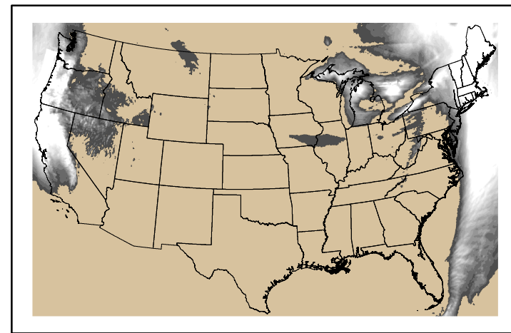
Precipitation p24m_2024121100f048.bil
