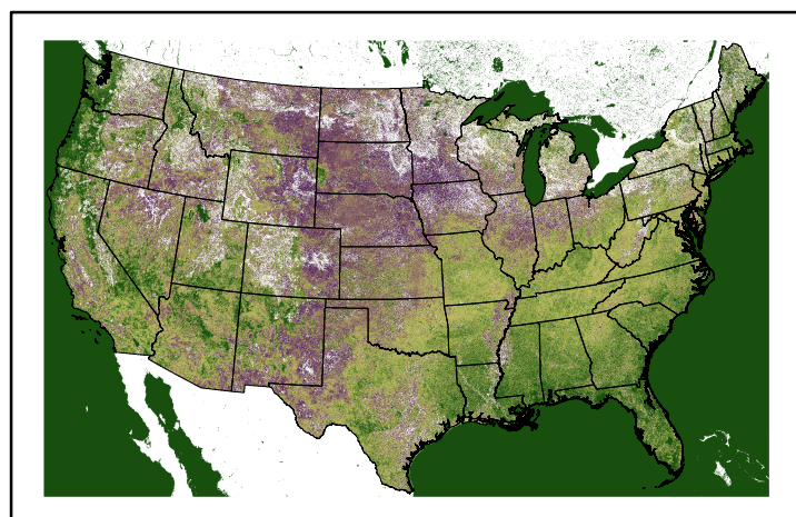
Greenness us24_337343wk_greenness.img
