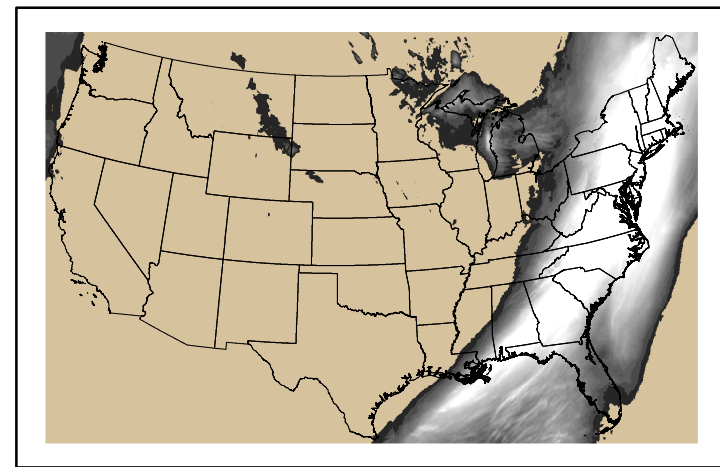
Precipitation p24m_2024121000f048.bil
