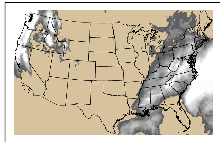
Precipitation p24m_2024121000f144.bil
