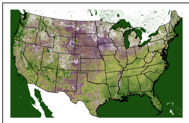
Greenness us24_337343wk_greenness.img
