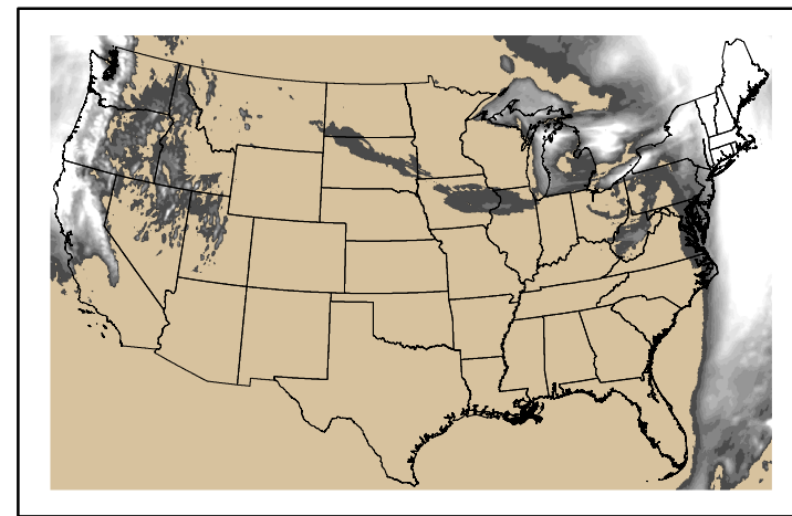
Precipitation p24m_2024121000f072.bil
