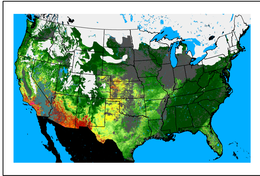
WFPI fp241210.bil
