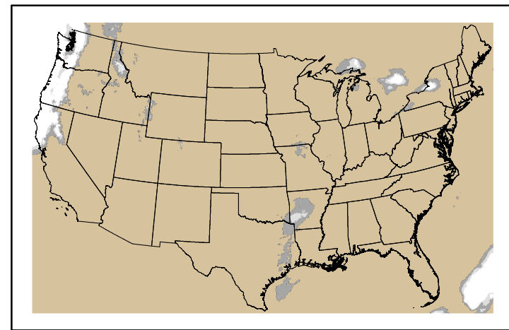
Precipitation p24m_2024121000f096.bil
