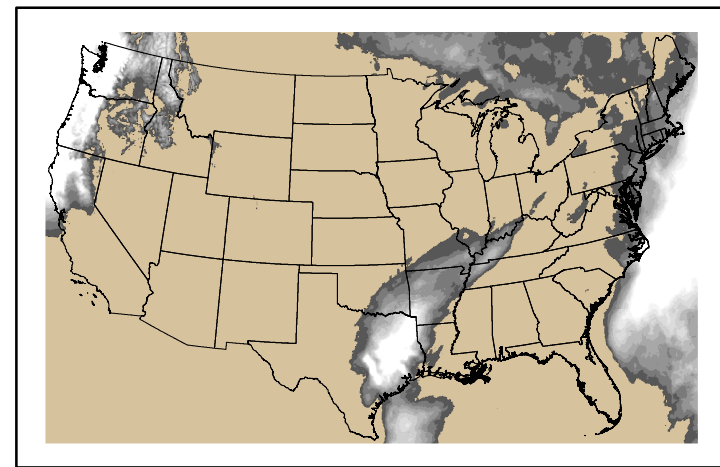
Precipitation p24m_2024121000f168.bil
