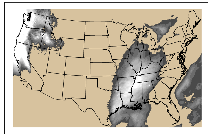
Precipitation p24m_2024121000f120.bil
