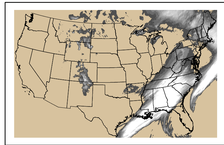
Precipitation p24m_2024121000f024.bil
