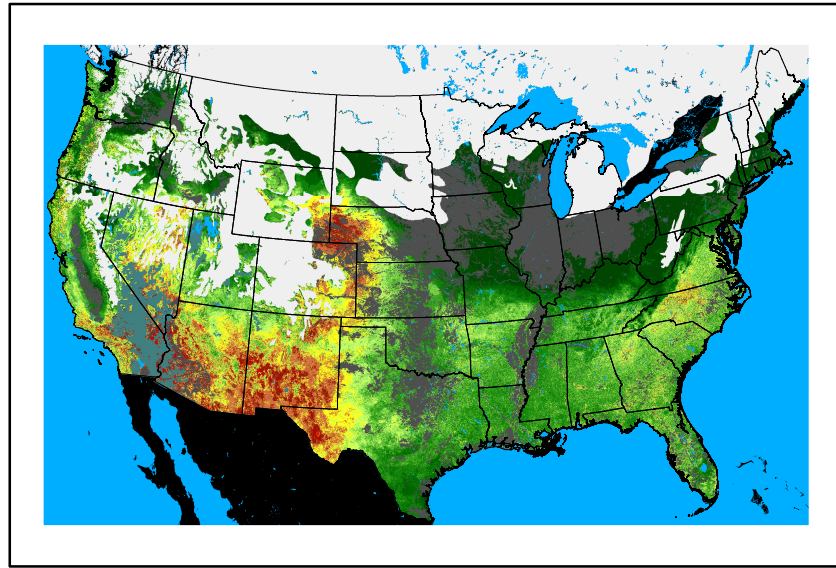
WFPI fp241201.bil
