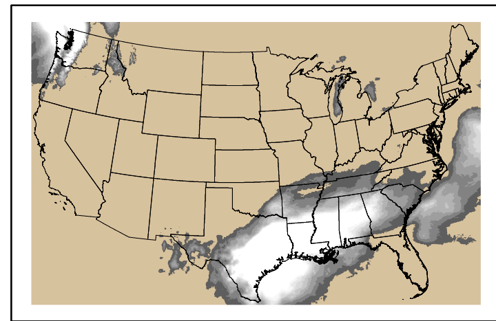
Precipitation p24m_2024120100f168.bil
