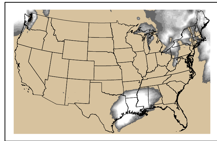
Precipitation p24m_2024120100f120.bil
