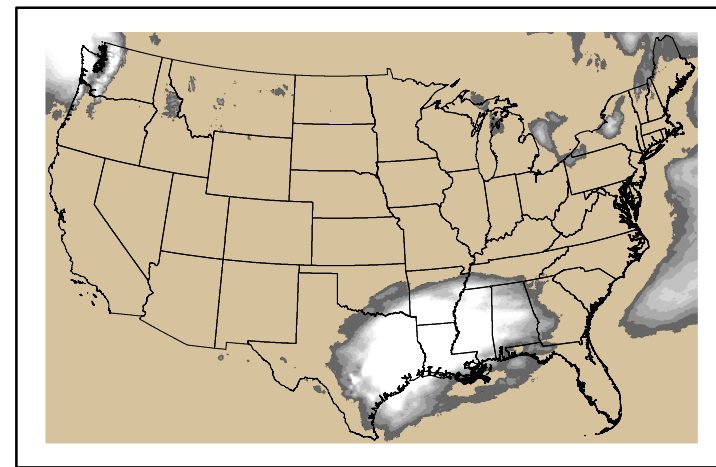
Precipitation p24m_2024120100f144.bil
