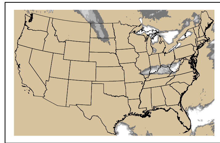
Precipitation p24m_2024120100f024.bil
