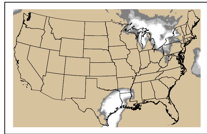
Precipitation p24m_2024120100f096.bil
