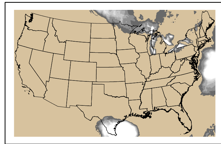
Precipitation p24m_2024120100f072.bil
