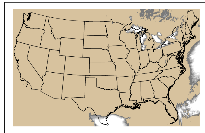
Precipitation p24m_2024120100f048.bil
