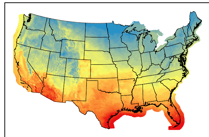
Dry Bulb Temp temp20241204.bil
