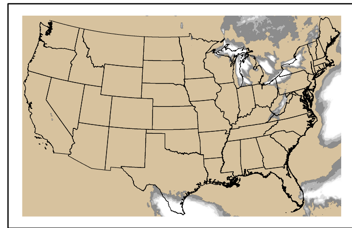
Precipitation p24m_2024113000f072.bil
