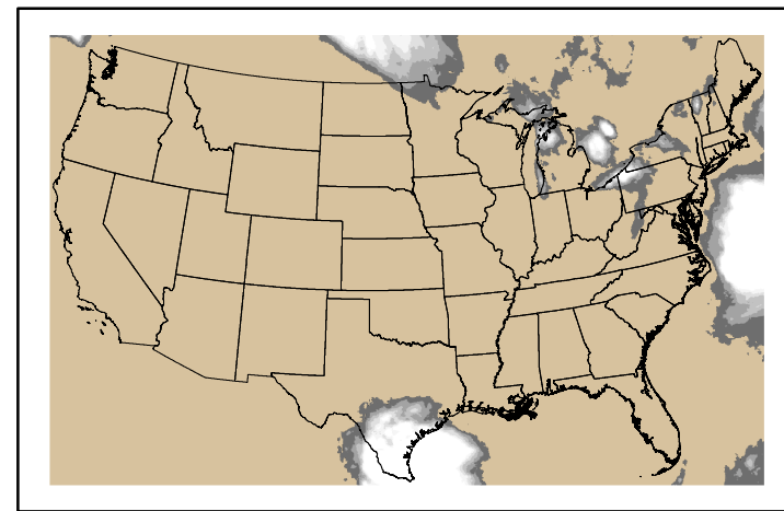
Precipitation p24m_2024113000f096.bil
