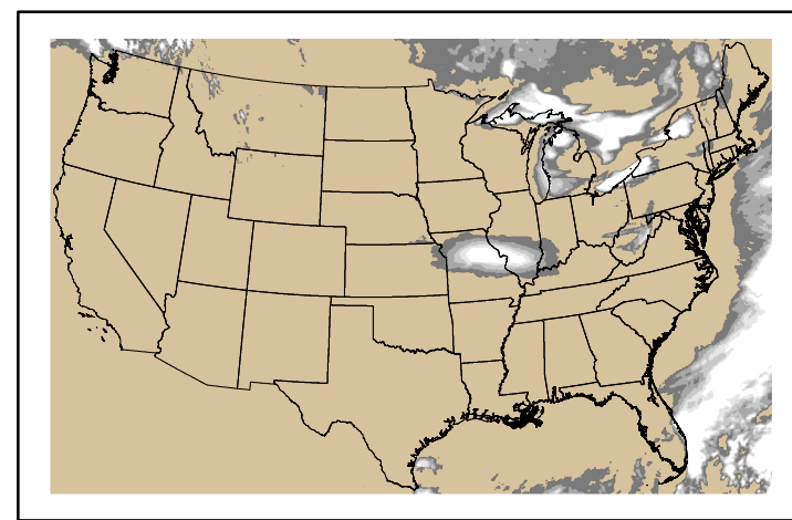
Precipitation p24m_2024113000f024.bil
