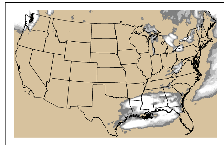
Precipitation p24m_2024113000f168.bil
