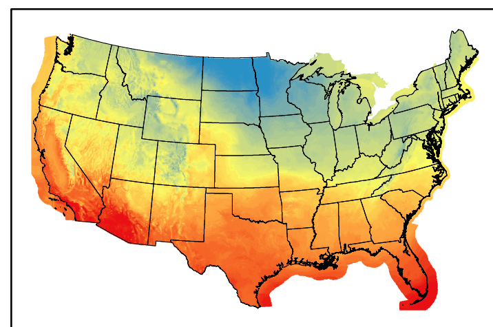
Dry Bulb Temp temp20241130.bil
