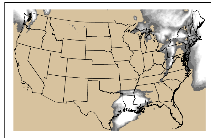
Precipitation p24m_2024113000f144.bil
