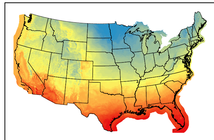
Dry Bulb Temp temp20241206.bil
