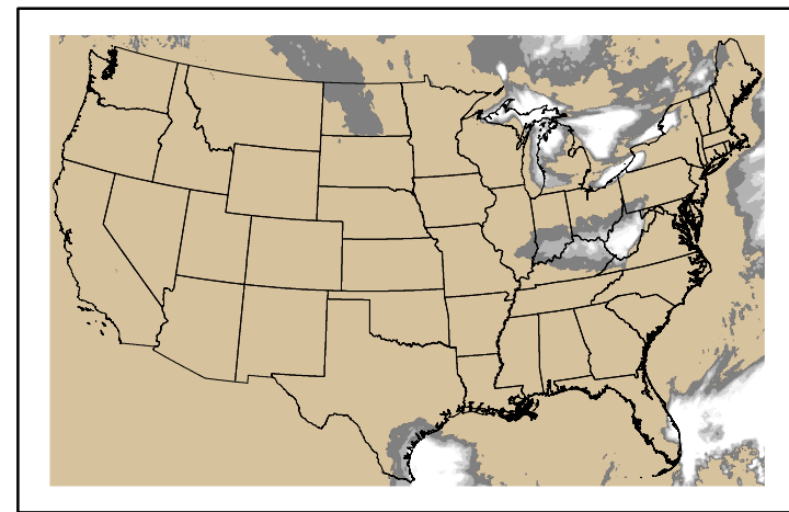
Precipitation p24m_2024113000f048.bil
