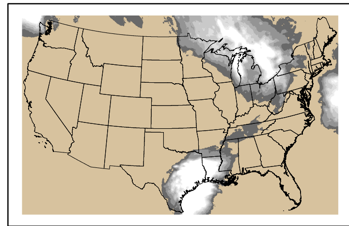
Precipitation p24m_2024113000f120.bil
