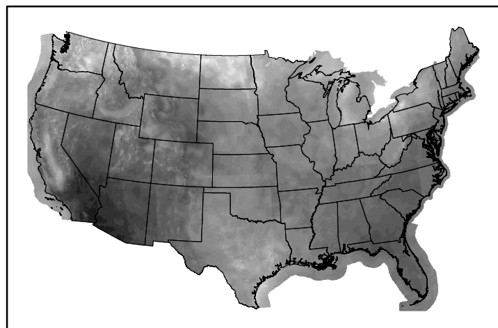
10hr Fuel Moisture mc10241203.bil
