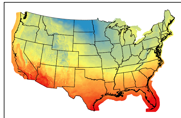
Dry Bulb Temp temp20241201.bil
