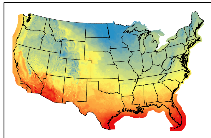
Dry Bulb Temp temp20241203.bil
