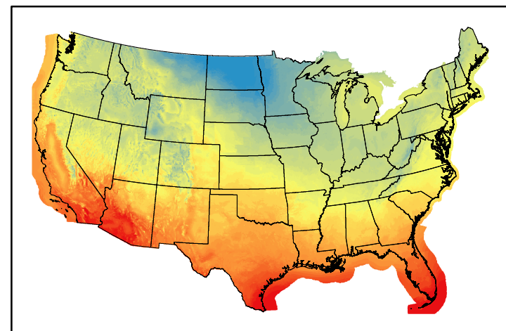
Dry Bulb Temp temp20241202.bil
