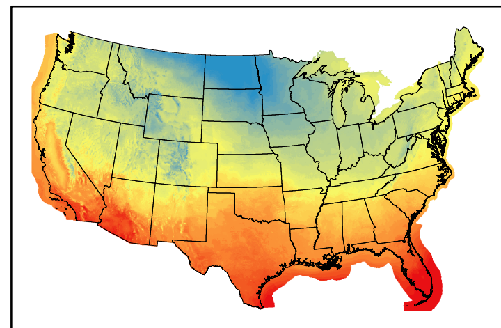
Dry Bulb Temp temp20241130.bil
