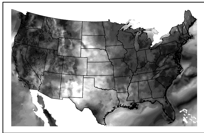
Wind Speed wspd20241127.bil
