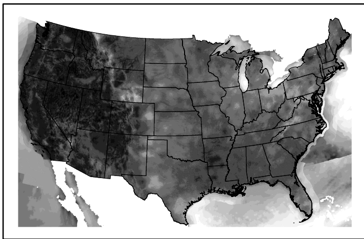
Wind Speed wspd20241202.bil
