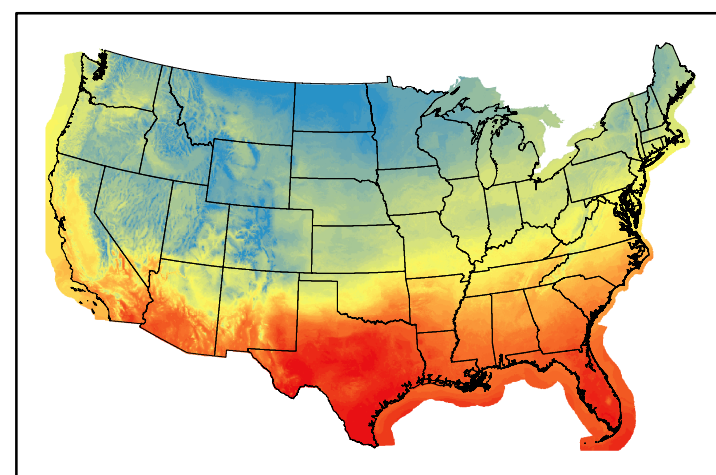
Dry Bulb Temp temp20241127.bil
