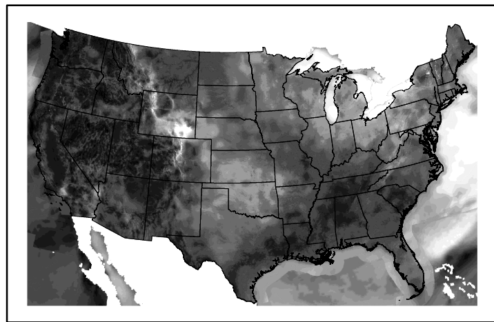
Wind Speed wspd20241130.bil
