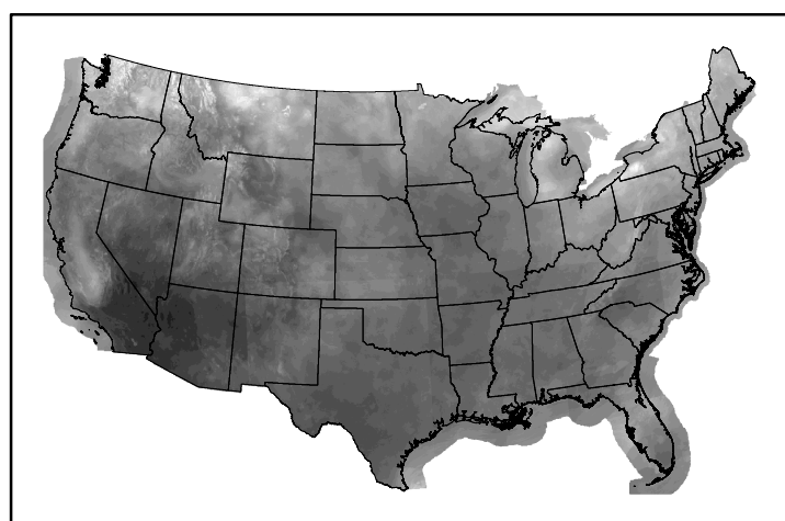
10hr Fuel Moisture mc10241129.bil
