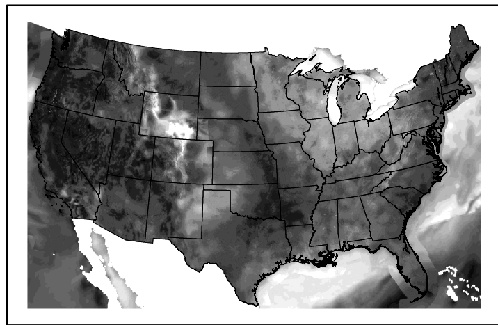
Wind Speed wspd20241129.bil
