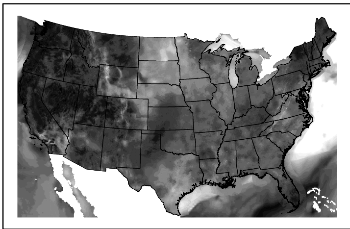
Wind Speed wspd20241128.bil
