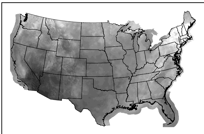
10hr Fuel Moisture mc10241128.bil
