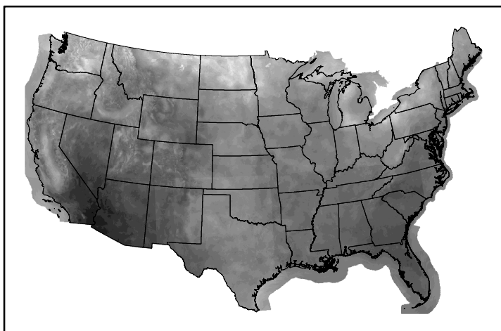
10hr Fuel Moisture mc10241202.bil
