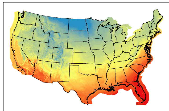
Dry Bulb Temp temp20241128.bil
