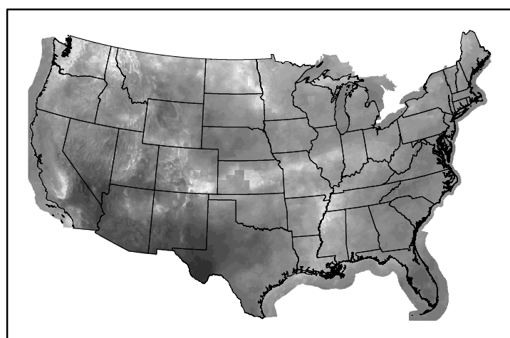
10hr Fuel Moisture mc10241127.bil
