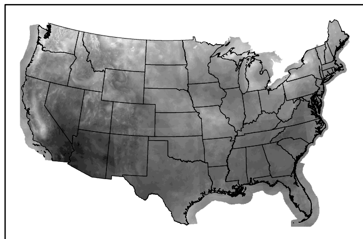
10hr Fuel Moisture mc10241130.bil
