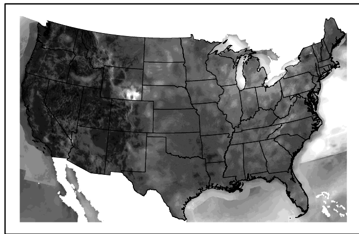
Wind Speed wspd20241201.bil
