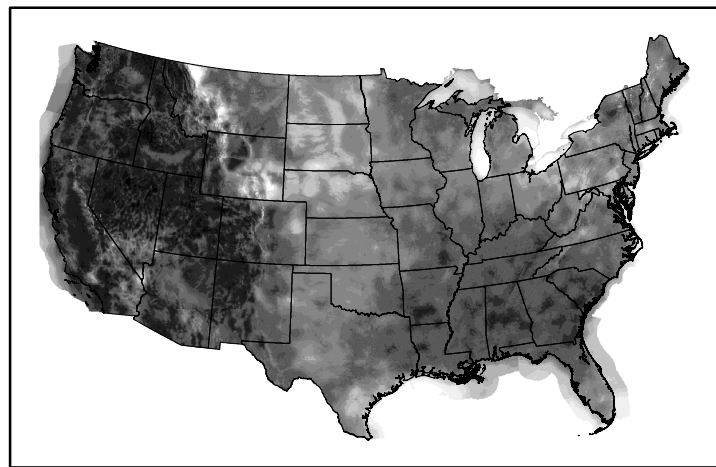
Wind Speed wspd20241203.bil
