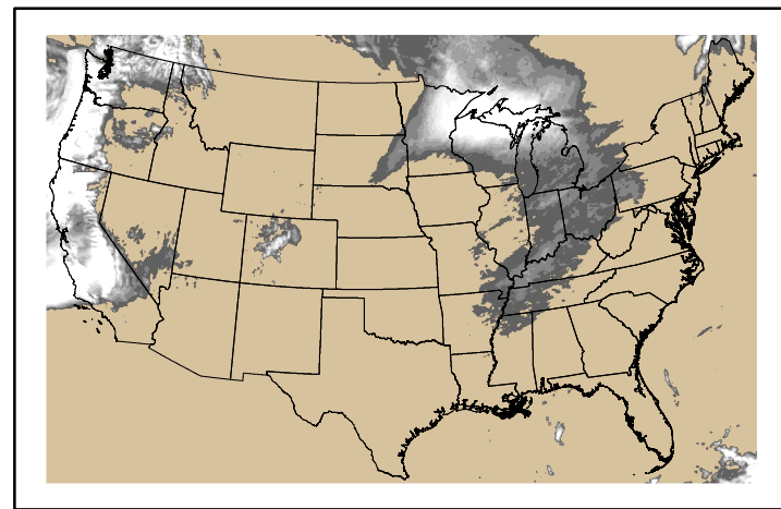
Precipitation p24m_2024112500f024.bil
