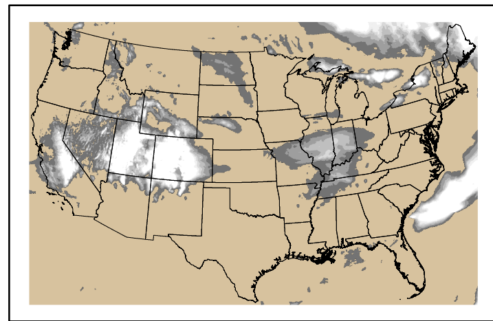
Precipitation p24m_2024112500f072.bil
