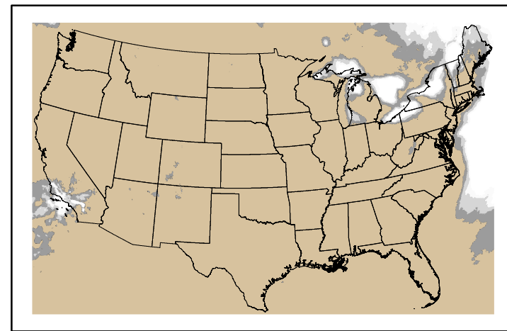
Precipitation p24m_2024112500f144.bil
