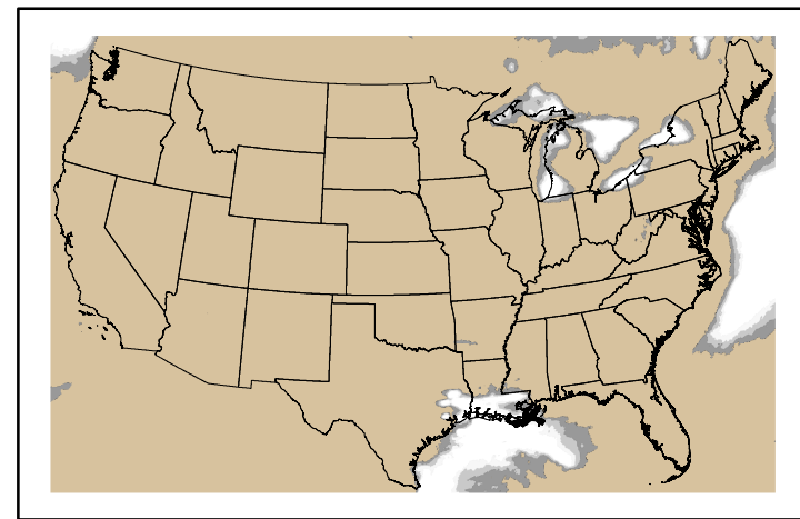
Precipitation p24m_2024112500f168.bil
