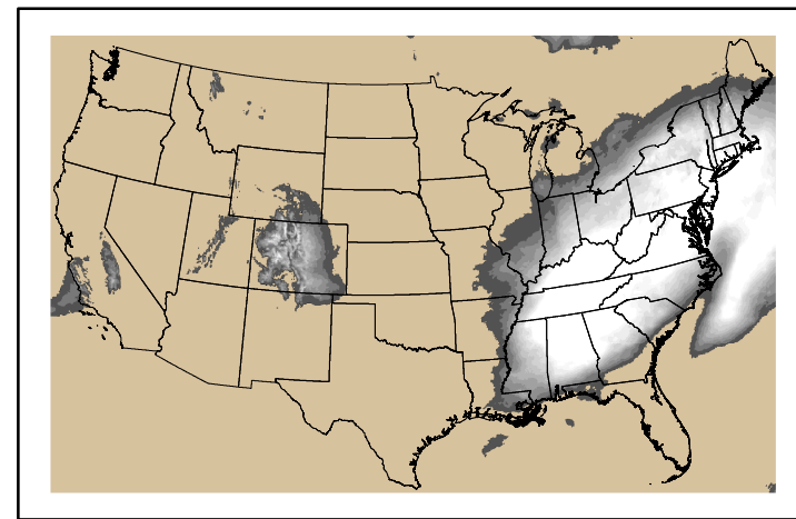
Precipitation p24m_2024112500f096.bil
