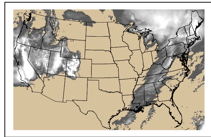
Precipitation p24m_2024112500f048.bil
