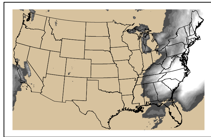
Precipitation p24m_2024112500f120.bil
