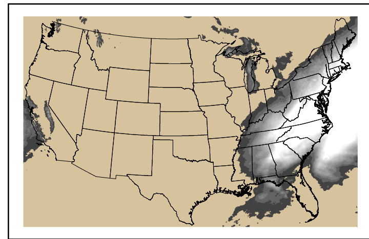
Precipitation p24m_2024112400f144.bil
