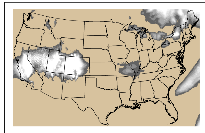
Precipitation p24m_2024112400f096.bil
