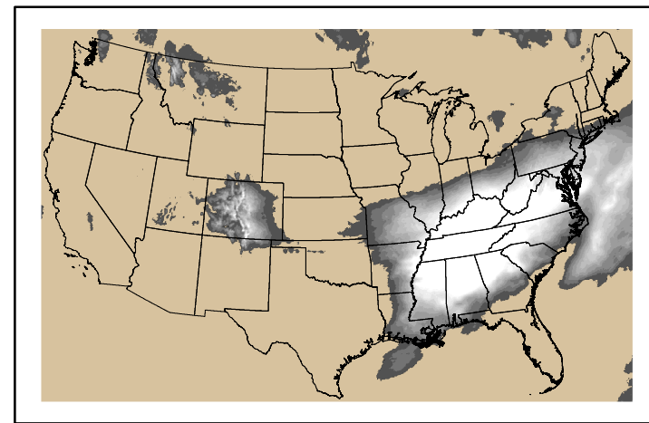
Precipitation p24m_2024112400f120.bil
