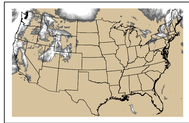
Precipitation p24m_2024112400f024.bil
