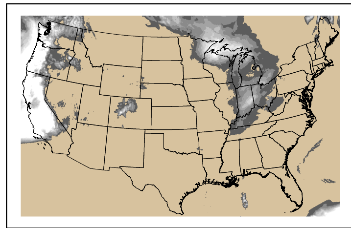
Precipitation p24m_2024112400f048.bil
