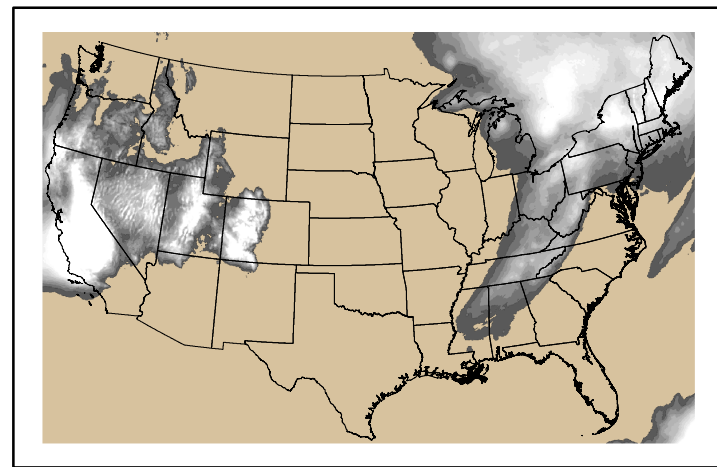
Precipitation p24m_2024112400f072.bil
