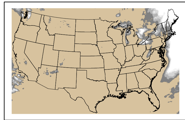
Precipitation p24m_2024112400f168.bil
