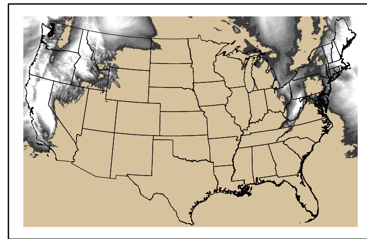
Precipitation p24m_2024112300f024.bil
