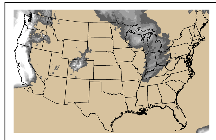
Precipitation p24m_2024112300f072.bil
