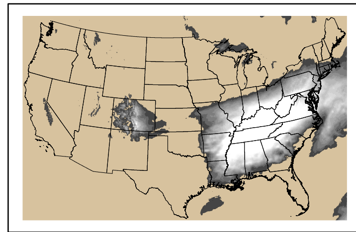
Precipitation p24m_2024112300f144.bil
