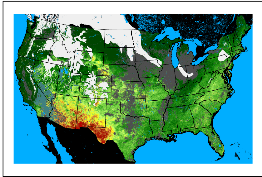
WFPI fp241125.bil
