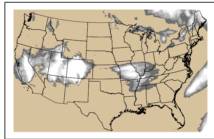
Precipitation p24m_2024112300f120.bil
