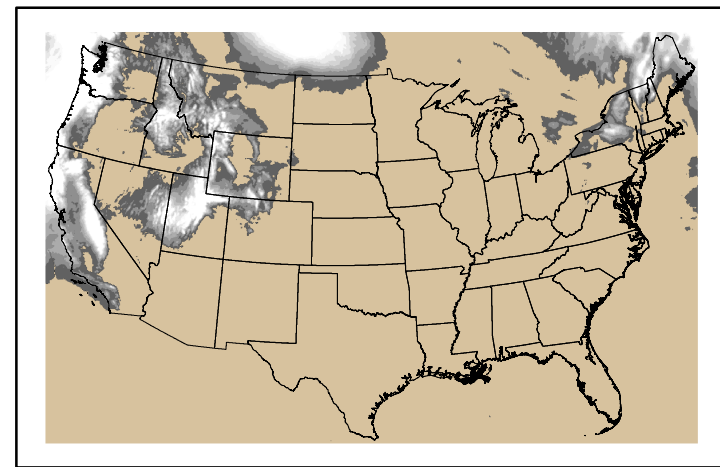
Precipitation p24m_2024112300f048.bil
