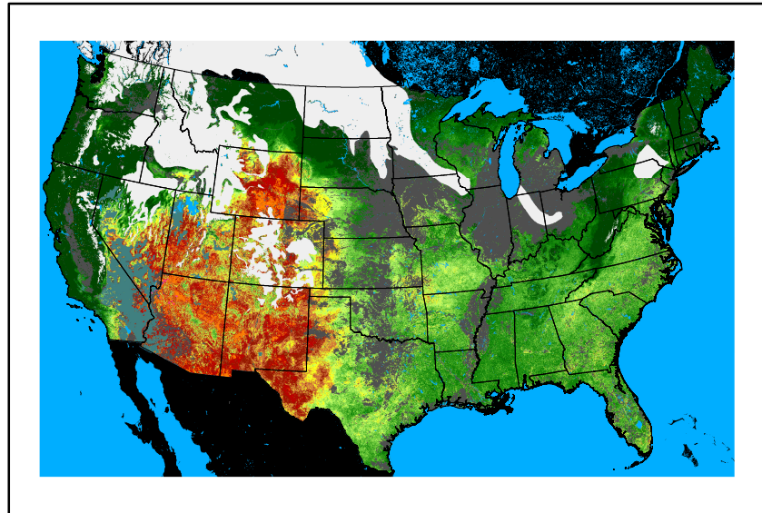
WFPI fp241123.bil
