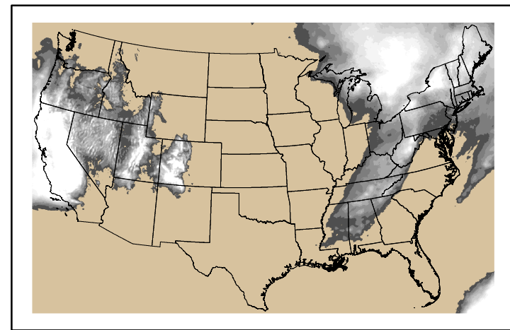
Precipitation p24m_2024112300f096.bil
