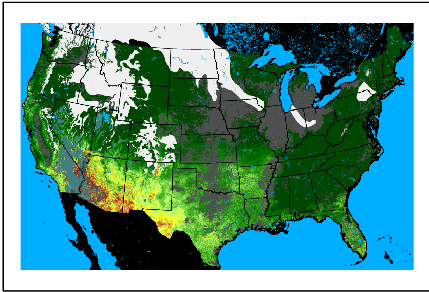
WFPI fp241129.bil
