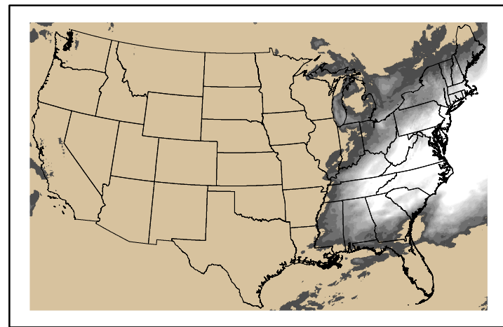
Precipitation p24m_2024112300f168.bil
