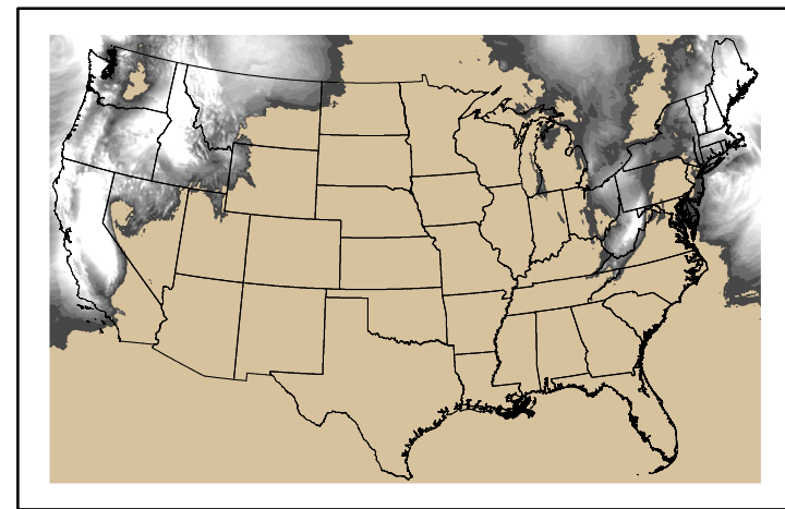
Precipitation p24m_2024112200f048.bil
