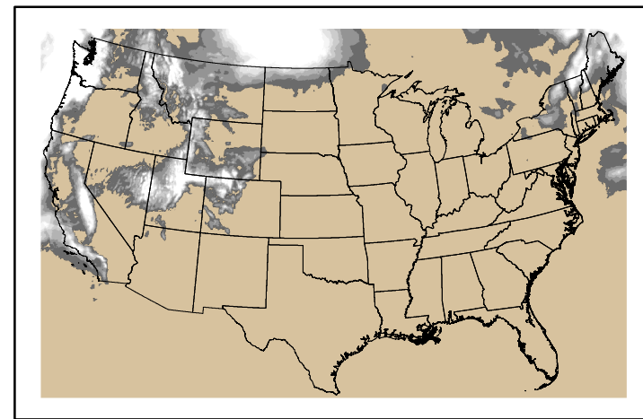
Precipitation p24m_2024112200f072.bil
