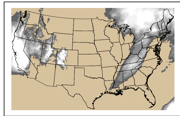
Precipitation p24m_2024112200f120.bil
