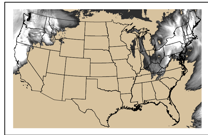
Precipitation p24m_2024112200f024.bil
