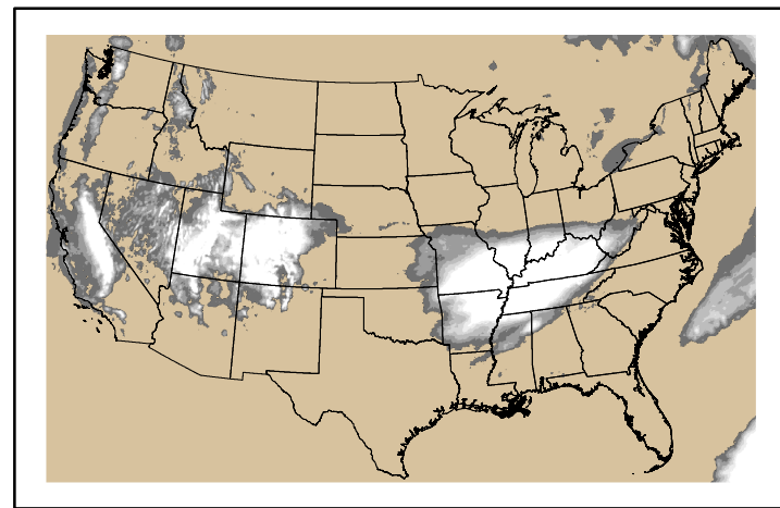
Precipitation p24m_2024112200f144.bil
