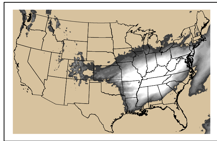
Precipitation p24m_2024112200f168.bil
