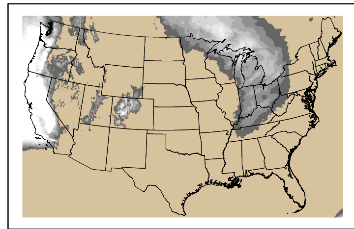
Precipitation p24m_2024112200f096.bil
