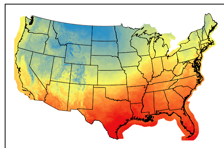
Dry Bulb Temp temp20241125.bil
