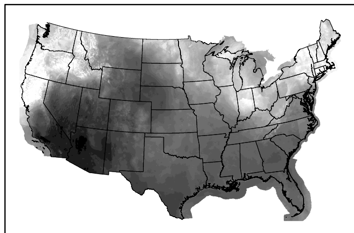
10hr Fuel Moisture mc10241121.bil
