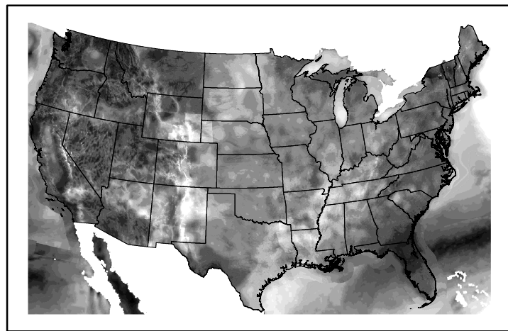
Wind Speed wspd20241125.bil
