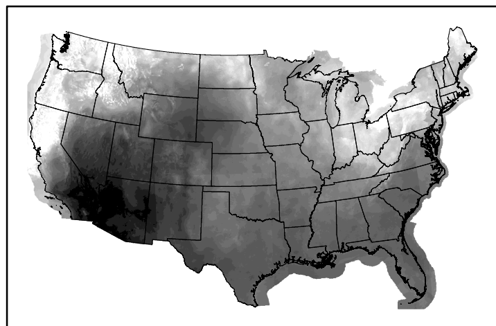
10hr Fuel Moisture mc10241122.bil
