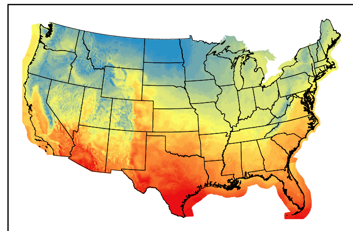
Dry Bulb Temp temp20241123.bil
