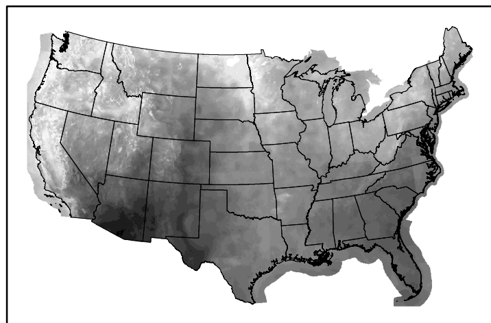
10hr Fuel Moisture mc10241124.bil
