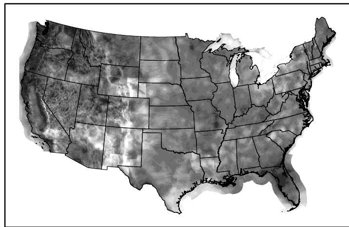
Wind Speed wspd20241126.bil
