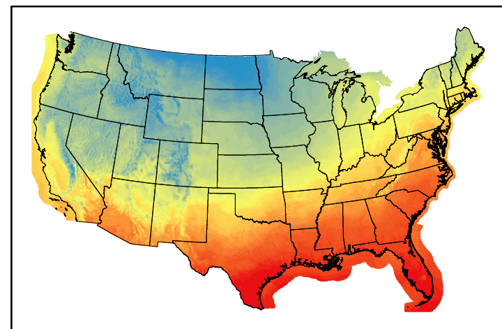
Dry Bulb Temp temp20241126.bil
