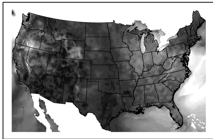
Wind Speed wspd20241122.bil
