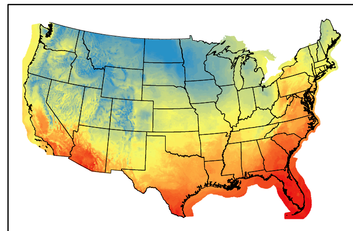
Dry Bulb Temp temp20241120.bil
