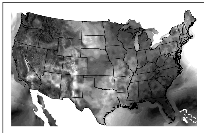
Wind Speed wspd20241124.bil
