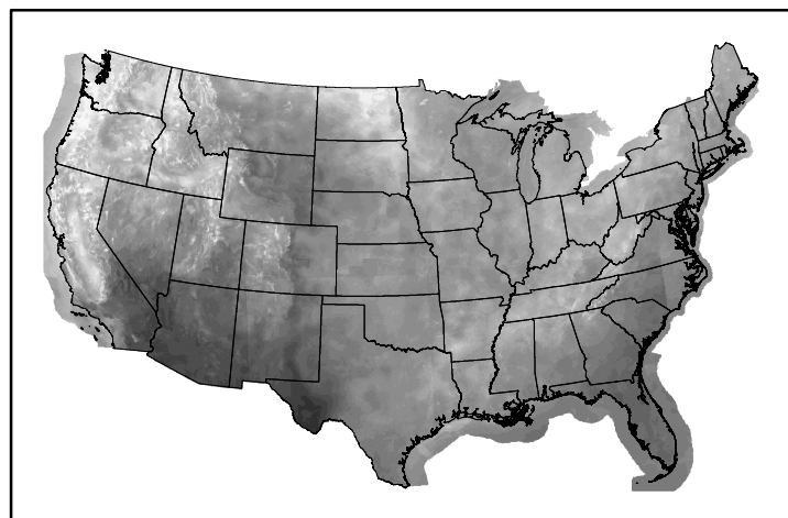
10hr Fuel Moisture mc10241126.bil
