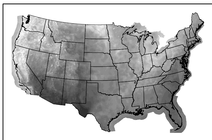
10hr Fuel Moisture mc10241125.bil
