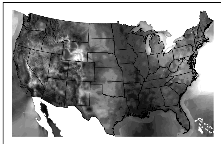
Wind Speed wspd20241123.bil
