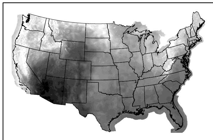
10hr Fuel Moisture mc10241123.bil
