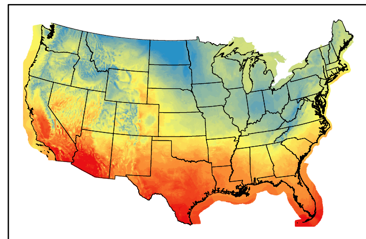
Dry Bulb Temp temp20241121.bil
