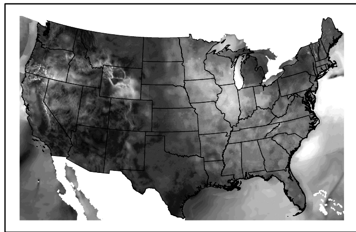
Wind Speed wspd20241121.bil
