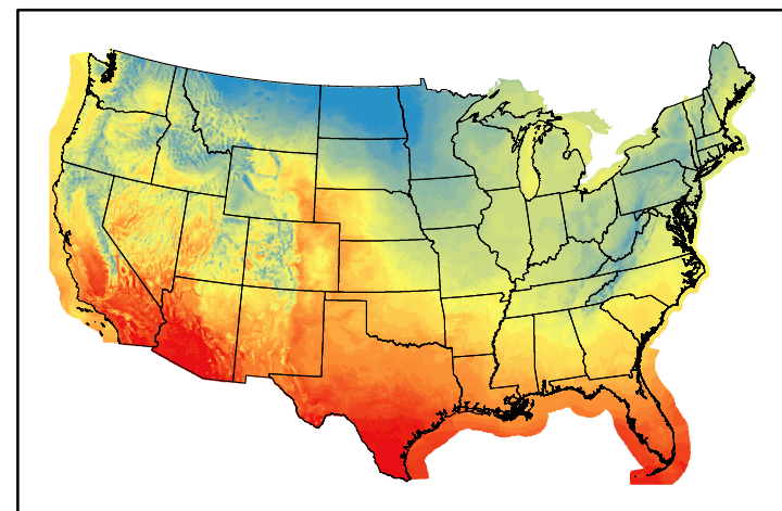
Dry Bulb Temp temp20241122.bil
