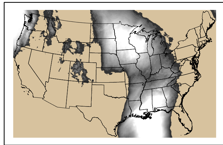
Precipitation p24m_2024111600f096.bil
