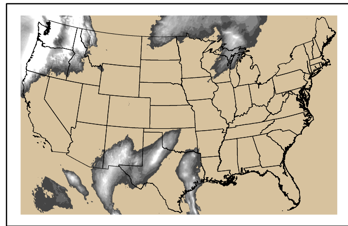
Precipitation p24m_2024111600f048.bil
