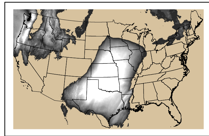
Precipitation p24m_202411600f072.bil
