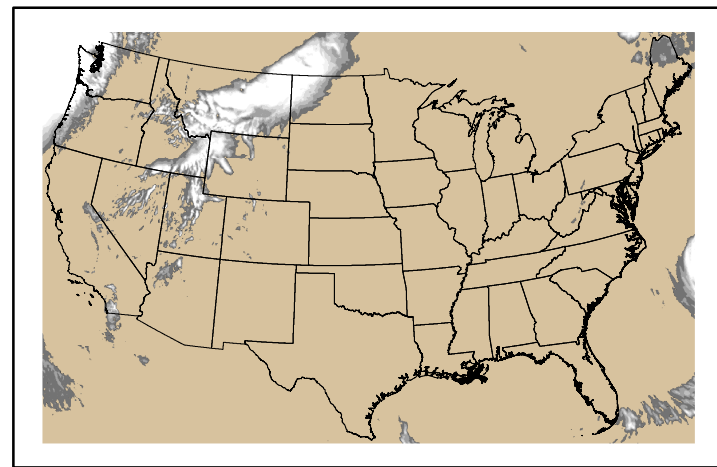
Precipitation p24m_2024111600f024.bil
