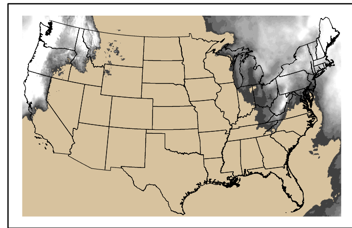
Precipitation p24m_202411600f168.bil
