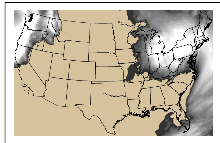
Precipitation p24m_202411600f144.bil
