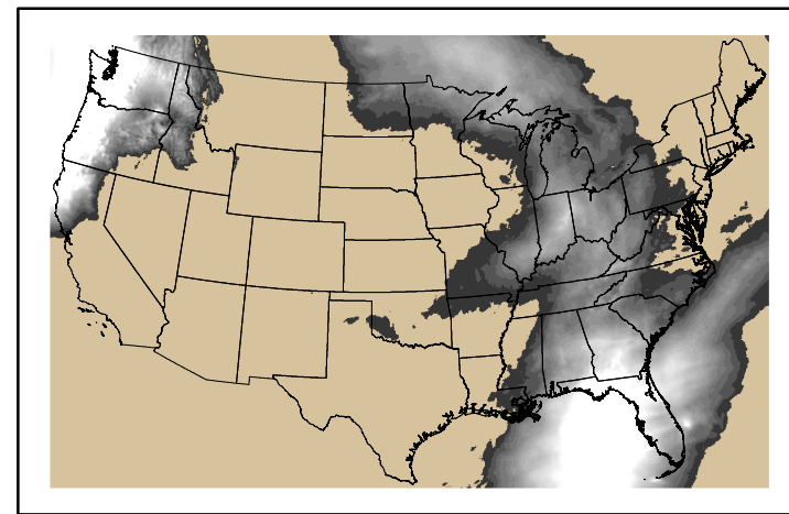
Precipitation p24m_202411600f120.bil
