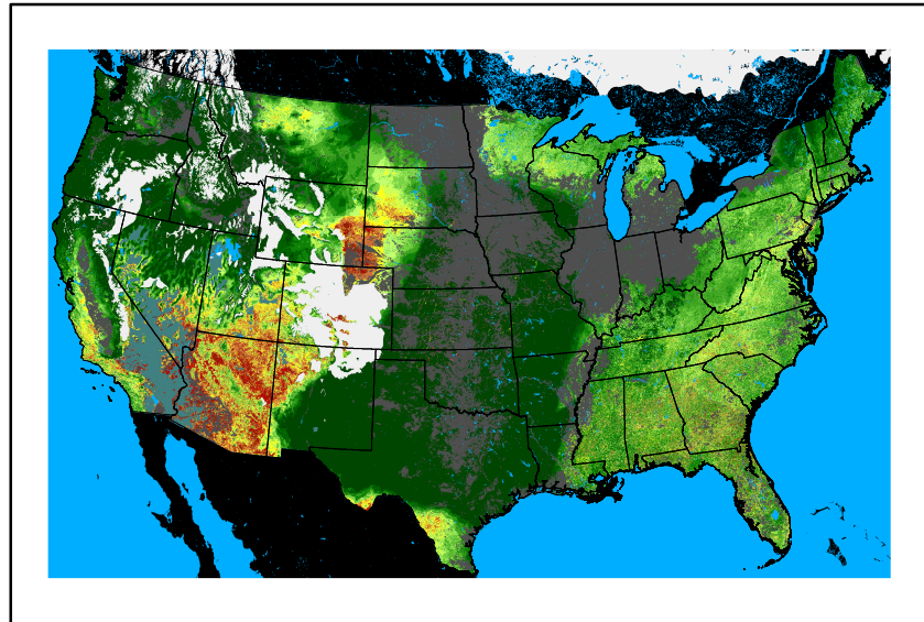
WFPI fp241118.bil
