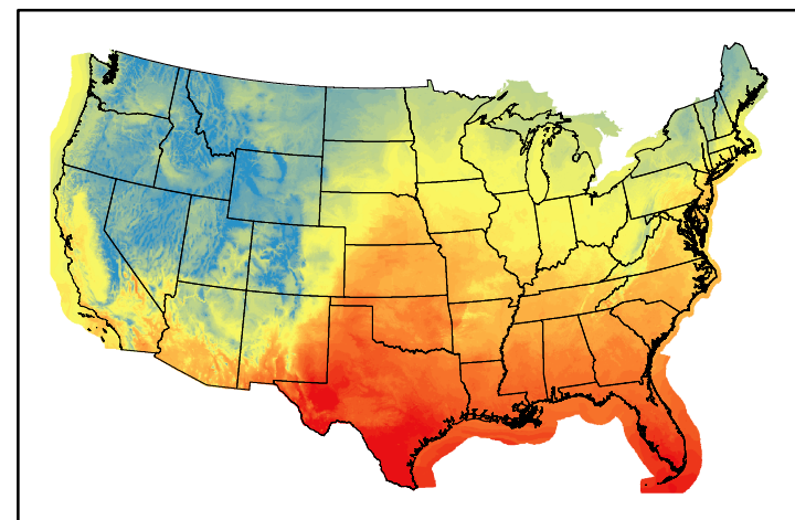
Dry Bulb Temp temp20241116.bil
