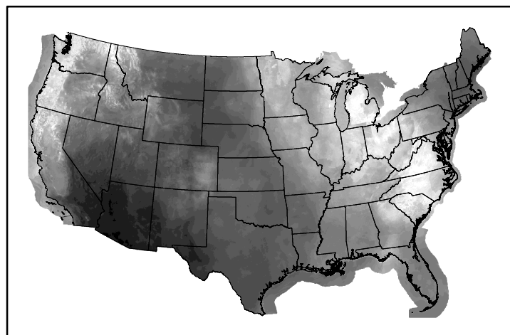
10hr Fuel Moisture mc10241114.bil
