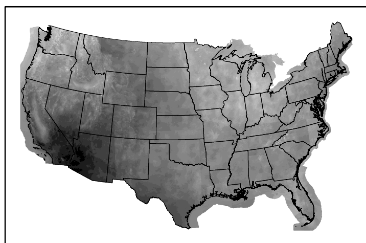
10hr Fuel Moisture mc10241120.bil
