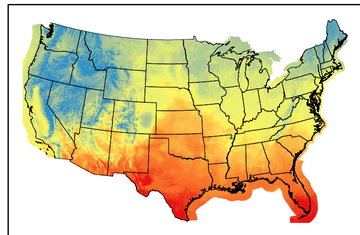
Dry Bulb Temp temp20241115.bil
