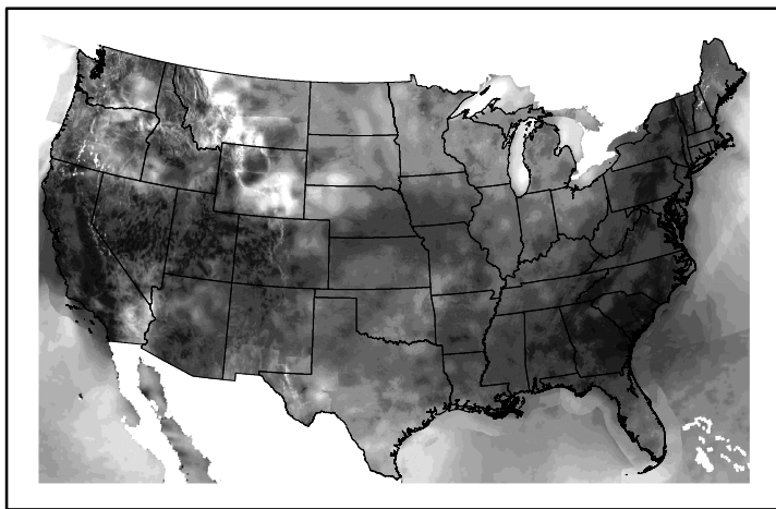
Wind Speed wspd20241117.bil
