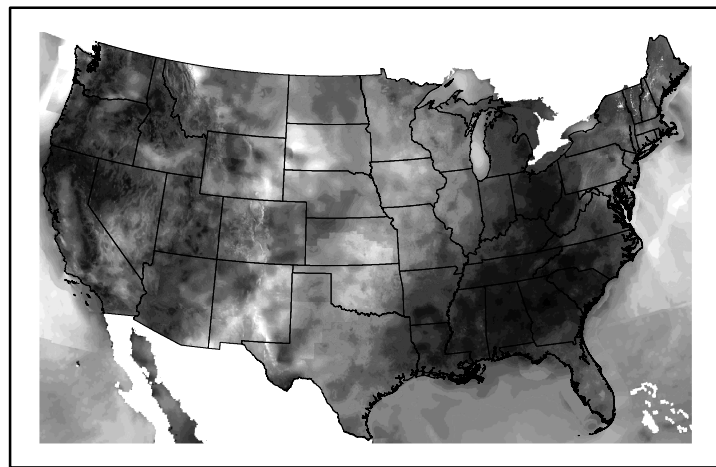
Wind Speed wspd20241116.bil
