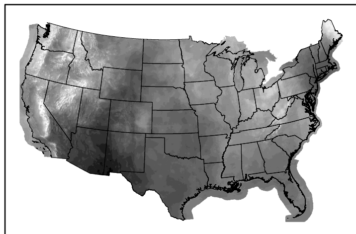
10hr Fuel Moisture mc10241115.bil
