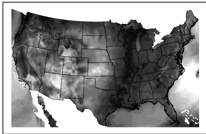
Wind Speed wspd20241115.bil
