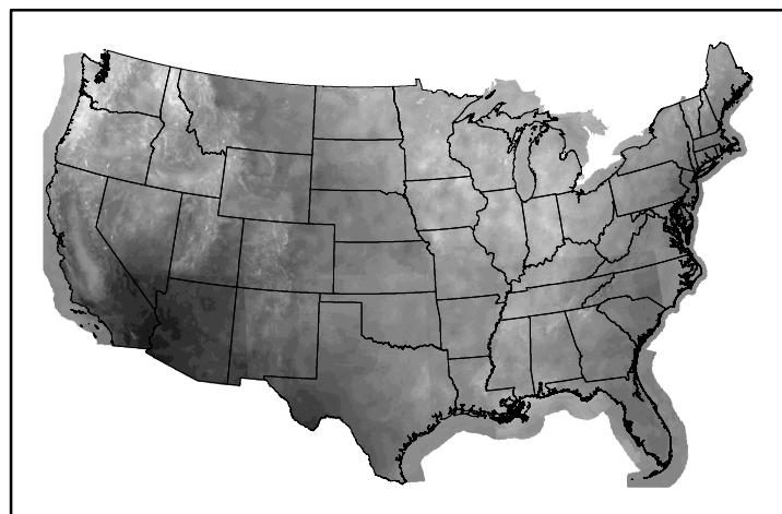
10hr Fuel Moisture mc10241119.bil
