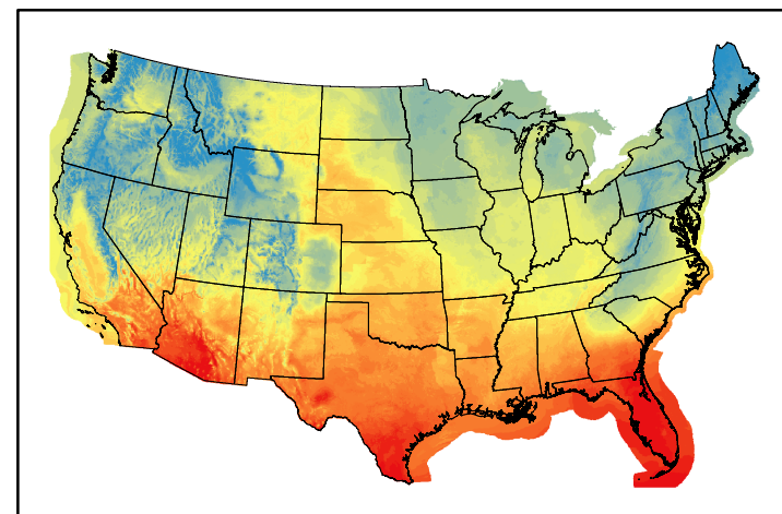
Dry Bulb Temp temp20241114.bil
