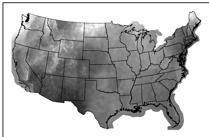
10hr Fuel Moisture mc10241116.bil
