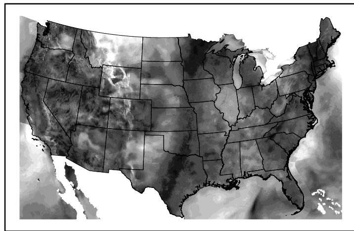
Wind Speed wspd20241114.bil
