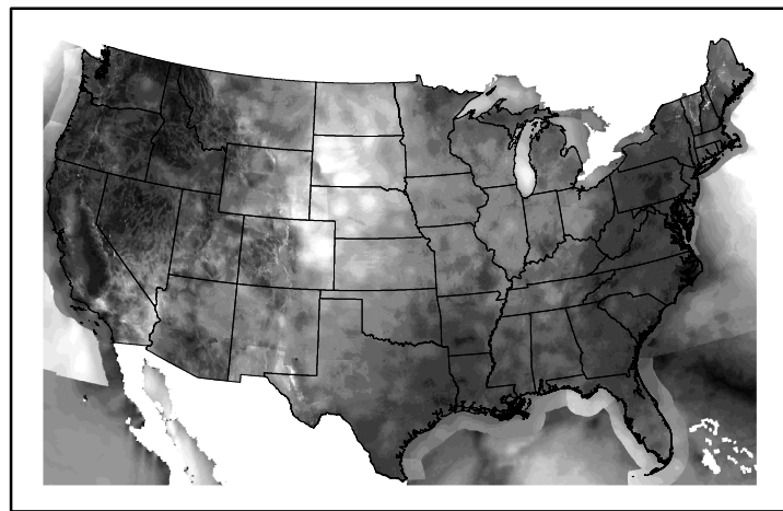
Wind Speed wspd20241119.bil
