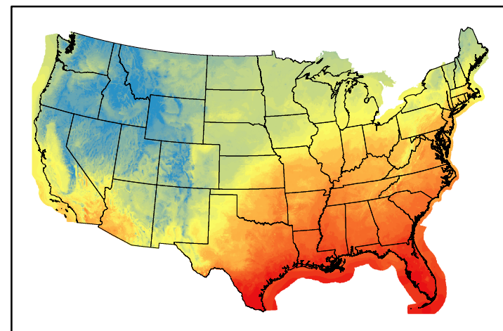
Dry Bulb Temp temp20241118.bil
