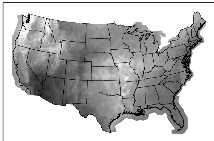
10hr Fuel Moisture mc10241118.bil
