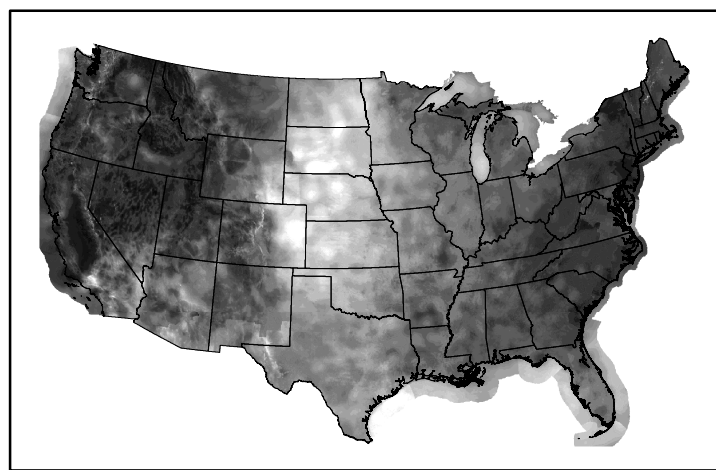
Wind Speed wspd20241120.bil
