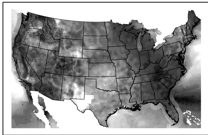
Wind Speed wspd20241118.bil
