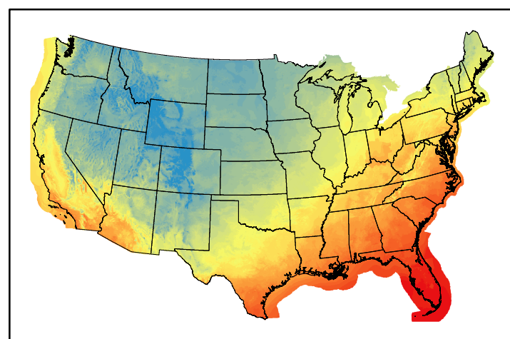
Dry Bulb Temp temp20241120.bil
