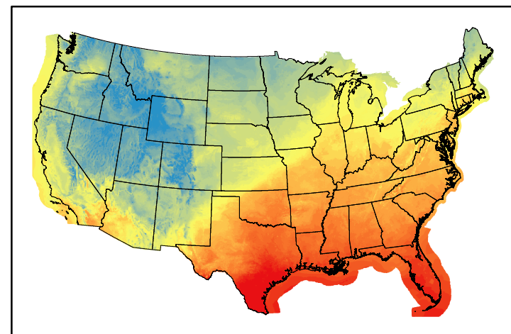
Dry Bulb Temp temp20241117.bil
