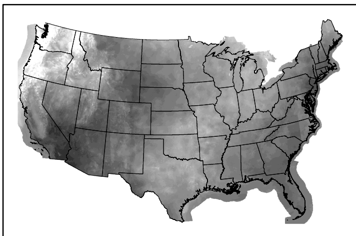
10hr Fuel Moisture mc10241117.bil
