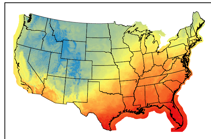
Dry Bulb Temp temp20241119.bil
