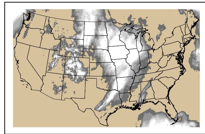
Precipitation p24m_202411300f168.bil
