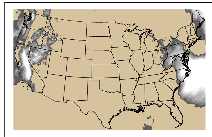
Precipitation p24m_2024111300f072.bil
