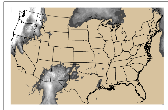
Precipitation p24m_2024111300f120.bil
