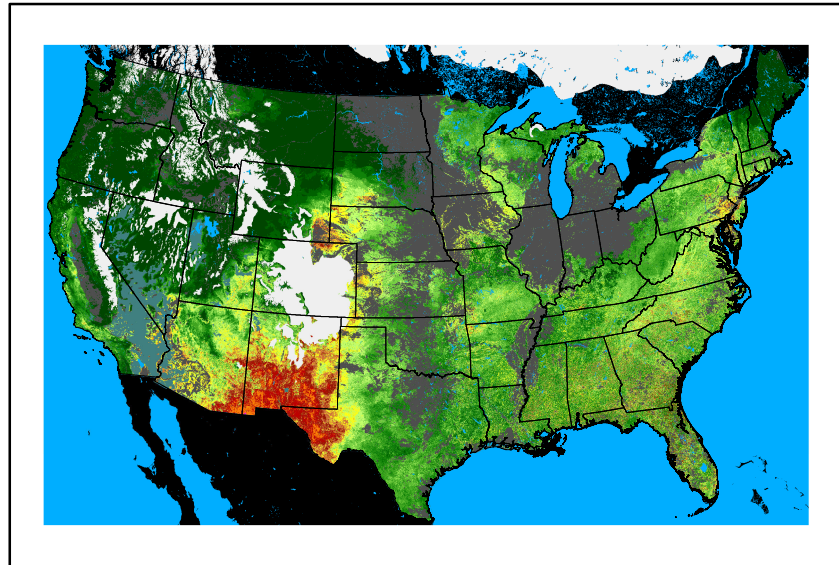
WFPI fp241116.bil
