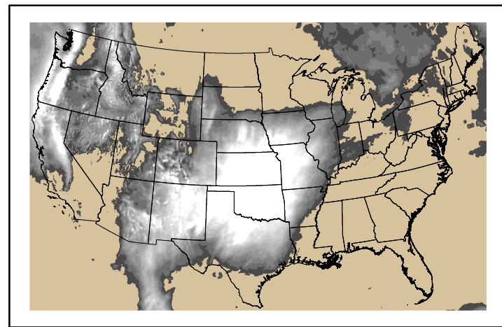
Precipitation p24m_202411300f144.bil
