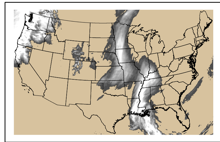
Precipitation p24m_2024111300f024.bil
