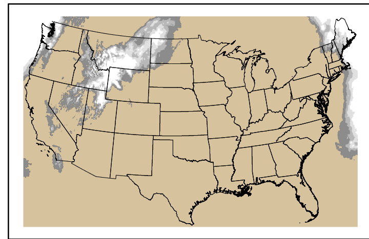
Precipitation p24m_2024111300f096.bil
