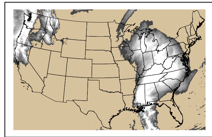
Precipitation p24m_2024111300f048.bil
